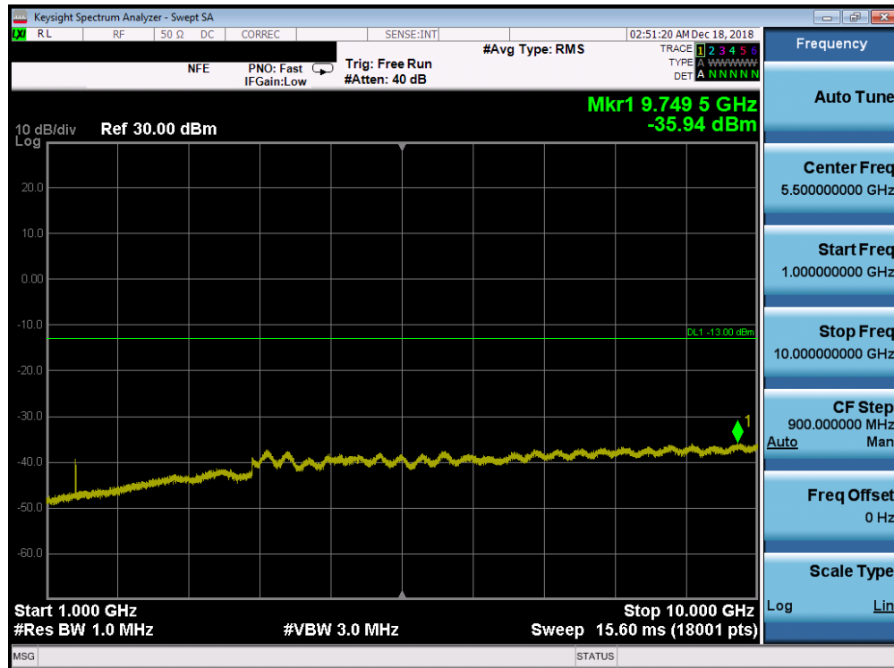
Plot 7-120. Conducted Spurious Plot (Band 71 - 15.0MHz QPSK - RB Size 1, RB Offset 0 - High Channel)
