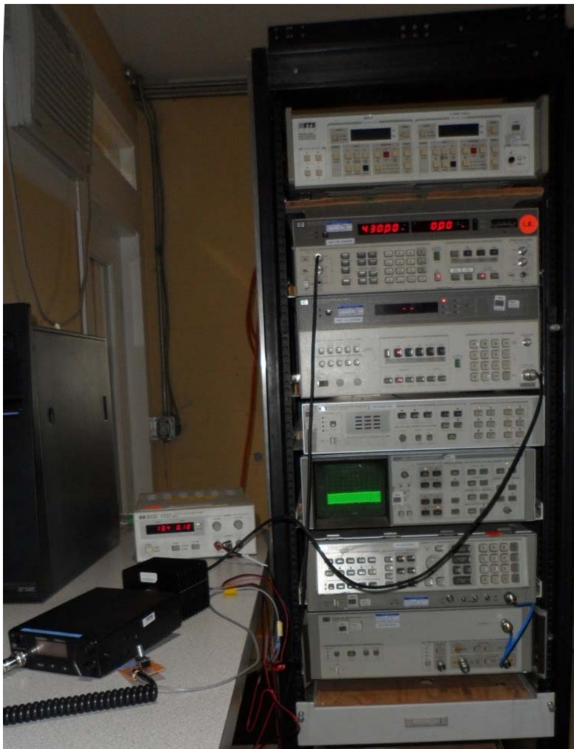
Figure E21.2 – Setup Photo – Audio Response Measurements
