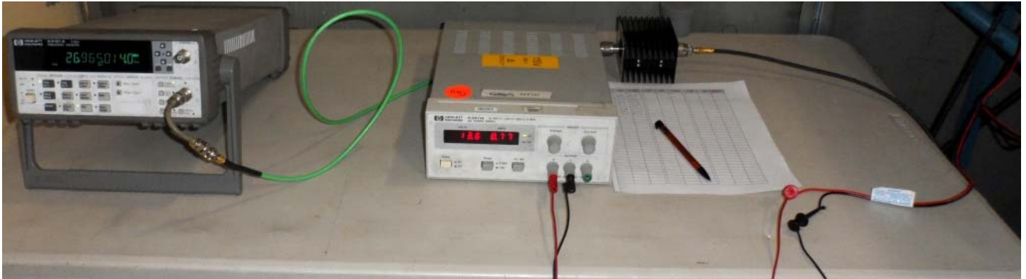
Figure E21.3 – Setup Photo – Frequency Stability Measurements
