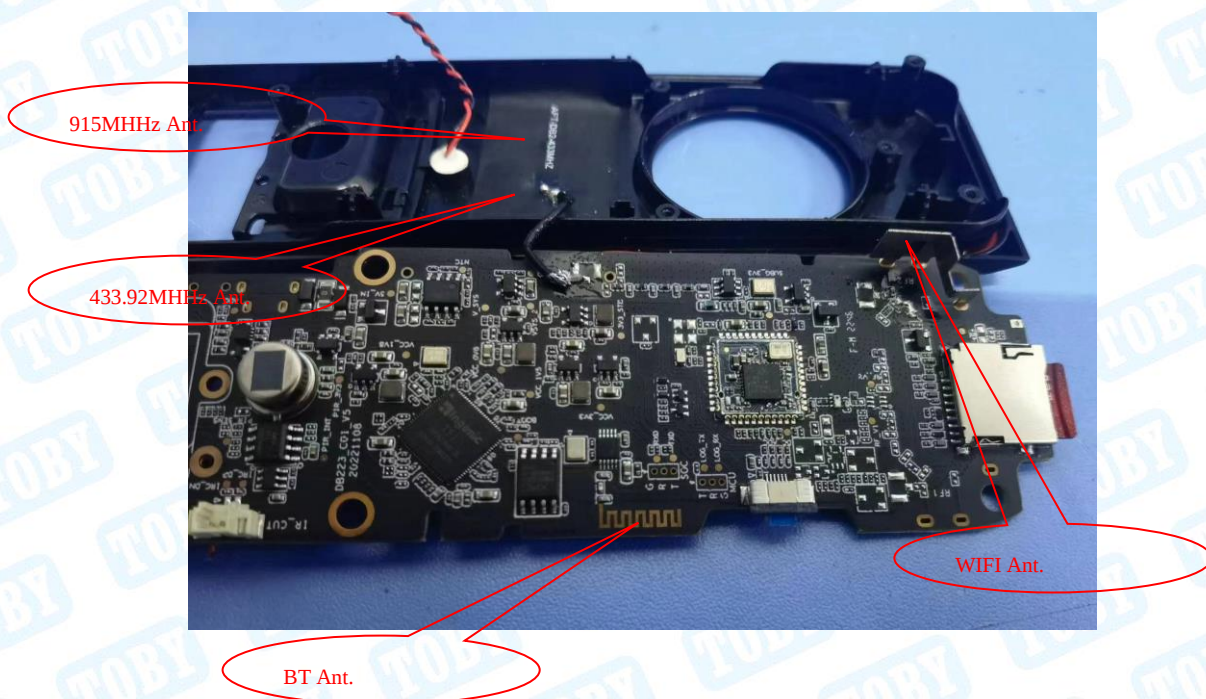
Photo 12 Appearance of PCB
