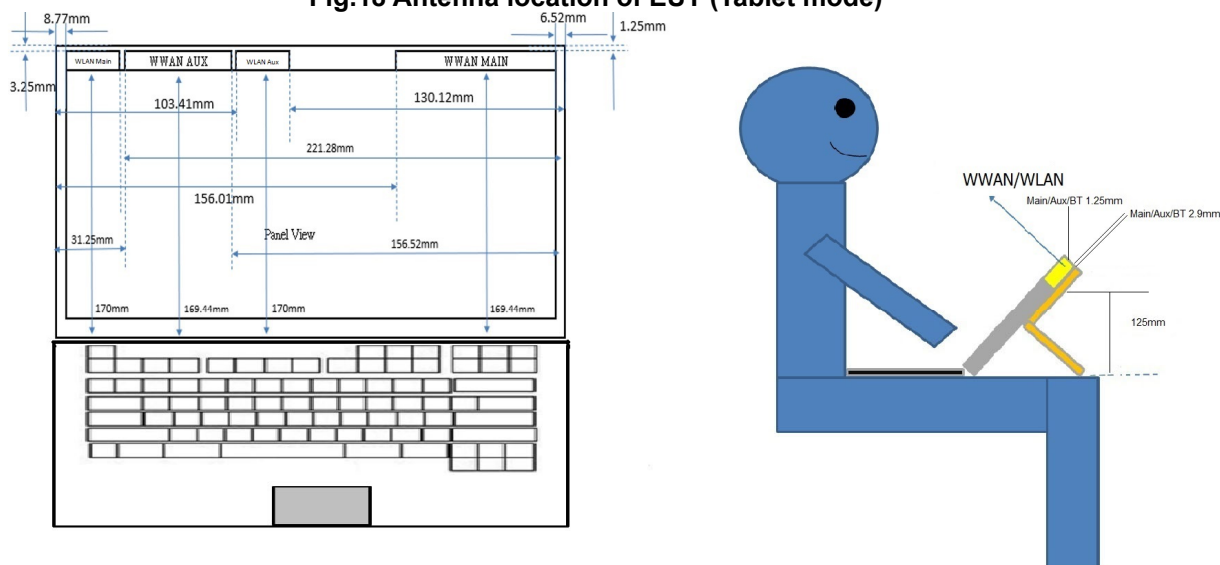
Fig.18 Antenna location of EUT (Tablet mode)
