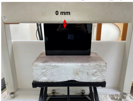
Fig.13 With_Kickstand_Top side
