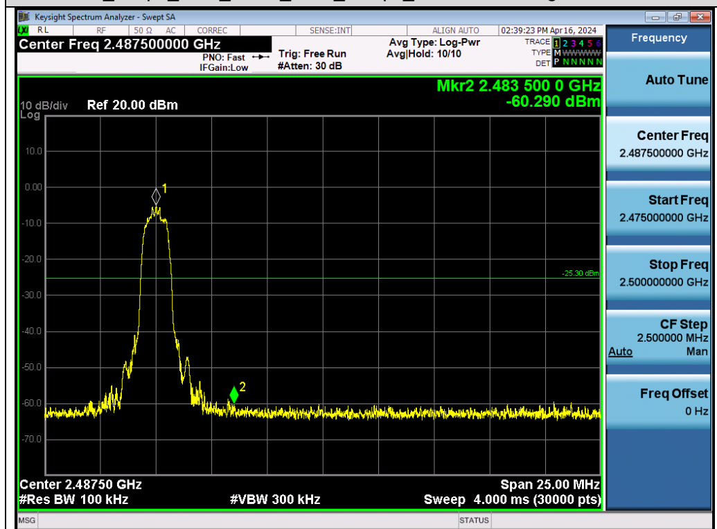
Test Graph EDR ANT1 2480 3Mbps Higher Band Edge Emissions
