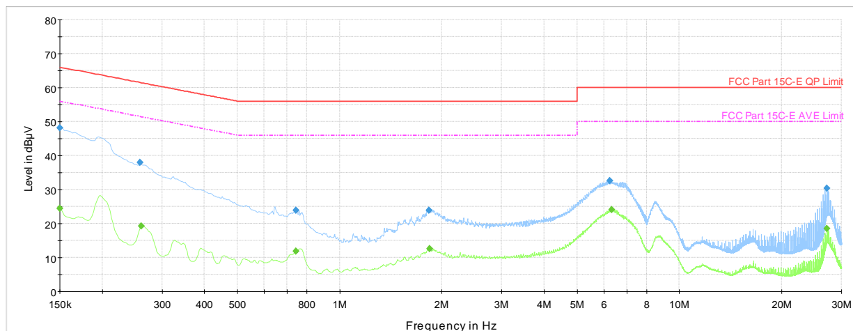
Plot 7-36. AC Line Conducted Plot with Bluetooth LE (N, 1Mbps – Ch.39 with host PC and USB-C Cable)
