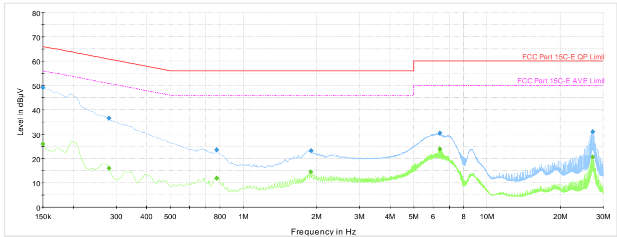
Plot 7-35. AC Line Conducted Plot with Bluetooth LE (L1, 1Mbps – Ch.39 with host PC and USB-C Cable)
