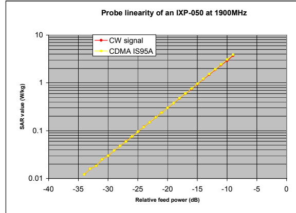
Figure 12. The CDMA IS95A response of an IXP-050 probe at 1900MHz.
