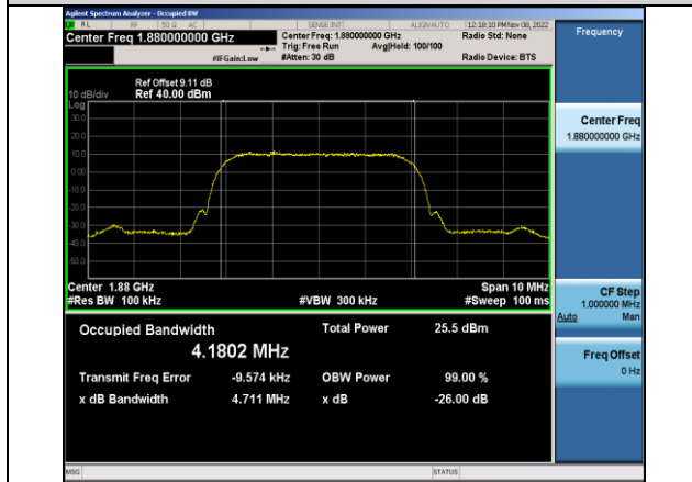
Band2-9400-4.711
