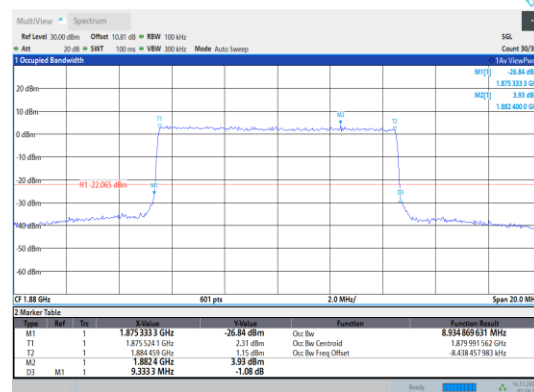
Band2-10MHz-64QAM-18900-50RB#0
