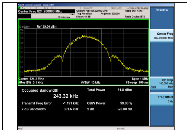
EGPRS850-128-8-0.3016
