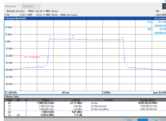
Band2-10MHz-64QAM-19150-50RB#0
