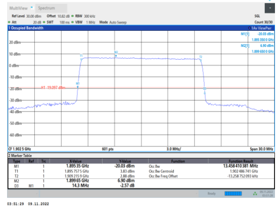
Band2-15MHz-16QAM-19125-75RB#0
