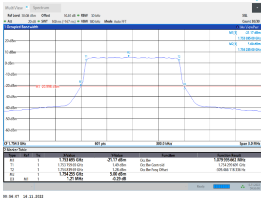
Band4-1.4MHz-64QAM-20393-6RB#0
