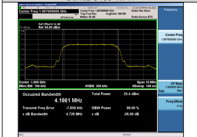
Band2-9538-4.726
