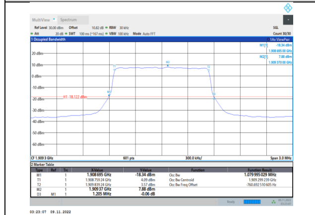
Band2-1.4MHz-QPSK-19193-6RB#0
