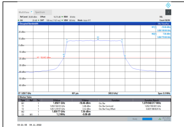
Band2-1.4MHz-QPSK-18607-6RB#0
