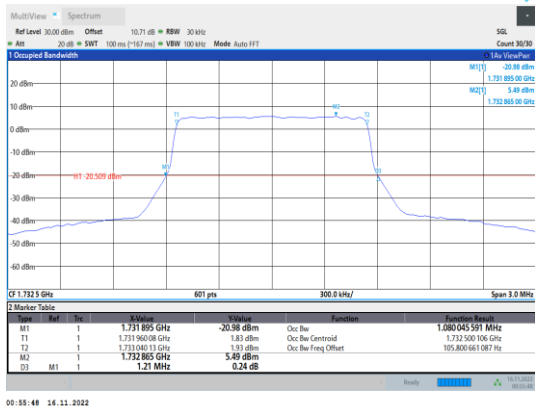
Band4-1.4MHz-64QAM-20175-6RB#0
