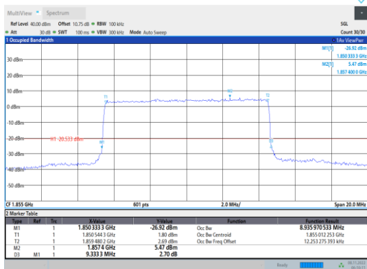
Band2-10MHz-16QAM-18650-50RB#0
