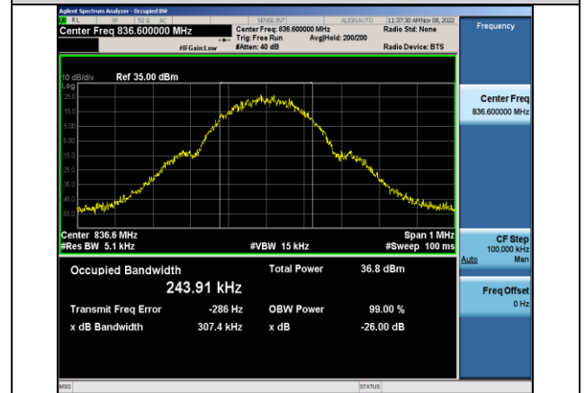
GPRS850-190-3-0.3074
