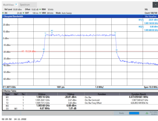
Band2-5MHz-64QAM-19175-25RB#0
