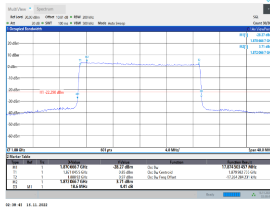
Band2-20MHz-64QAM-18900-100RB#0
