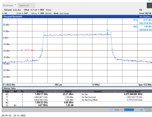
Band2-5MHz-64QAM-18625-25RB#0
