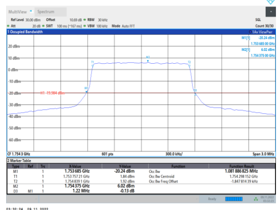
Band4-1.4MHz-16QAM-20393-6RB#0
