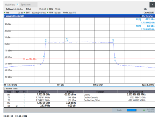
Band4-3MHz-QPSK-20385-15RB#0
