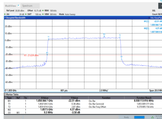
Band2-10MHz-64QAM-18650-50RB#0
