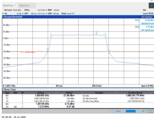
03:04:52 16.11.2022 Band2-1.4MHz-64QAM-18607-6RB#0
