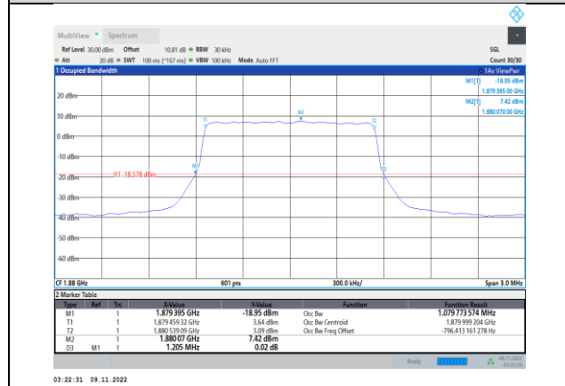
Band2-1.4MHz-QPSK-18900-6RB#0
