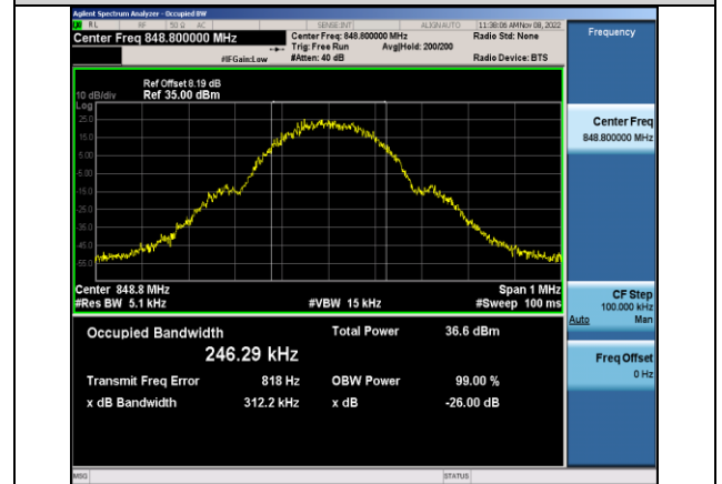
GPRS850-251-3-0.3122
