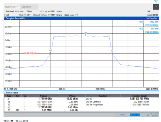
Band4-1.4MHz-16QAM-20175-6RB#0
