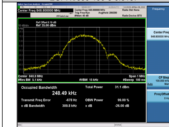
EGPRS850-251-8-0.3098
