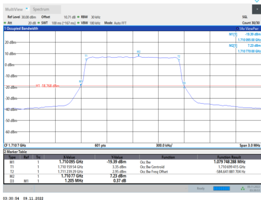
Band4-1.4MHz-QPSK-19957-6RB#0
