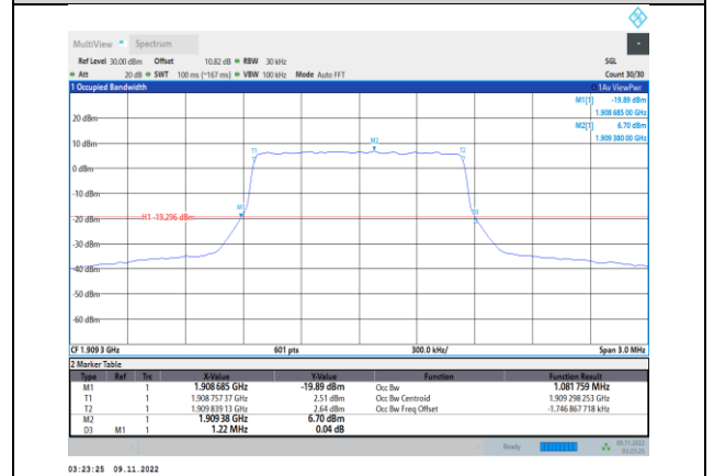
Band2-1.4MHz-16QAM-19193-6RB#0
