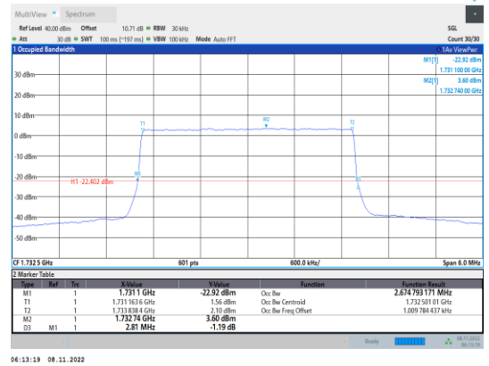
Band4-3MHz-QPSK-20175-15RB#0
