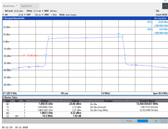
Band2-15MHz-64QAM-18675-75RB#0
