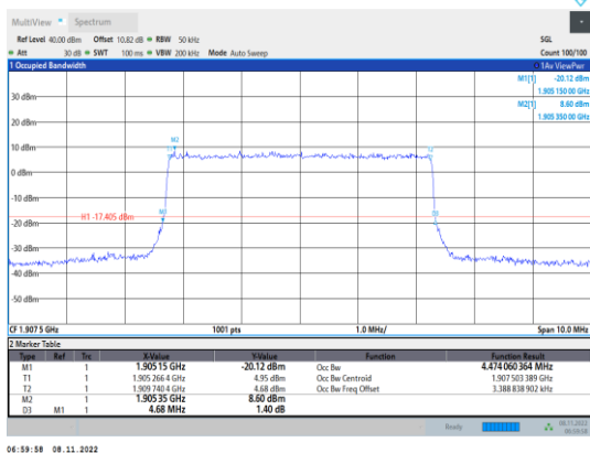
Band2-5MHz-QPSK-19175-25RB#0
