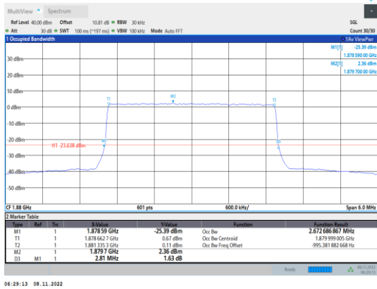
Band2-3MHz-16QAM-18900-15RB#0
