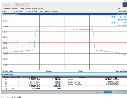
Band2-15MHz-64QAM-19125-75RB#0
