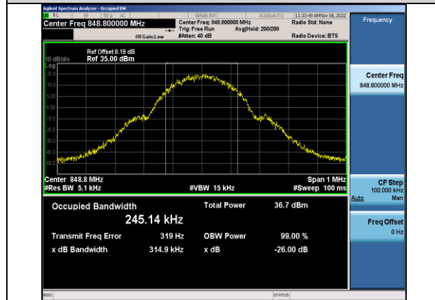
GSM850-251-3-0.3149
