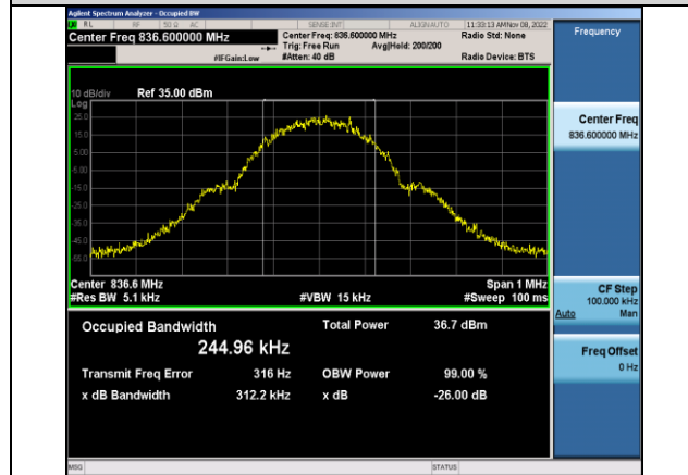
GSM850-190-3-0.3122
