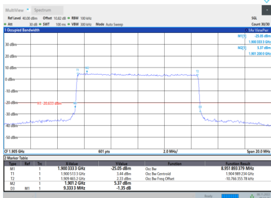
Band2-10MHz-16QAM-19150-50RB#0
