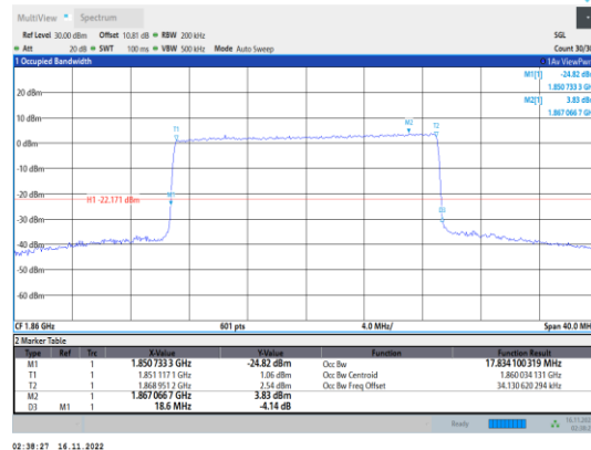
Band2-20MHz-64QAM-18700-100RB#0
