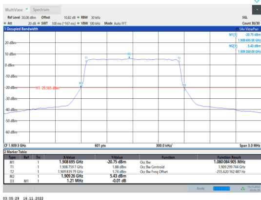
03:05:29 16.11.2022 Band2-1.4MHz-64QAM-19193-6RB#0
