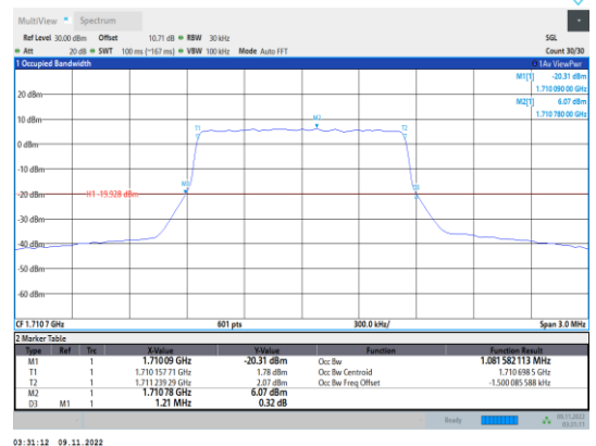
Band4-1.4MHz-16QAM-19957-6RB#0
