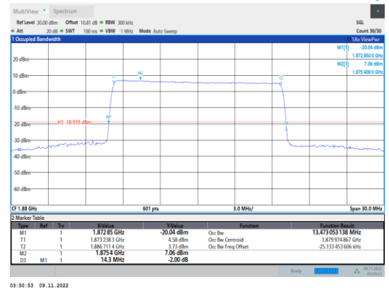
Band2-15MHz-16QAM-18900-75RB#0
