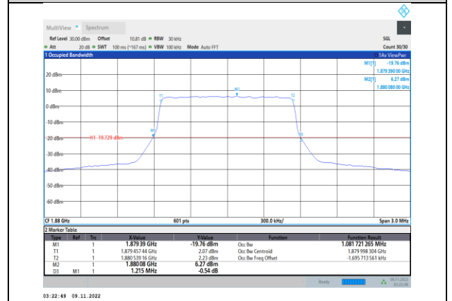
Band2-1.4MHz-16QAM-18900-6RB#0
