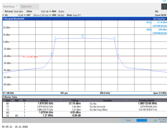
03:05:11 16.11.2022 Band2-1.4MHz-64QAM-18900-6RB#0
