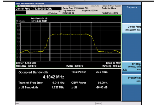
Band4-1513-4.727
