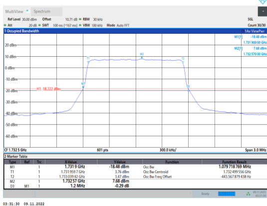
Band4-1.4MHz-QPSK-20175-6RB#0
