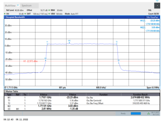
Band4-3MHz-QPSK-19965-15RB#0
