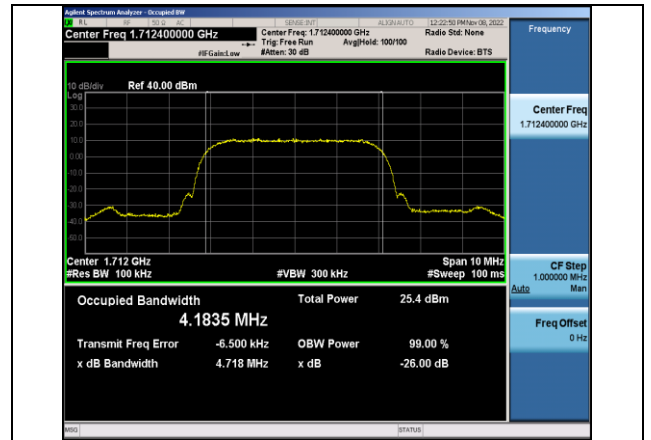
Band4-1312-4.718
