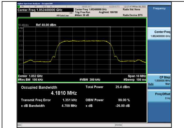
Band2-9262-4.709
