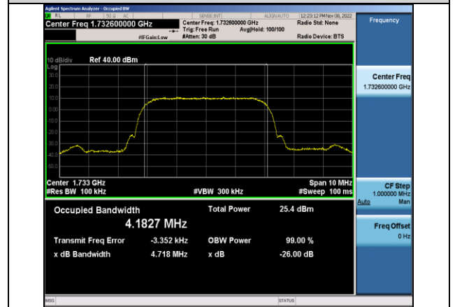
Band4-1413-4.718
