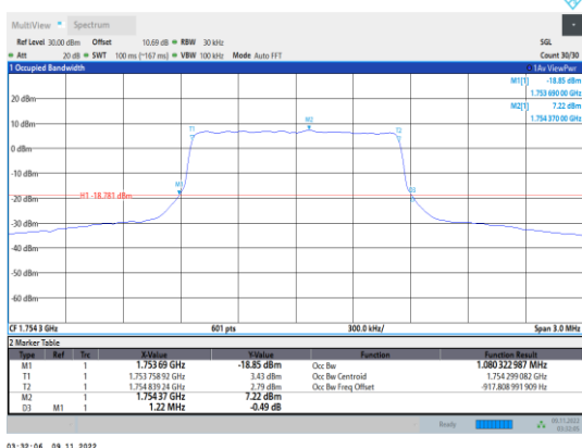
Band4-1.4MHz-QPSK-20393-6RB#0
