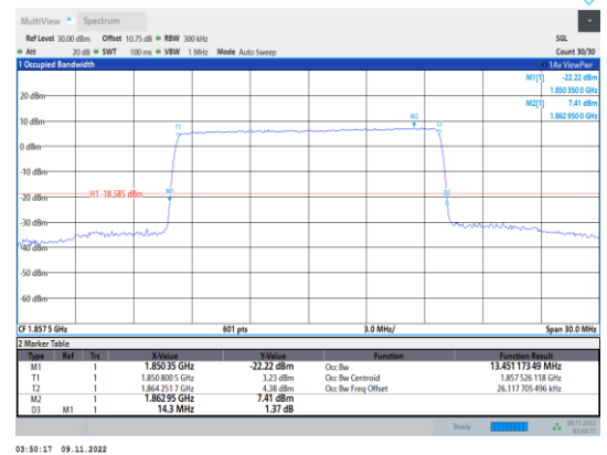
Band2-15MHz-16QAM-18675-75RB#0
