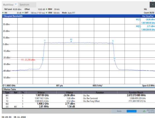
Band2-3MHz-16QAM-19185-15RB#0
