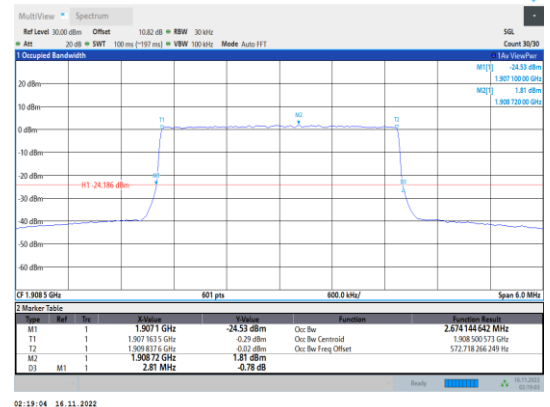
Band2-3MHz-64QAM-19185-15RB#0
