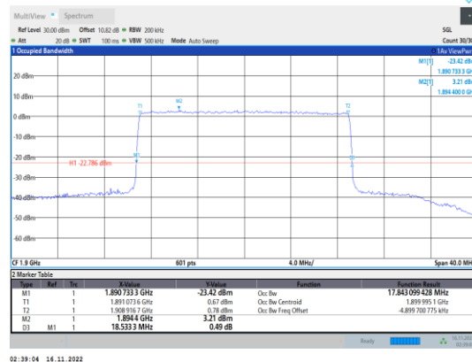
Band2-20MHz-64QAM-19100-100RB#0
