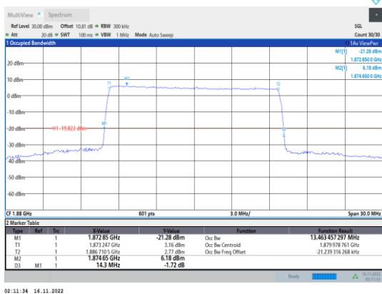
Band2-15MHz-64QAM-18900-75RB#0
