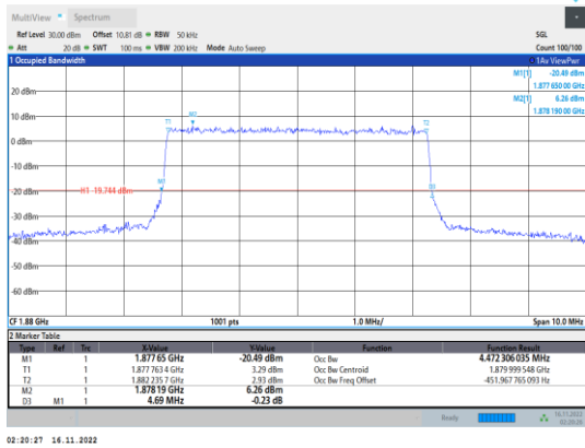
Band2-5MHz-64QAM-18900-25RB#0
