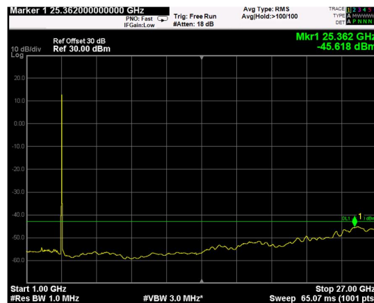
Channel: MIDDLE, Modulation: 256QAM, BW=15MHz, Range: 1GHz - 27GHz
