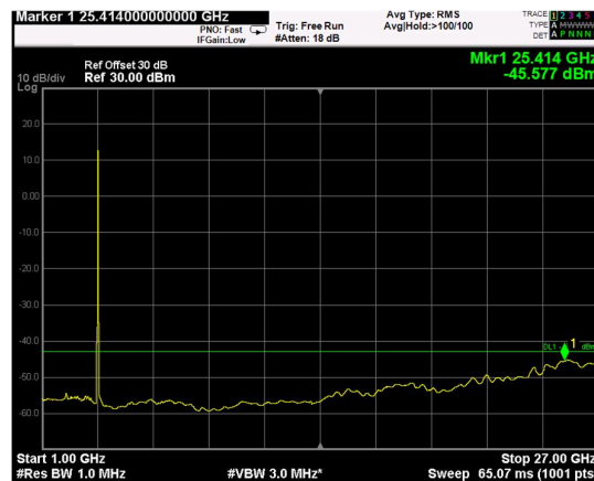
Channel: MIDDLE, Modulation: 256QAM, BW=10MHz, Range: 1GHz - 27GHz
