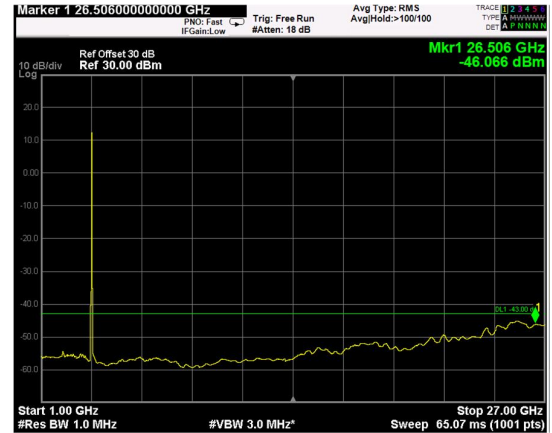
Channel: MIDDLE, Modulation: 16QAM, BW=15MHz, Range: 1GHz - 27GHz
