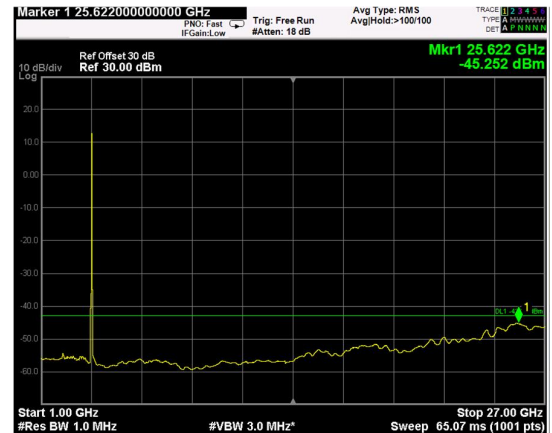
Channel: BOTTOM, Modulation: 256QAM, BW=15MHz, Range: 1GHz - 27GHz
