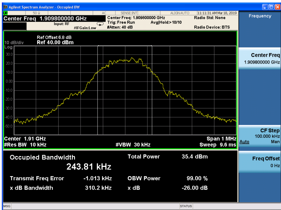
Channel 810
