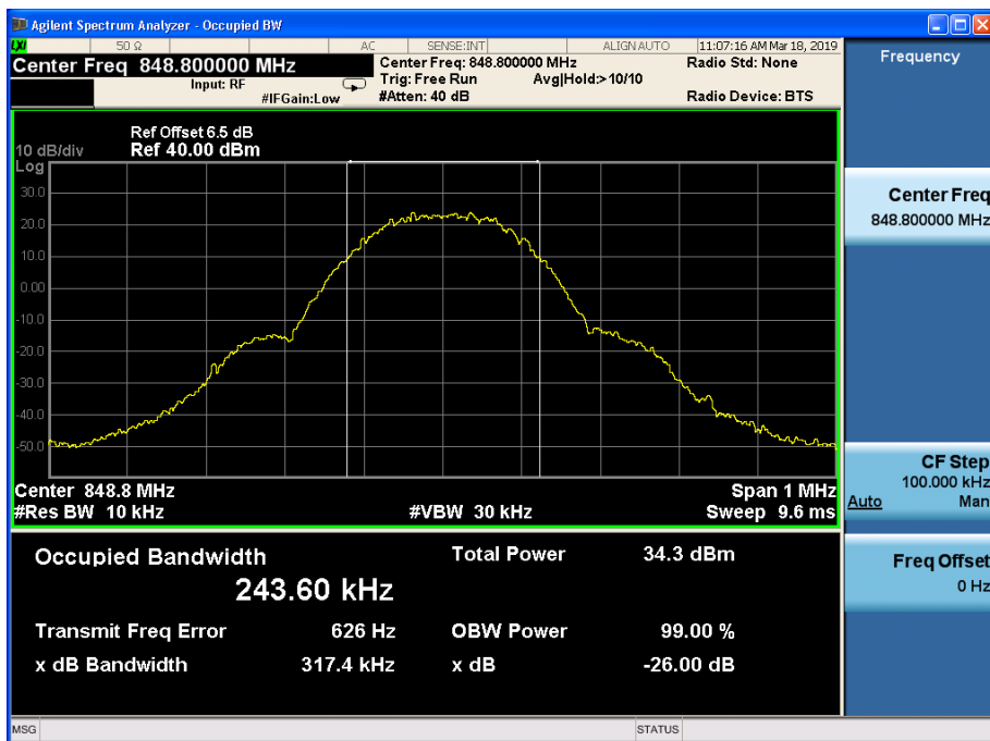
Channel 251
