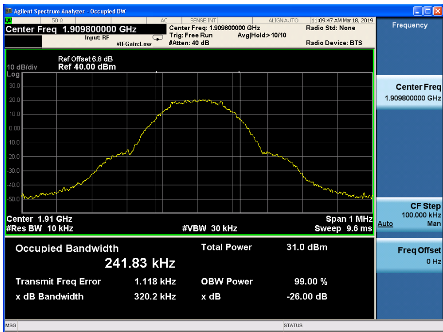
Channel 810
