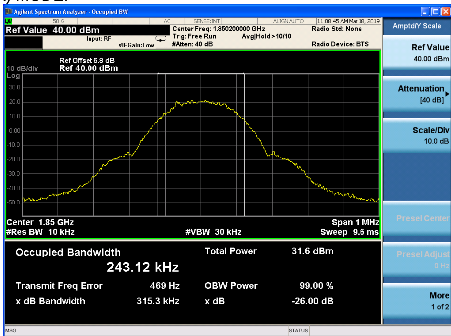
Channel 512
