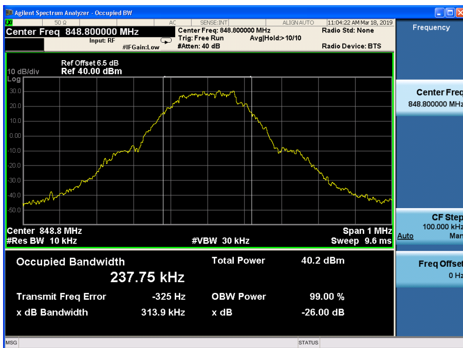
Channel 251
