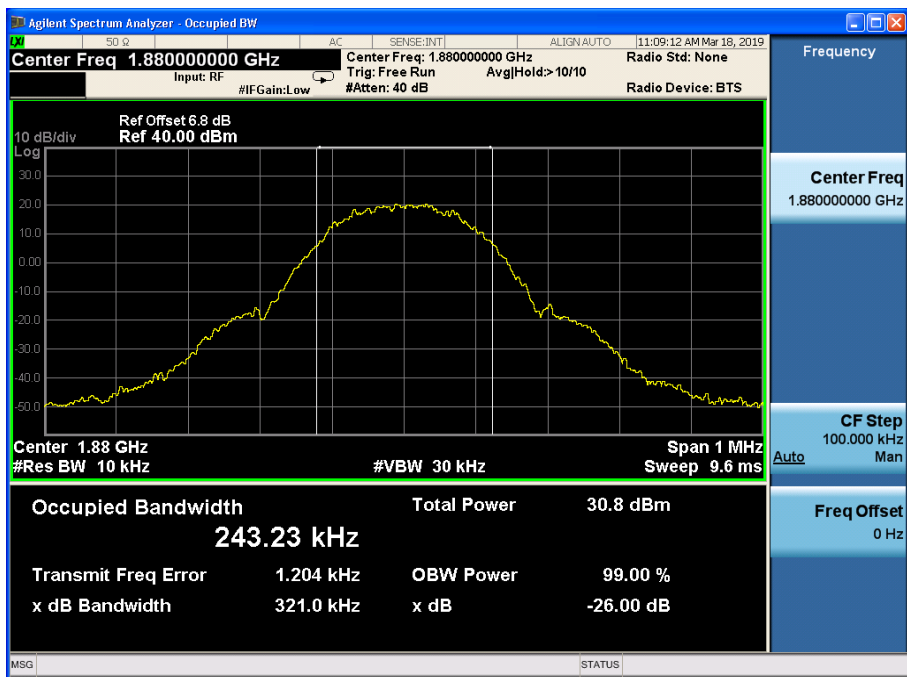
Channel 661
