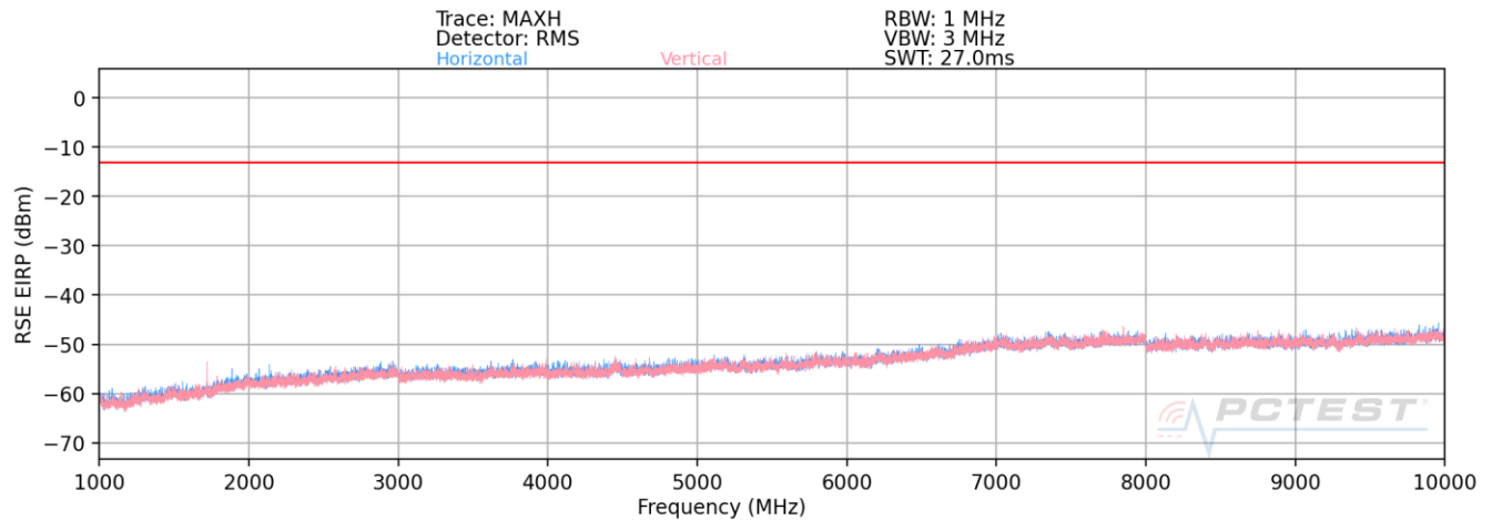
Plot 7-31. Radiated Spurious Plot (LTE Band 8- CAT -M1)
