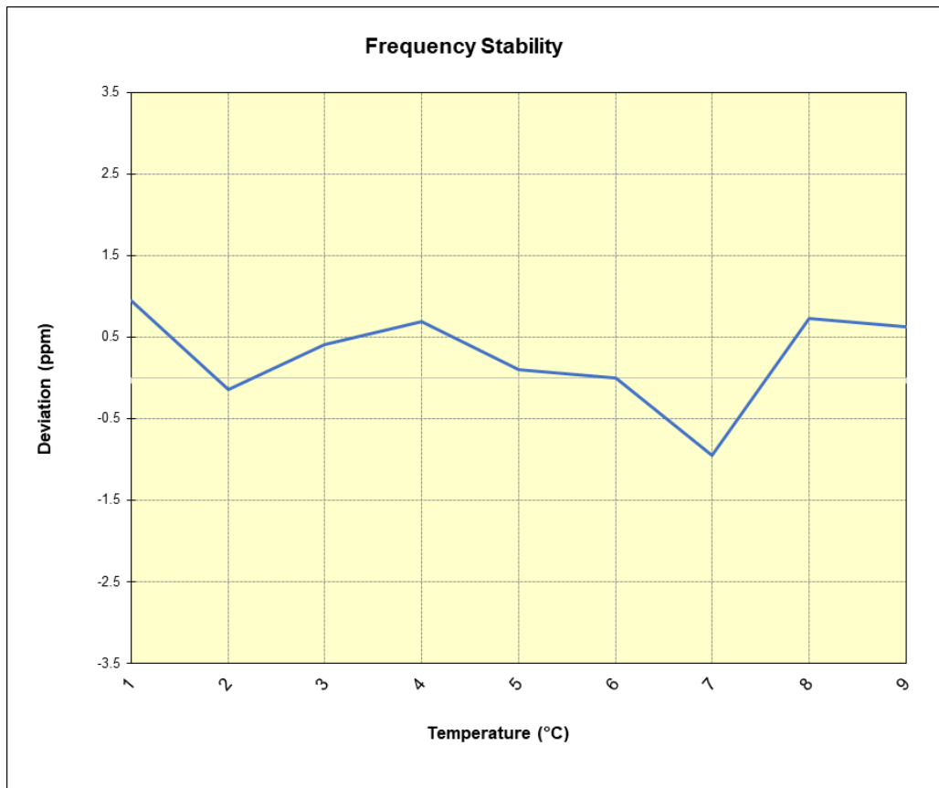
Plot 7-32. LTE Band 8 CAT-M1 Frequency Stability Chart
