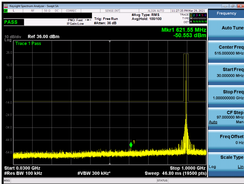
Plot 7-16. Conducted Spurious Plot – Mid Channel (3MHz, QPSK, 1RB, RB Offset 0)
