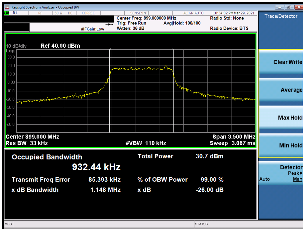
Plot 7-9. Occupied Bandwidth Plot (1.4MHz, 16-QAM, RB 5, RB Offset 0, NB=1)
