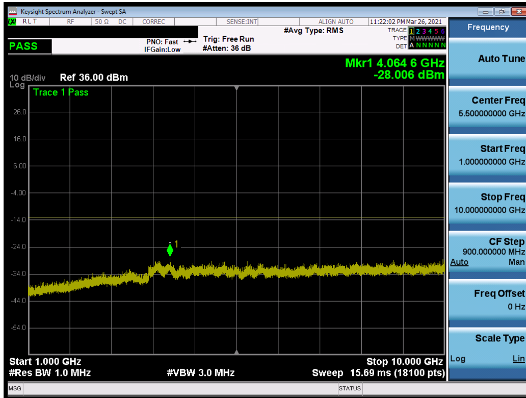
Plot 7-15. Conducted Spurious Plot – Low Channel (1.4MHz, QPSK, 1RB, RB Offset 0)
