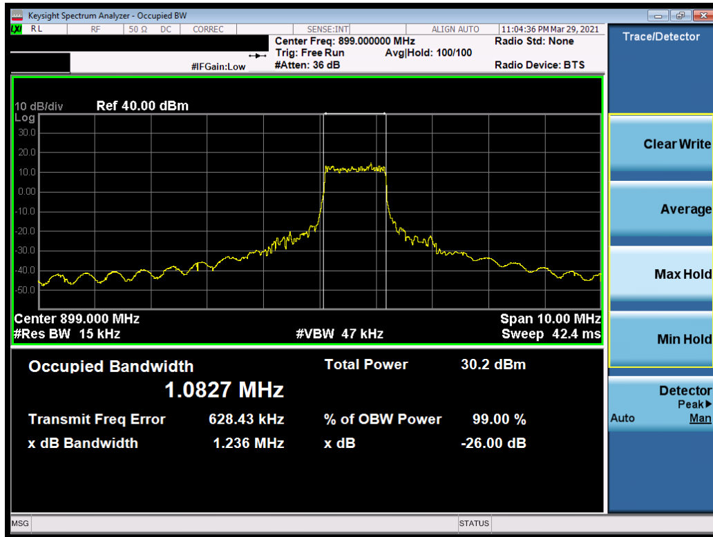
Plot 7-2. Occupied Bandwidth Plot (3MHz, QPSK, RB 6, RB Offset 0, NB=1)
