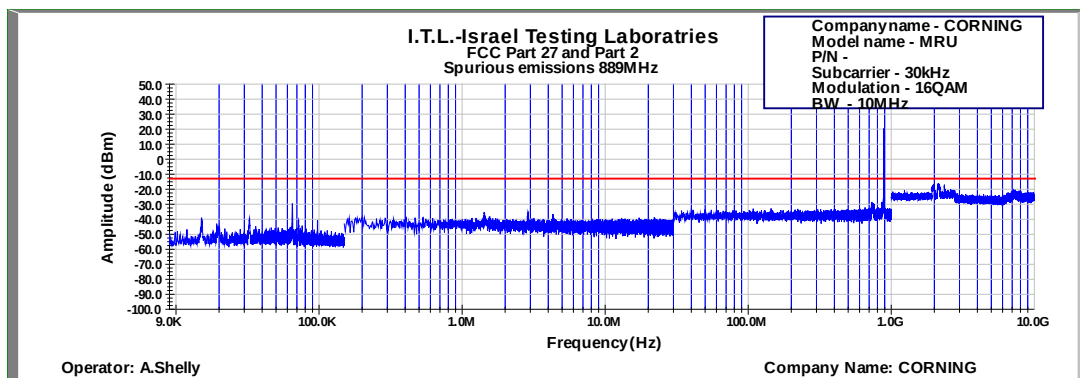
Figure 525: Spurious Emissions at Antenna Terminal 16QAM 10MHz B.W.; 889.MHz, 30kHz
