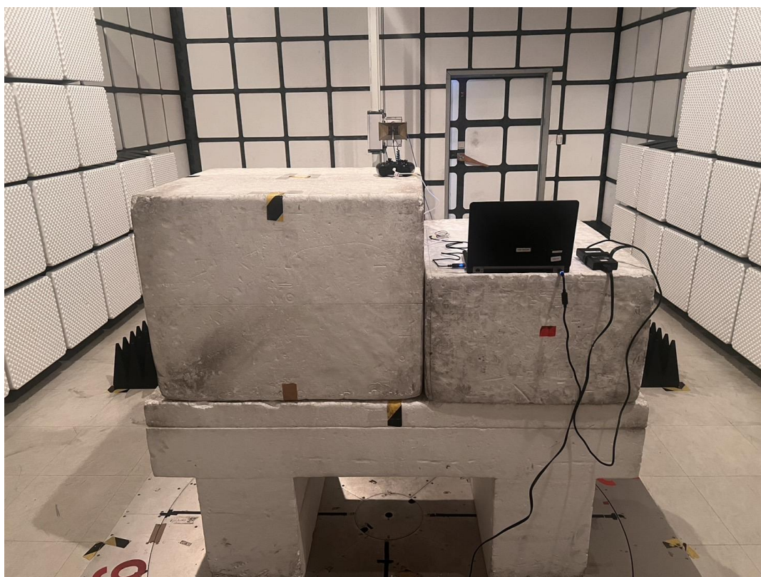
Rear View
