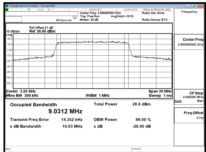
OCC B41 10M CH40190 QPSK
