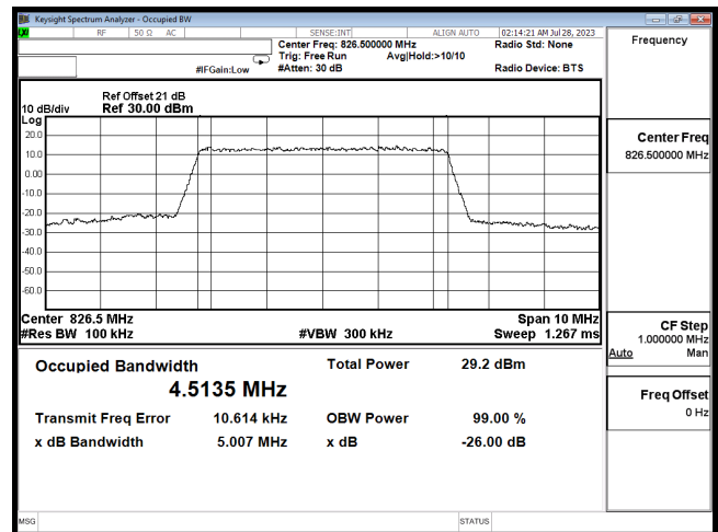
OCC B26 5M CH26815 16QAM
