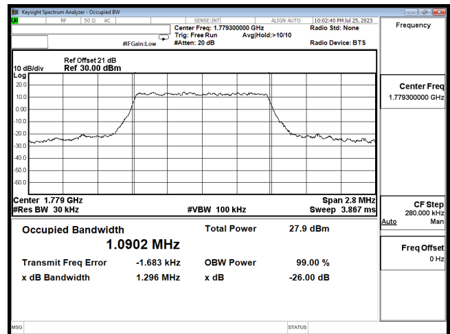
OCC B66 1.4M CH132665 16QAM
