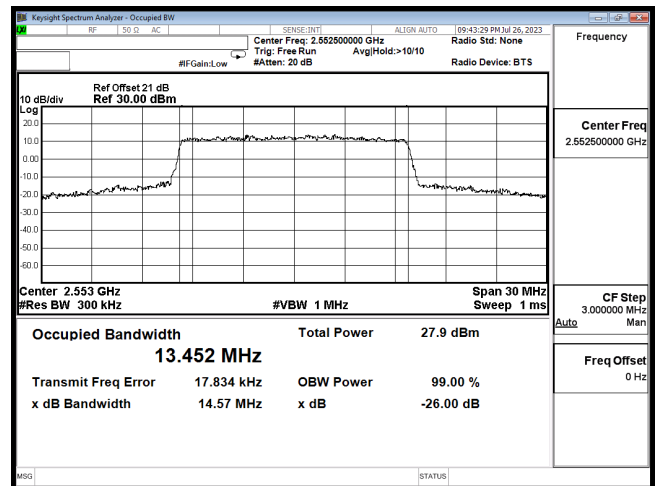
OCC B41 15M CH40215 16QAM
