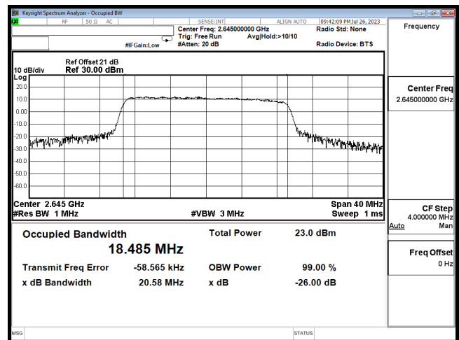
OCC B41 20M CH41140 QPSK
