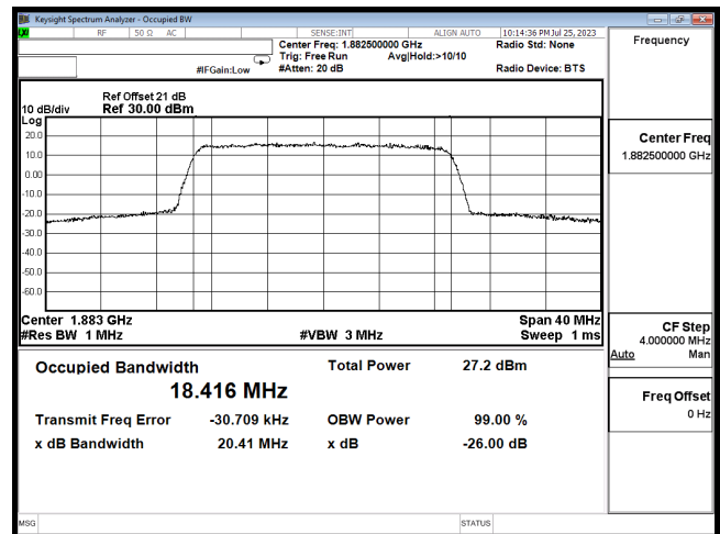
OCC B25 20M CH26365 16QAM
