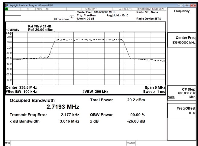
OCC B26 3M CH26915 16QAM
