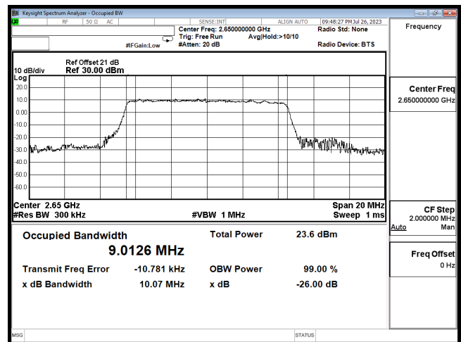
OCC B41 10M CH41190 QPSK
