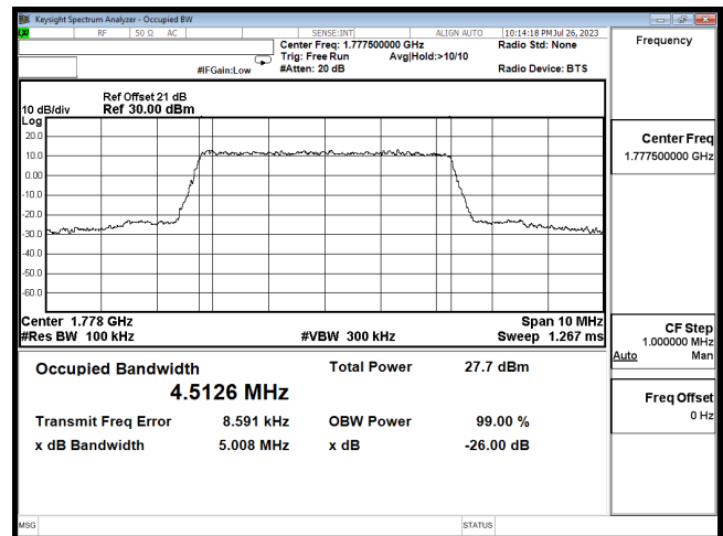
OCC B66 5M CH132647 16QAM
