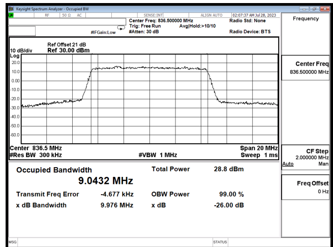
OCC B26 10M CH26915 16QAM
