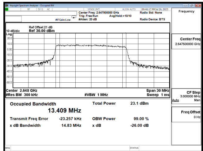
OCC B41 15M CH41165 16QAM
