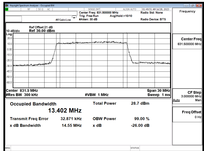
OCC B26 15M CH26865 16QAM
