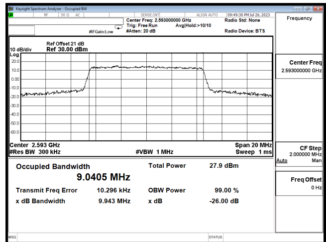
OCC B41 10M CH40620 16QAM
