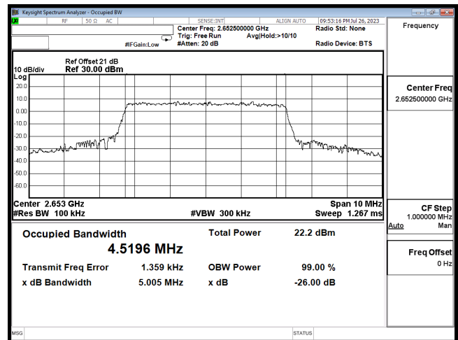
OCC B41 5M CH41215 16QAM
