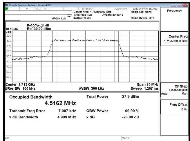
OCC B66 5M CH131997 16QAM
