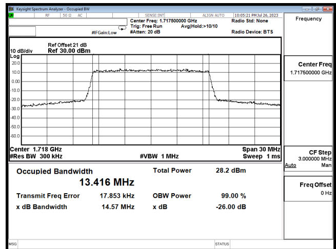
OCC B66 15M CH132047 16QAM
