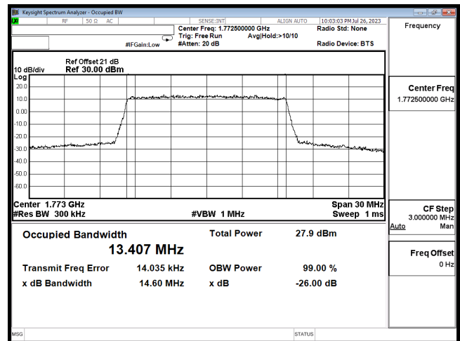
OCC B66 15M CH132597 16QAM
