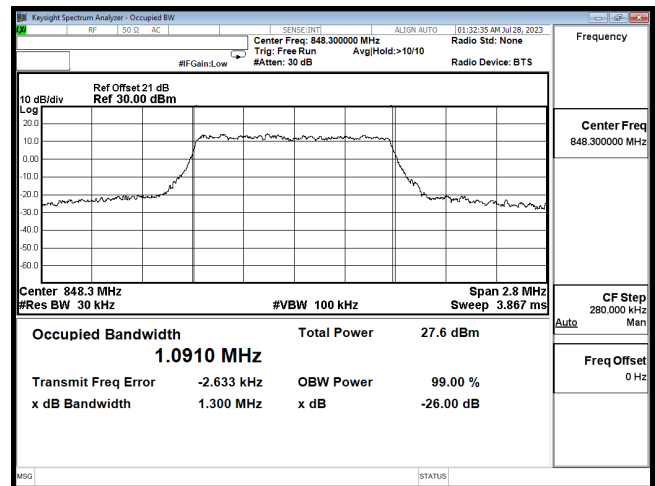
OCC B26 1.4M CH27033 16QAM
