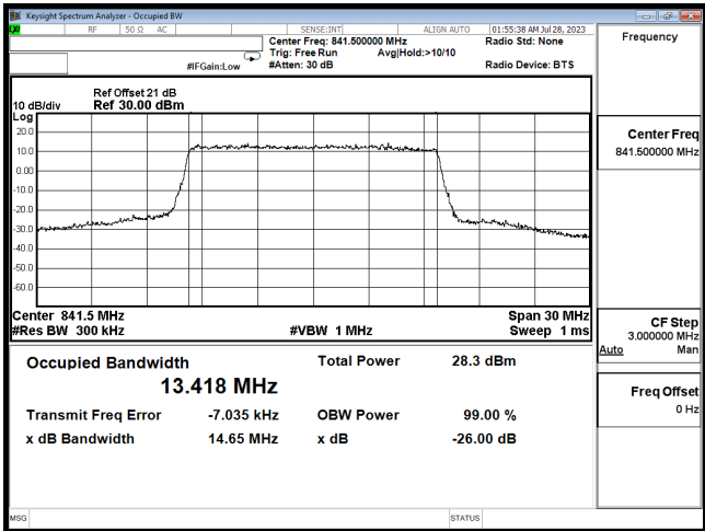
OCC B26 15M CH26965 16QAM
