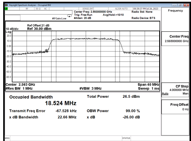
OCC B41 20M CH40620 16QAM
