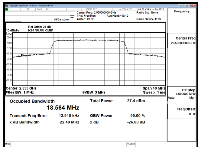
OCC B41 20M CH40240 QPSK
