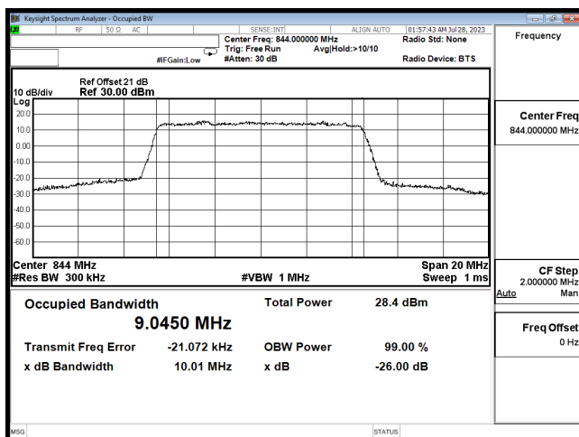
OCC B26 10M CH26990 64QAM
