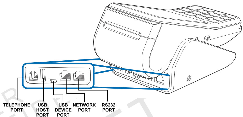
Figure 16 V400m FF Base Connections
