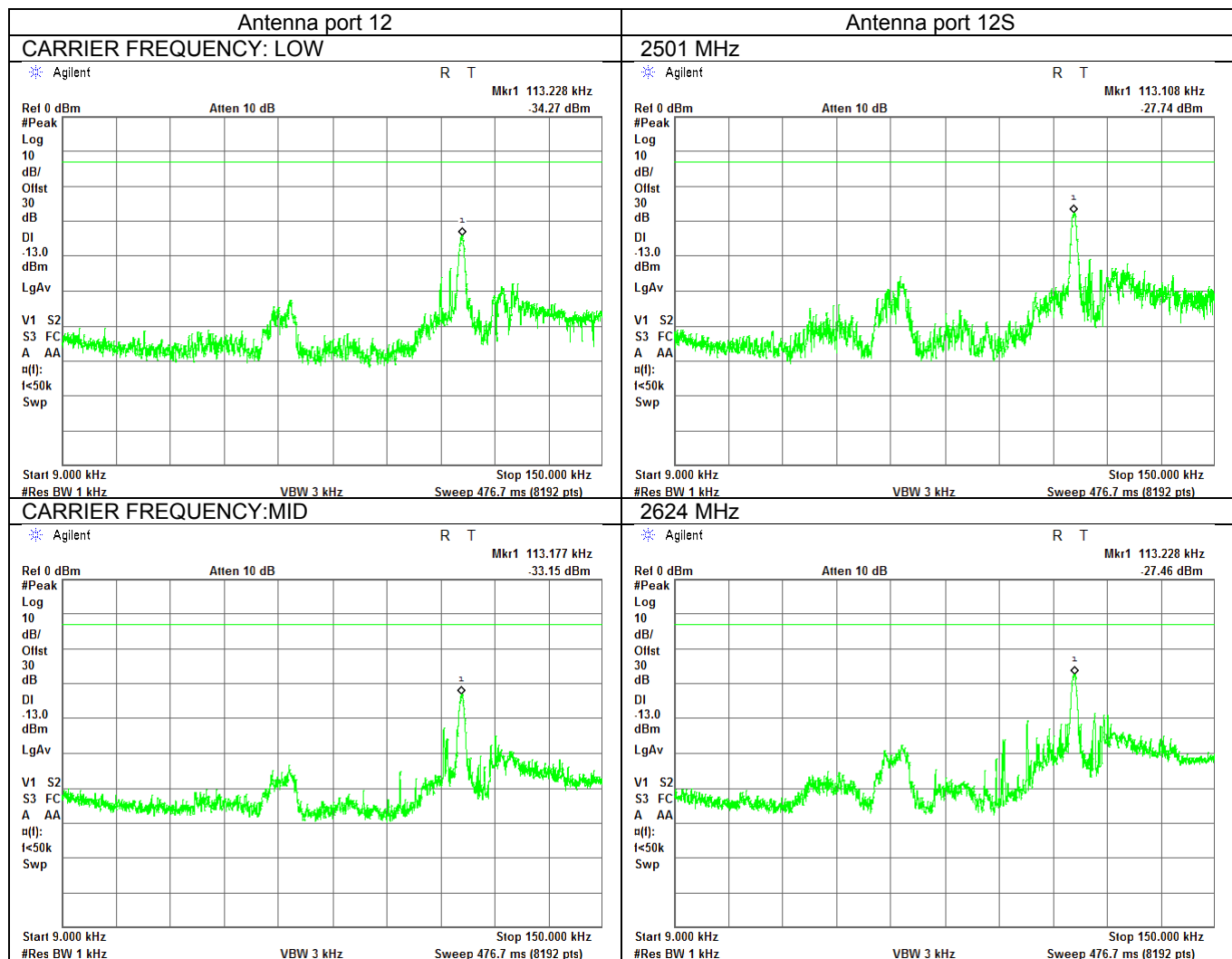
Plot 7.4.1 Spurious emission measurements in 9 - 150 kHz range
