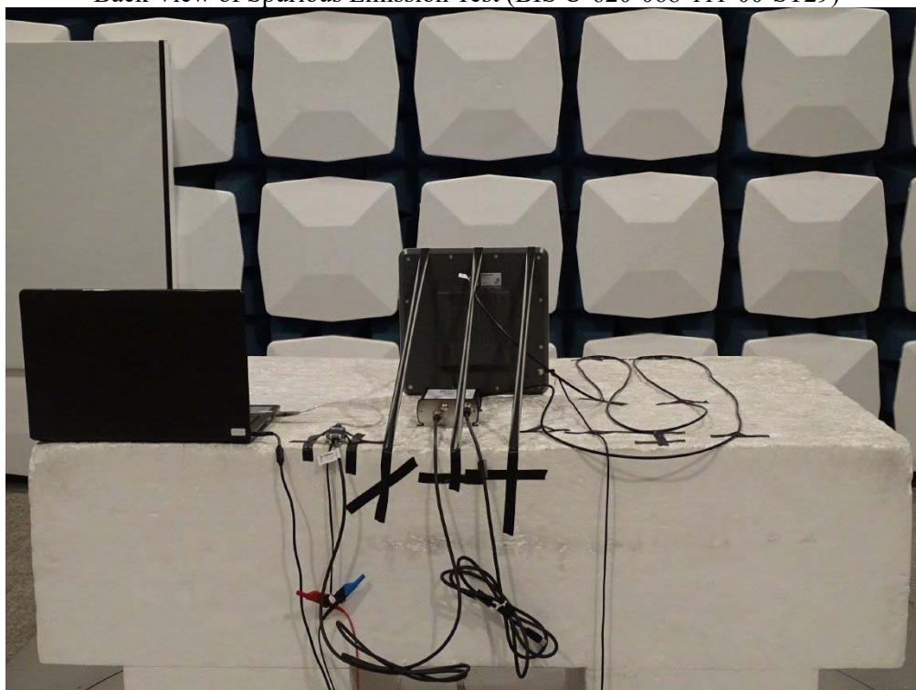
Back View of Spurious Emission Test (BIS U-620-068-111-00-ST29)
