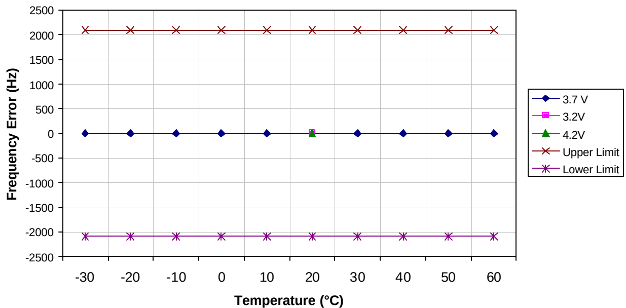
OVFKWC-KX5 CDMA 800 MHz Transmit RF Carrier Stability Over Temperature and Voltage
