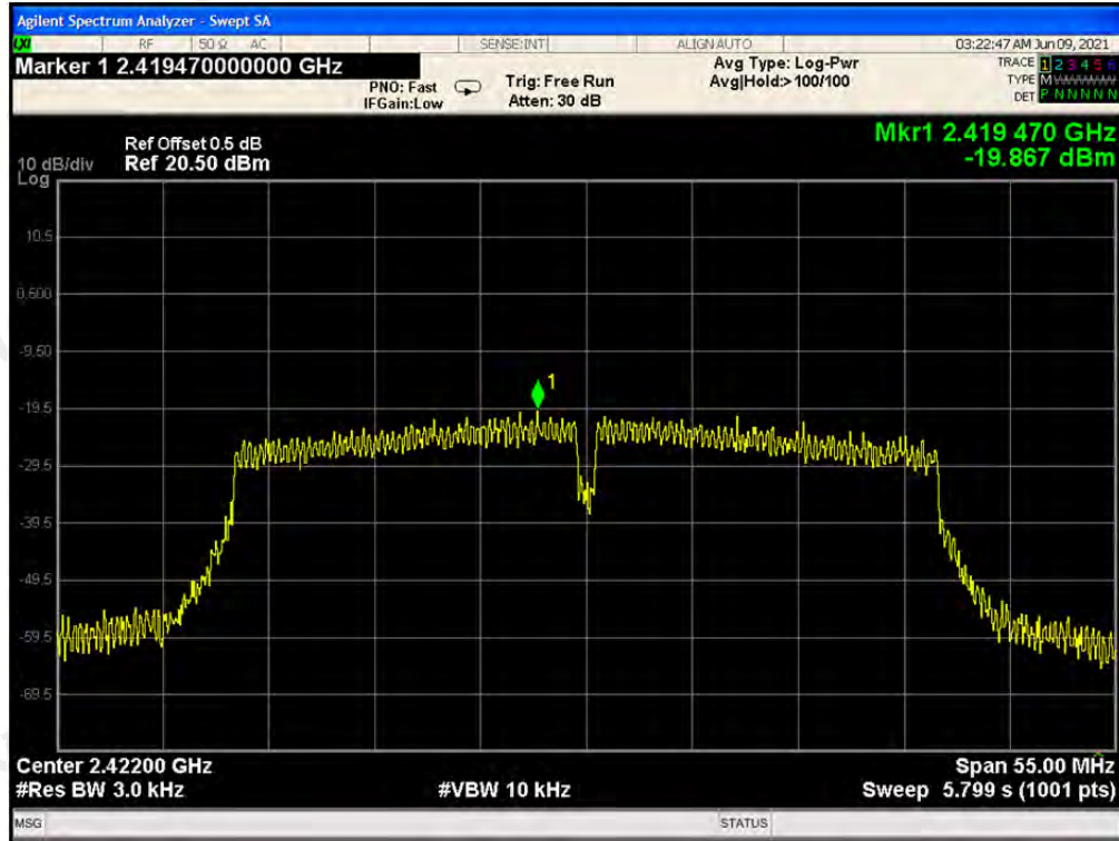
CH3: 2422MHz-ANT1
