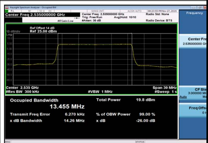
FDD07_MidRange_15MHz_2535MHz_Q16
