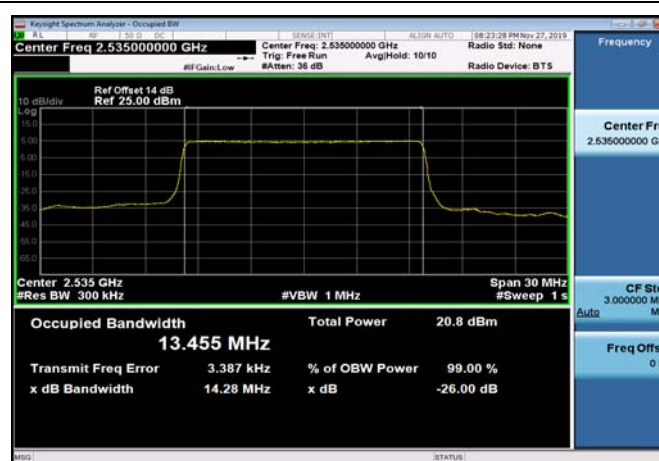
FDD07_MidRange_15MHz_2535MHz_QPSK
