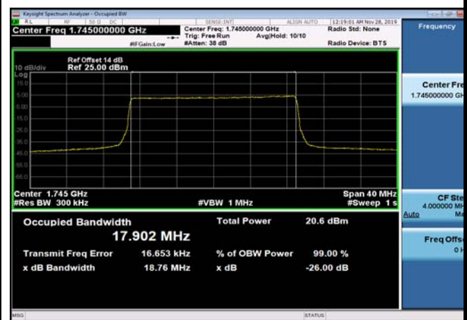
FDD66_MidRange_20_1745_Q16
