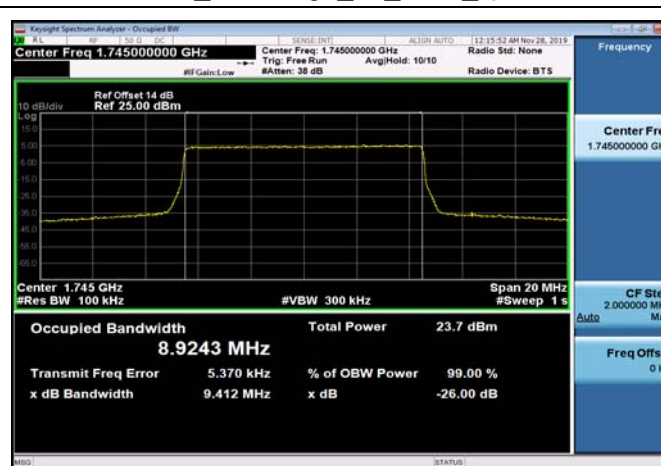
FDD66_MidRange_10_1745_QPSK
