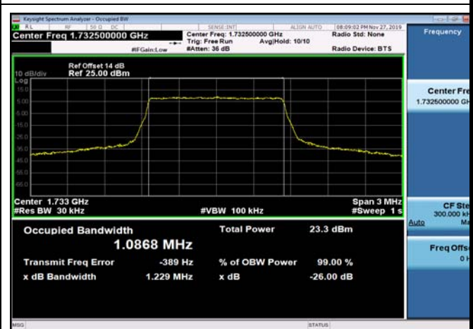
FDD04_MidRange_1.4MHz_1732.5MHz_Q16
