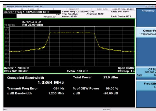
FDD04_MidRange_1.4MHz_1732.5MHz_QPSK
