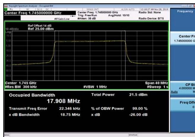
FDD66_MidRange_20_1745_QPSK
