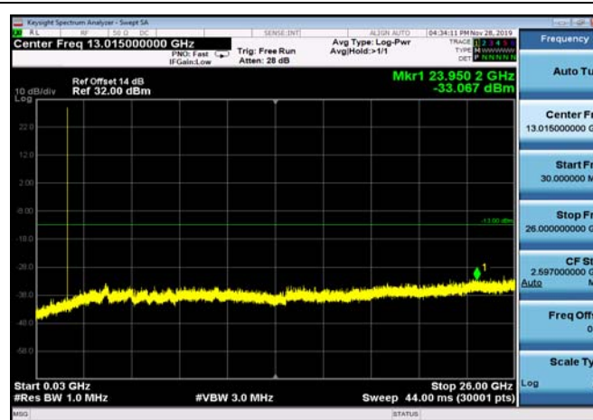
FDD04_MidRange_15MHz_30MHz~26GHz
