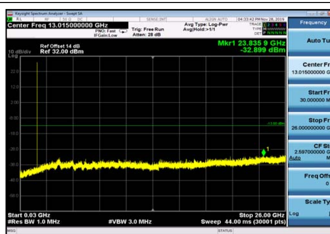
FDD04_LowRange_15MHz_30MHz~26GHz
