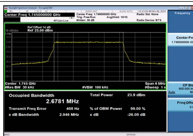
FDD66_MidRange_5_1745_QPSK
