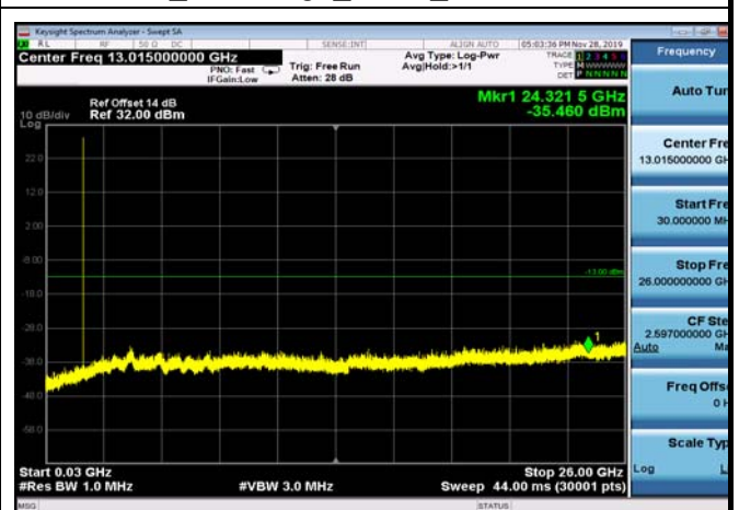
FDD04_LowRange_5MHz_30MHz~26GHz
