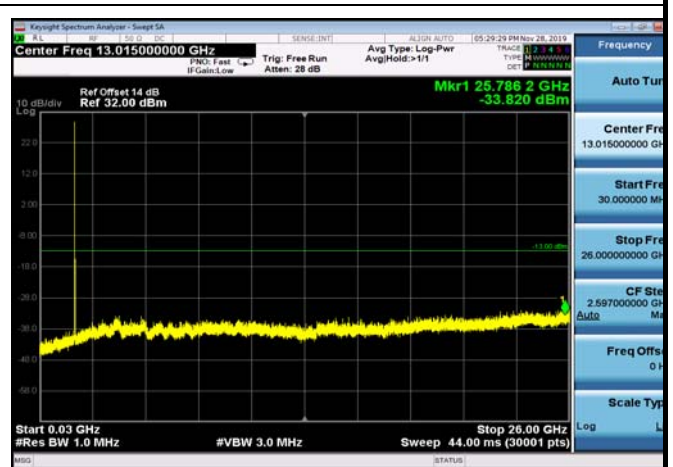
FDD04_HighRange_20MHz_30MHz~26GHz
