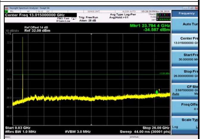
FDD04_LowRange_20MHz_30MHz~26GHz
