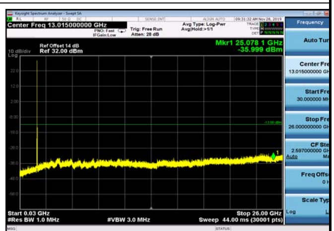
FDD04_HighRange_5MHz_30MHz~26GHz
