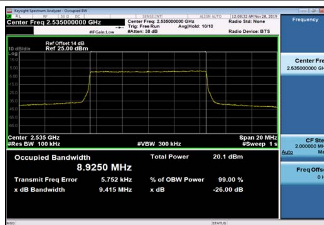
FDD07_MidRange_10_2535_Q16
