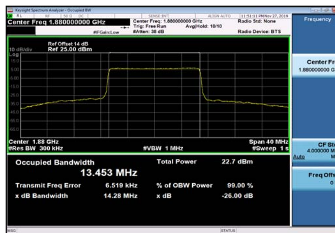
FDD02_MidRange_20_1880_Q16
