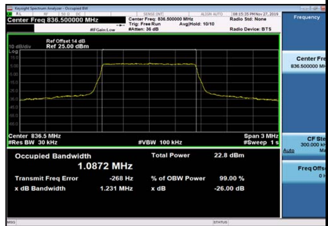
FDD05_MidRange_1.4MHz_836.5MHz _Q16
