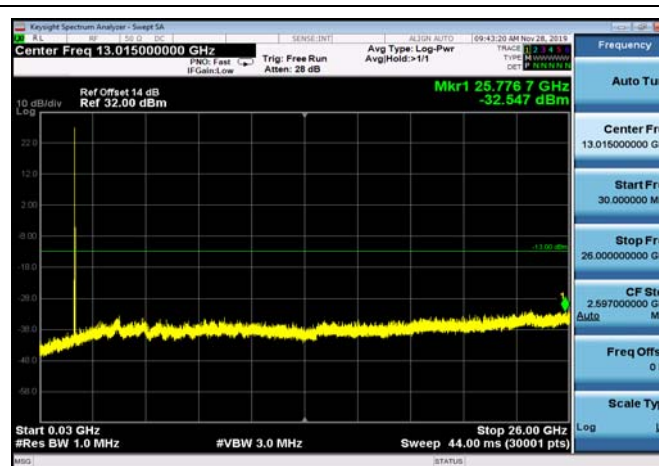
FDD04_HighRange_3MHz_30MHz~26GHz
