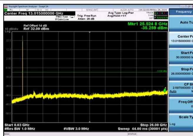
FDD02_LowRange_15MHz_30MHz~26GHz
