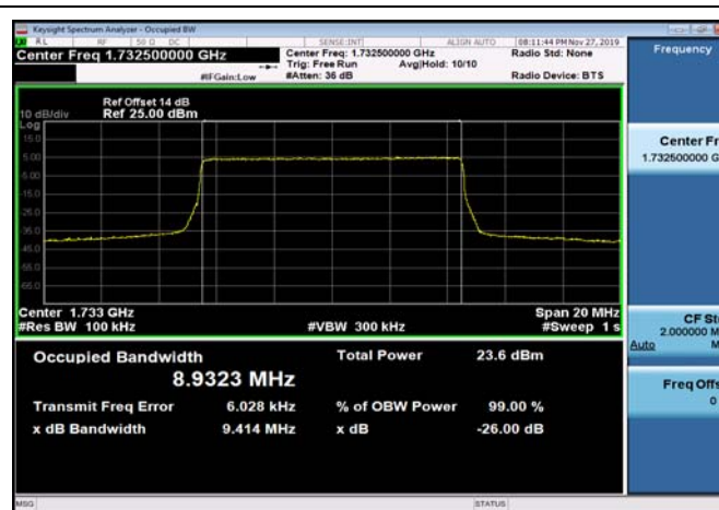
FDD04_MidRange_10MHz_1732.5MHz_QPSK
