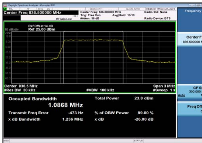
FDD05_MidRange_1.4MHz_836.5MHz _QPSK
