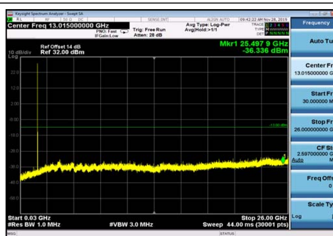
FDD04_LowRange_3MHz_30MHz~26GHz
