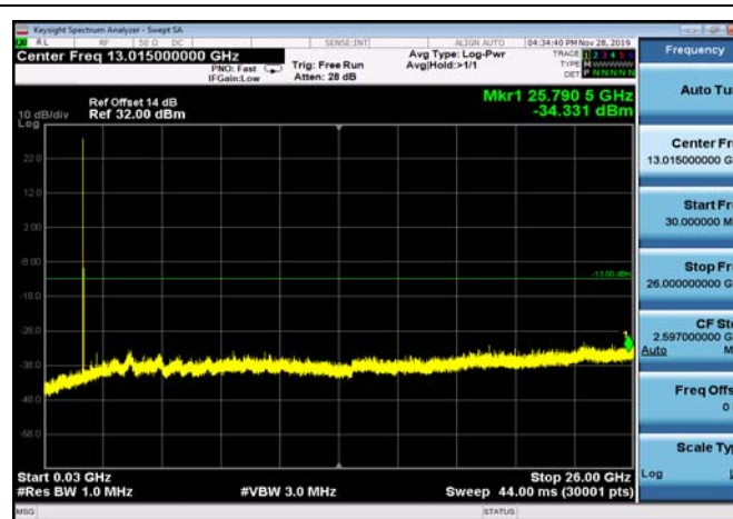
FDD04_HighRange_15MHz_30MHz~26GHz
