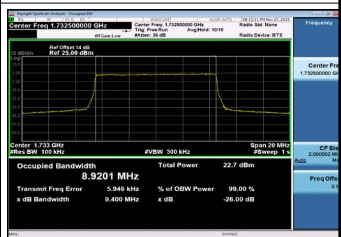
FDD04_MidRange_10MHz_1732.5MHz_Q16
