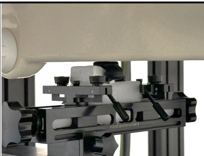
Rear Face of Right Earphone with 0 cm Gap
