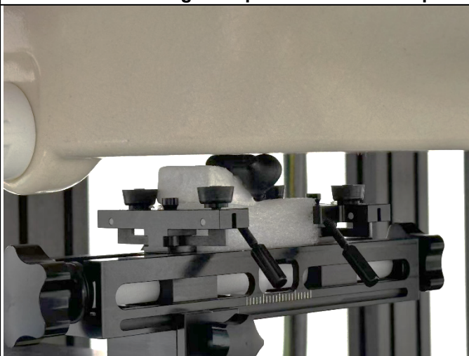
Right Side of Right Earphone with 0 cm Gap
