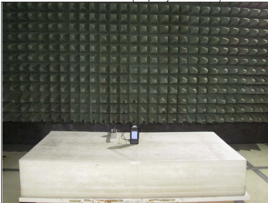
Radiated Emission Test (Frequency above 30MHz)
