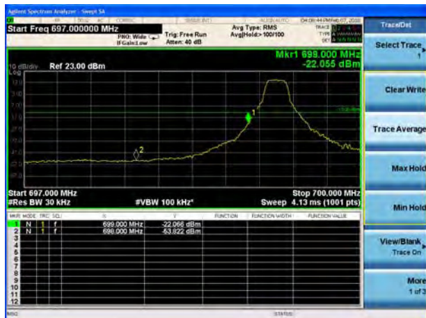
LTE Band 12 16QAM 1.4MHz CH-Low 698MHz~699MHz. 1 RB
