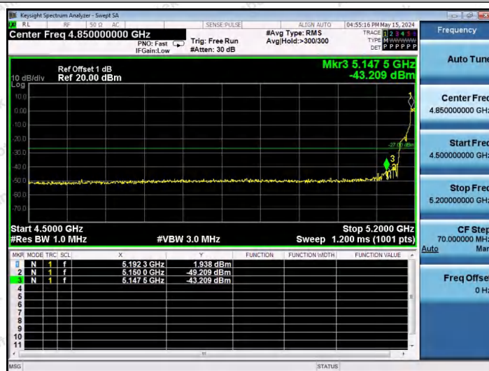
11AX40SISO-Ant1-5190-26Tone-RU17-PASS
