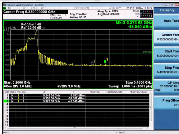
11AX40SISO-Ant1-5230-52Tone-RU44-PASS
