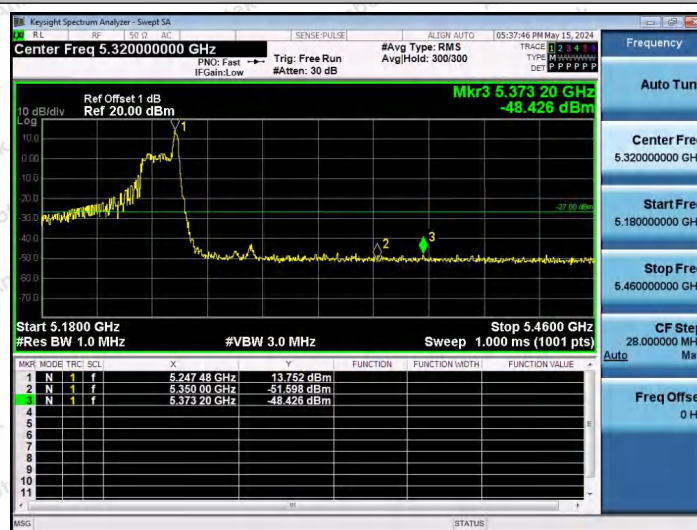
11AX80SISO-Ant1-5210-26Tone-RU36-PASS
