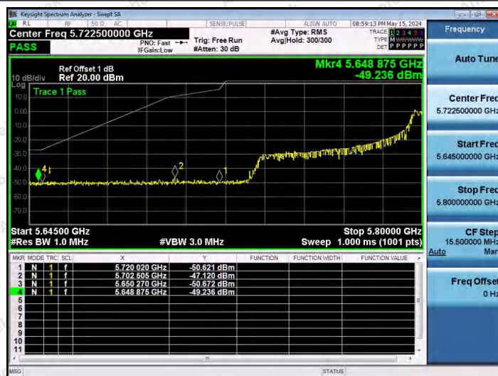
11AX80SISO-Ant1-5775-106Tone-RU60-PASS
