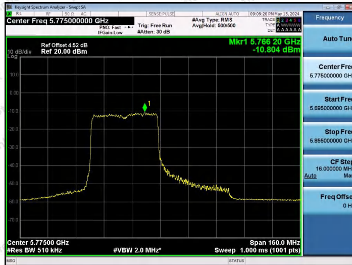
11AX80SISO-Ant1-5775-484Tone-RU65-PASS
