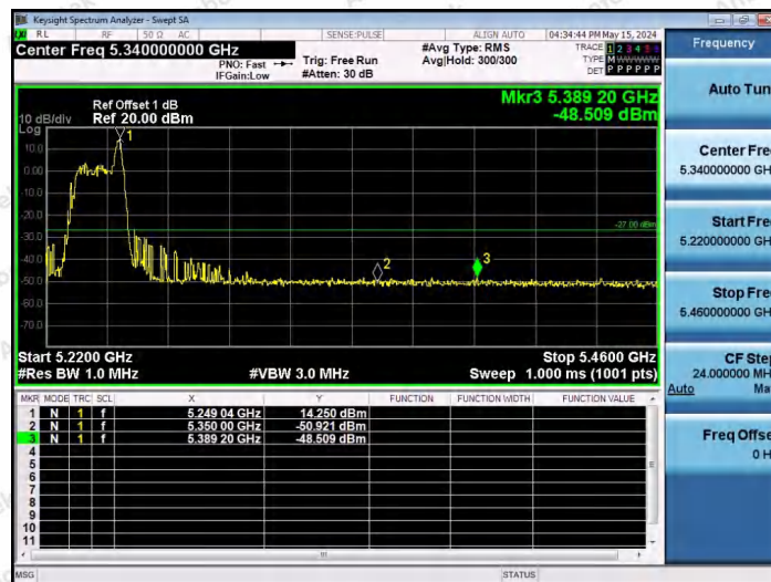
11AX20SISO-Ant1-5240-26Tone-RU5-PASS
