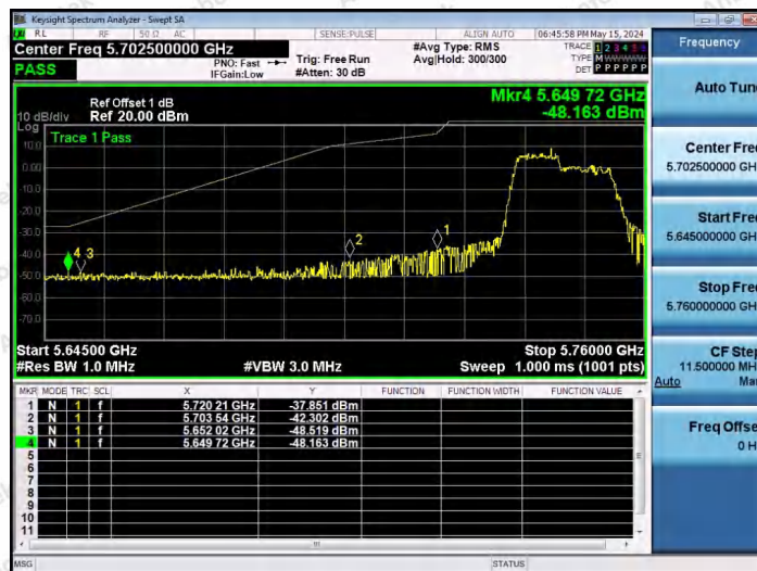
11AX20SISO-Ant1-5745-106Tone-RU53-PASS
