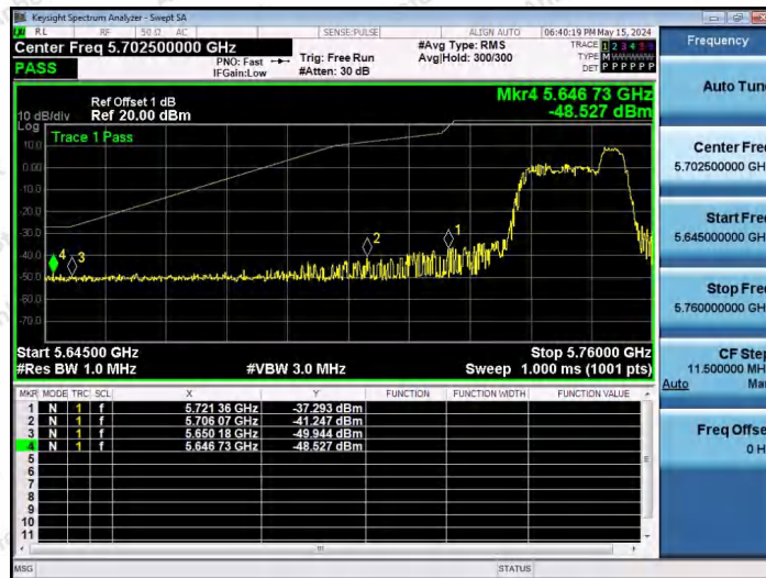
11AX20SISO-Ant1-5745-52Tone-RU40-PASS
