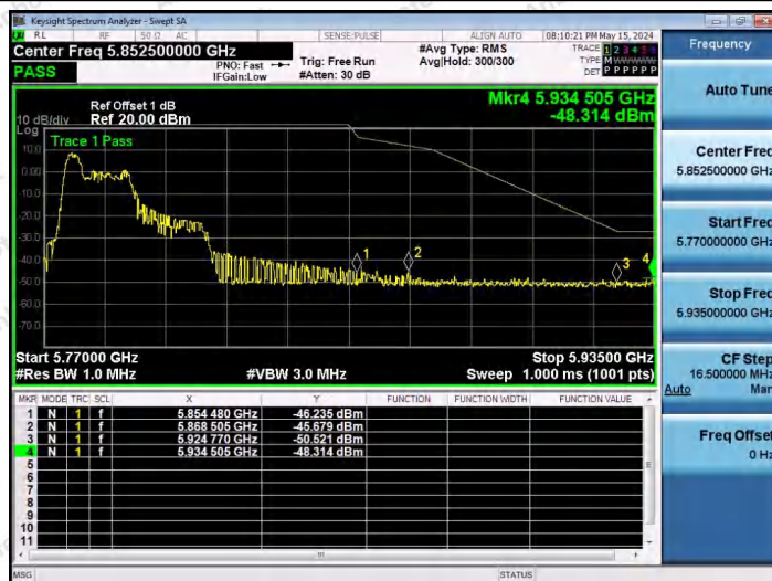
11AX40SISO-Ant1-5795-52Tone-RU37-PASS
