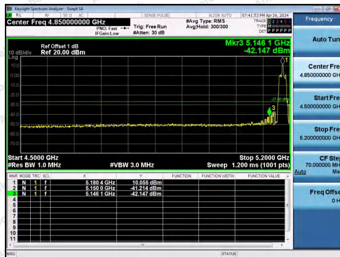
11AX20SISO-Ant1-5180-26Tone-RU4-PASS
