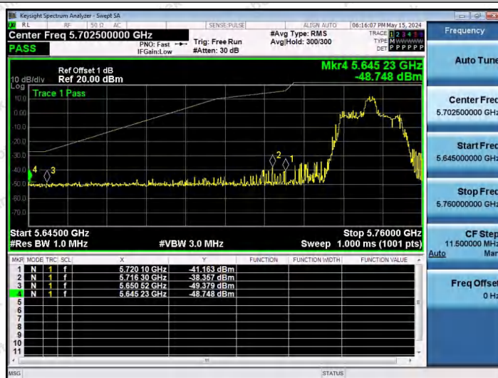
11AX20SISO-Ant1-5745-26Tone-RU4-PASS
