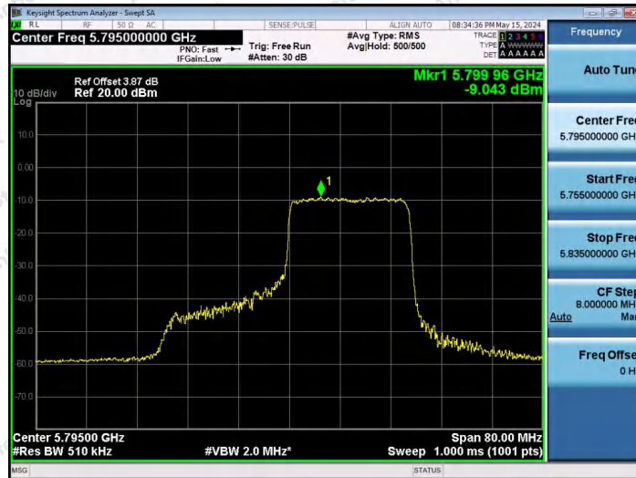
11AX40SISO-Ant1-5795-242Tone-RU62-PASS
