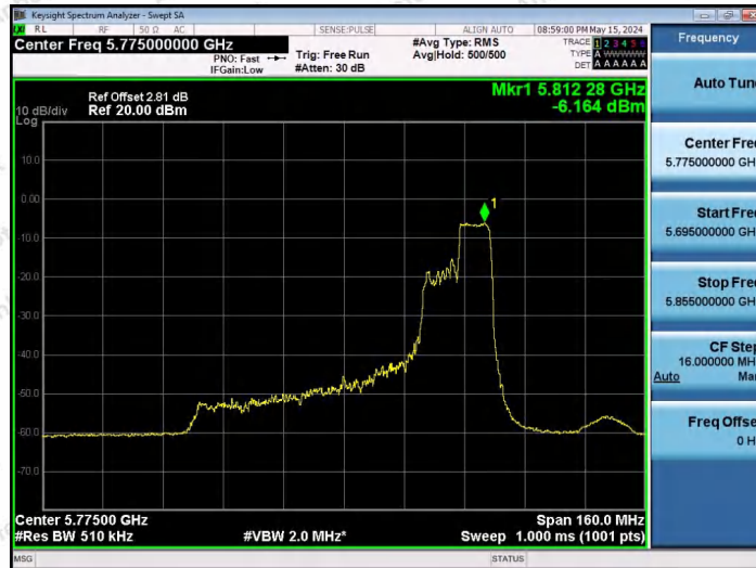
11AX80SISO-Ant1-5775-106Tone-RU60-PASS
