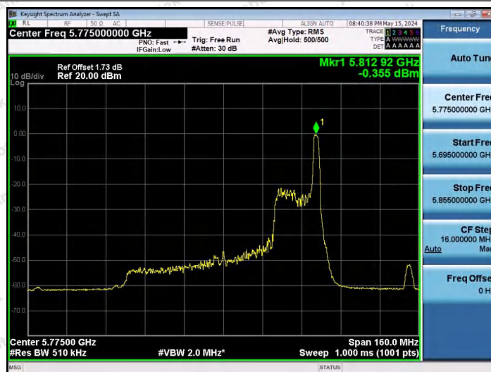
11AX80SISO-Ant1-5775-26Tone-RU36-PASS
