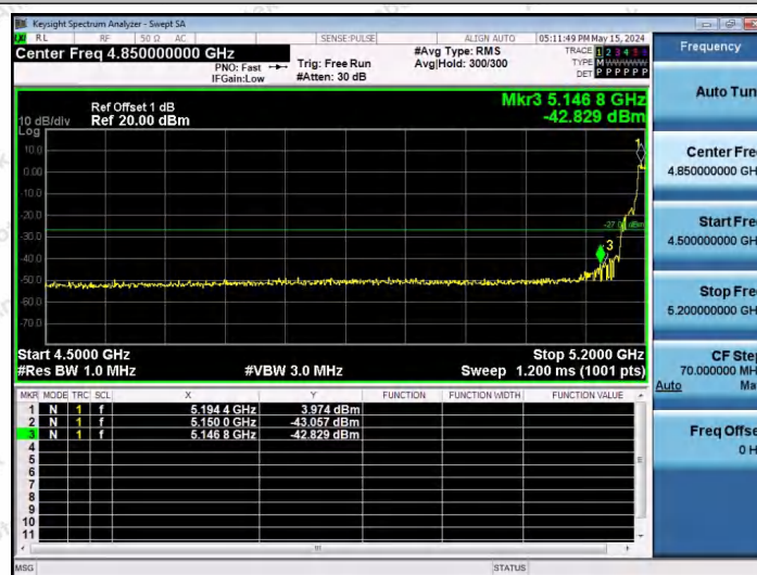
11AX40SISO-Ant1-5190-242Tone-RU62-PASS
