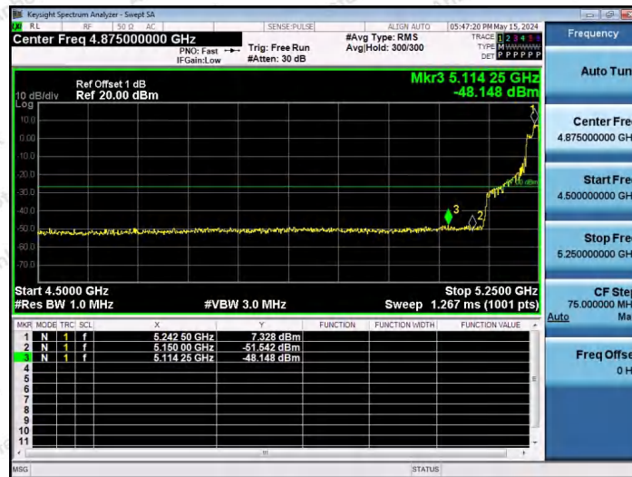
11AX80SISO-Ant1-5210-106Tone-RU60-PASS
