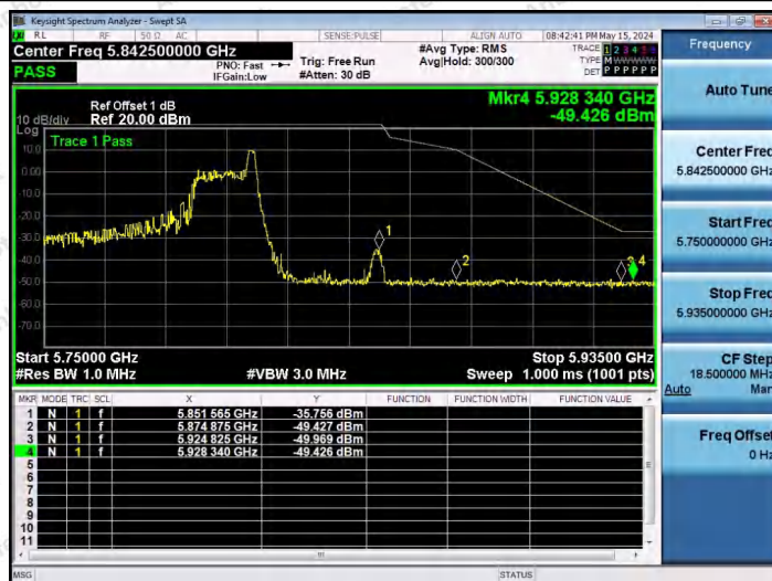
11AX80SISO-Ant1-5775-26Tone-RU36-PASS
