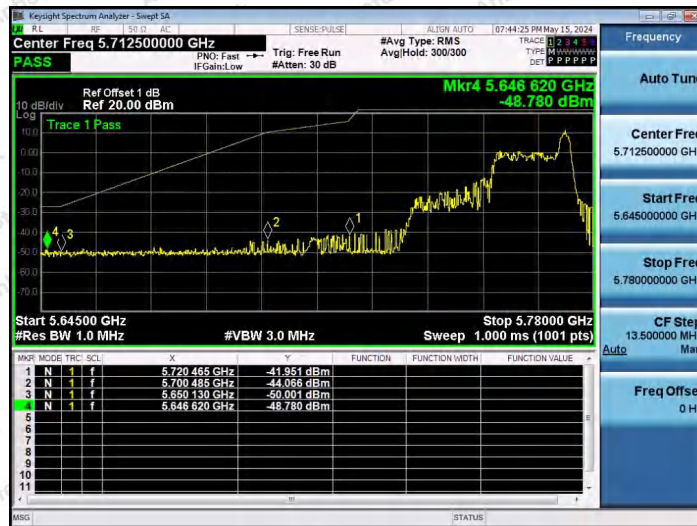
11AX40SISO-Ant1-5755-26Tone-RU17-PASS
