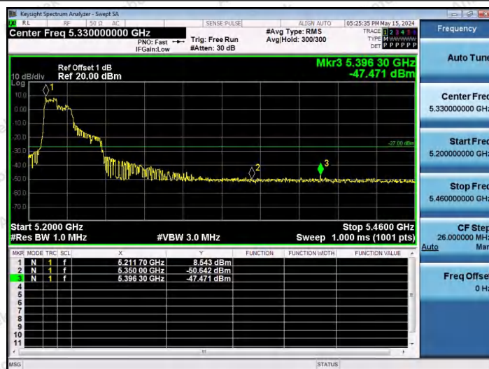
11AX40SISO-Ant1-5230-106Tone-RU53-PASS
