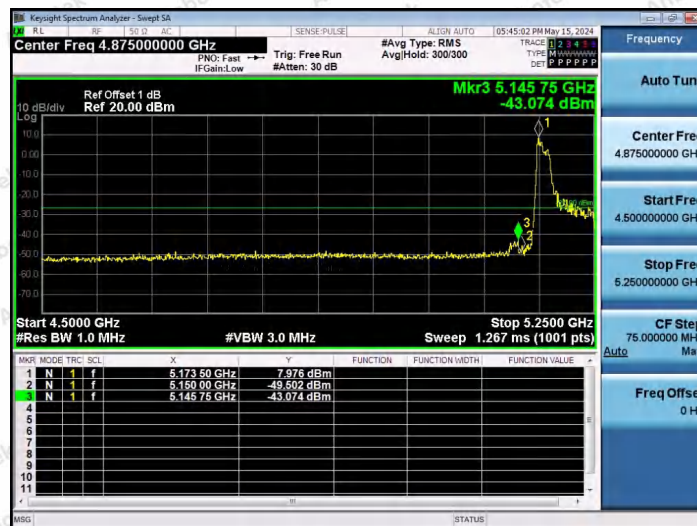
11AX80SISO-Ant1-5210-106Tone-RU53-PASS
