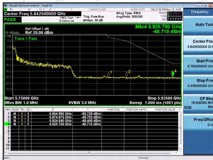
11AX80SISO-Ant1-5775-26Tone-RU0-PASS
