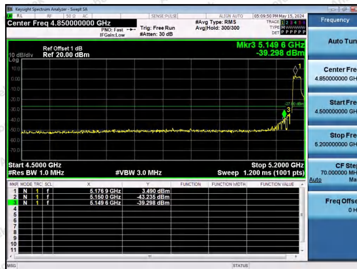
11AX40SISO-Ant1-5190-242Tone-RU61-PASS
