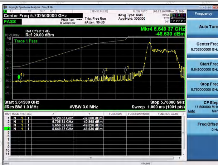
11AX20SISO-Ant1-5745-26Tone-RU0-PASS
