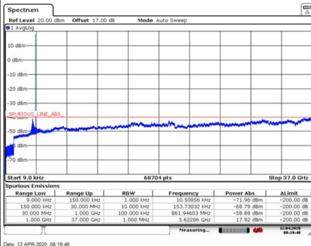
LTE Band 48 5MHz CH Middle 9KHz~37GHz
