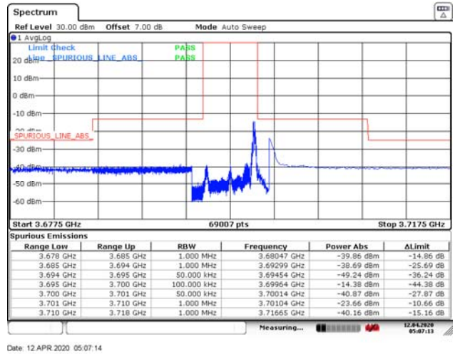
LTE Band 48 QPSK 5MHz CH-High, 100%RB
