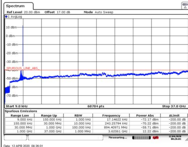
LTE Band 48 10MHz CH Middle 9KHz~37GHz
