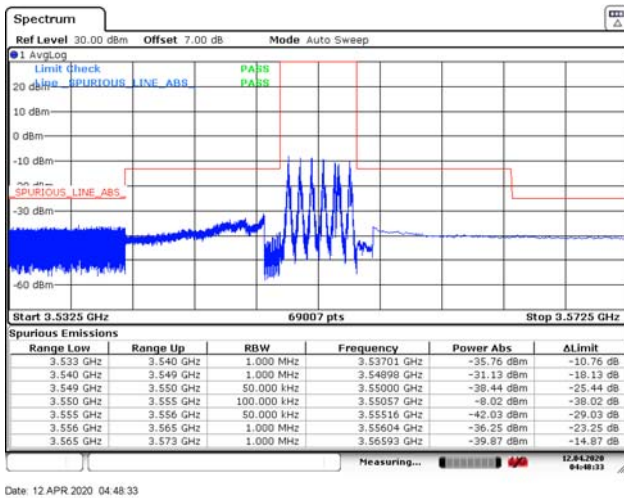
LTE Band 48 QPSK 5MHz CH-Low, 100%RB
