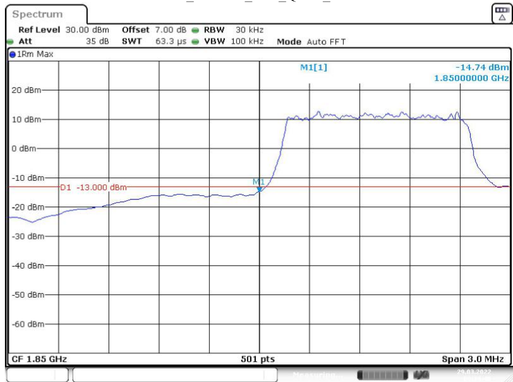
Band 2_1.4 MHz_Low_QPSK_RB6#0
