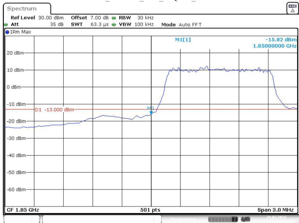
Band 2_1.4 MHz_Low_16QAM_RB6#0
