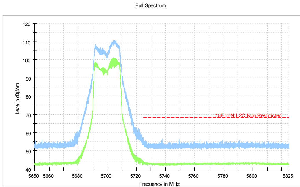
Fig.204 Band Edges (802.11n-HT20, 5700MHz)
