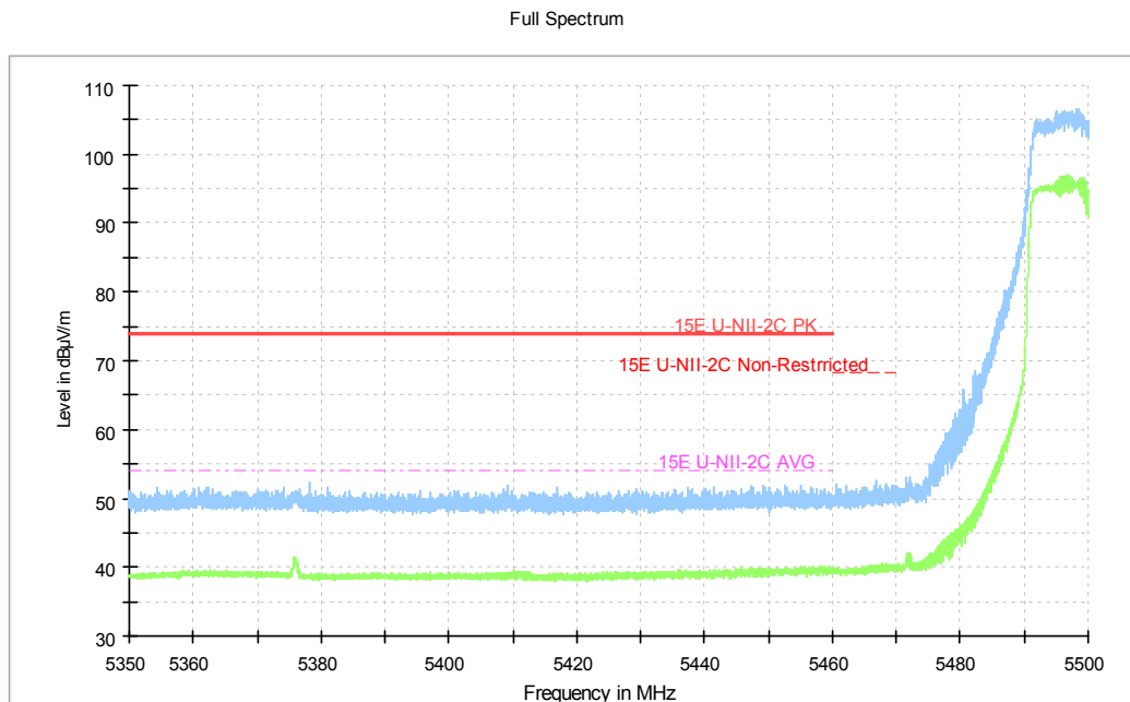
Fig.203 Band Edges (802.11n-HT20, 5500MHz)
