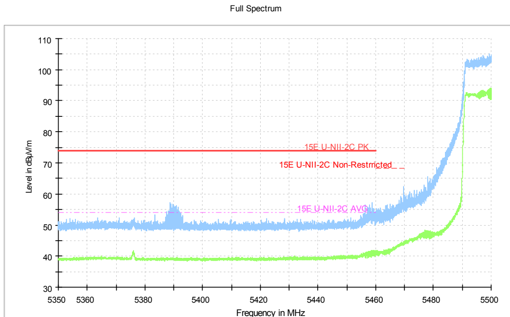
Fig.223 Band Edges (802.11ax-HT40, 5510MHz)
