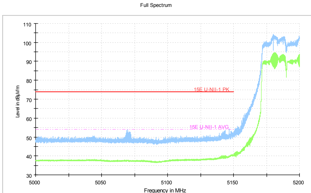
Fig.213 Band Edges (802.11n-HT40, 5190MHz)
