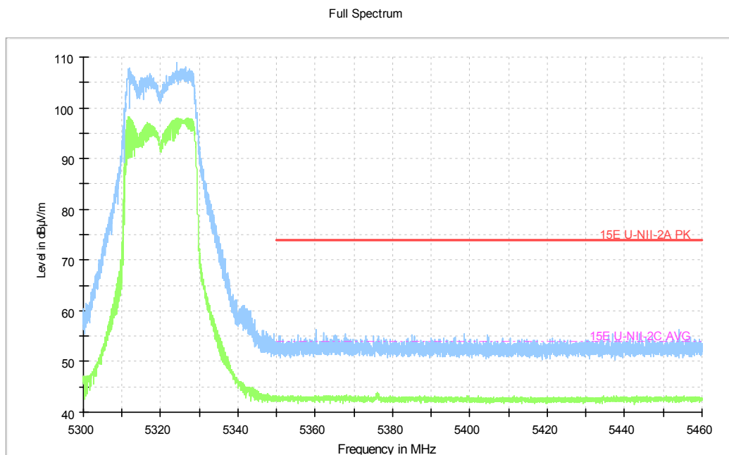
Fig.202 Band Edges (802.11n-HT20, 5320MHz)
