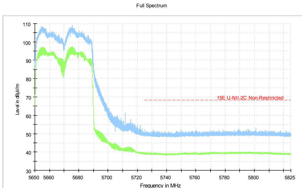
Fig.224 Band Edges (802.11ax-HT40, 5670MHz)
