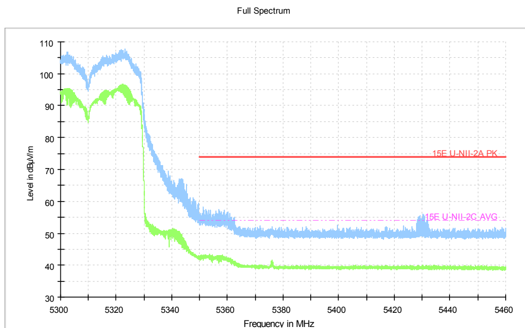
Fig.222 Band Edges (802.11ax-HT40, 5310MHz)
