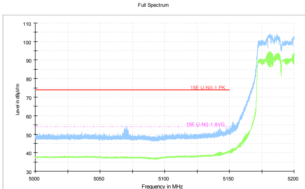
Fig.217 Band Edges (802.11ac-HT40, 5190MHz)
