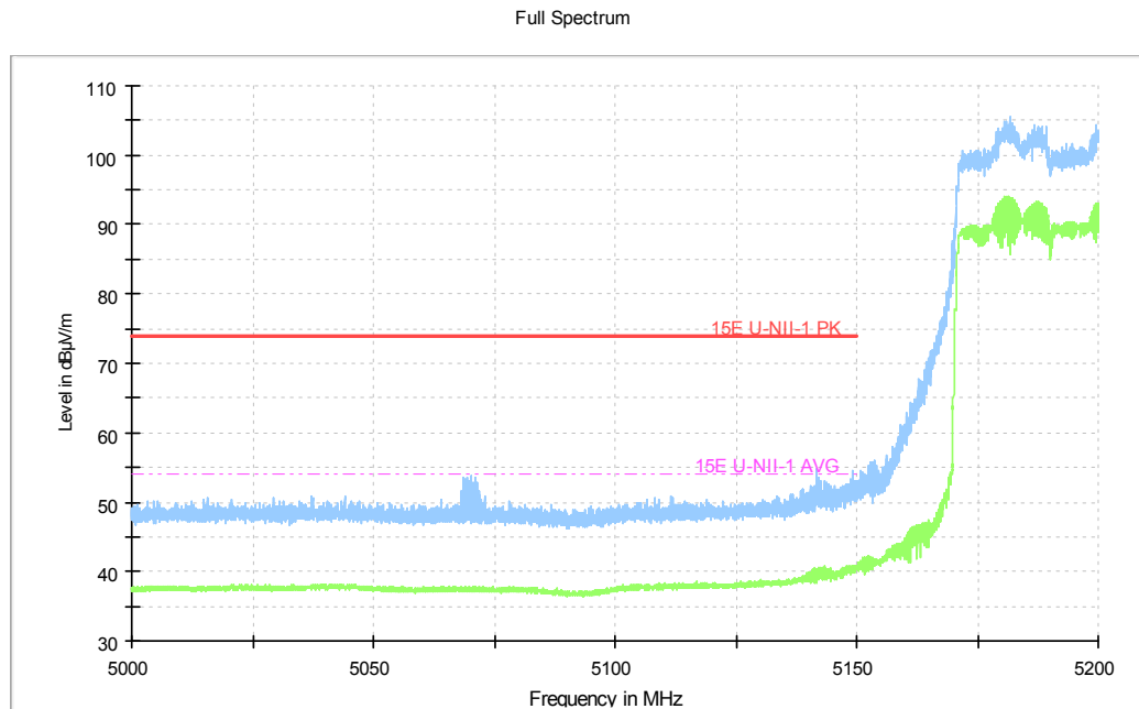
Fig.221 Band Edges (802.11ax-HT40, 5190MHz)
