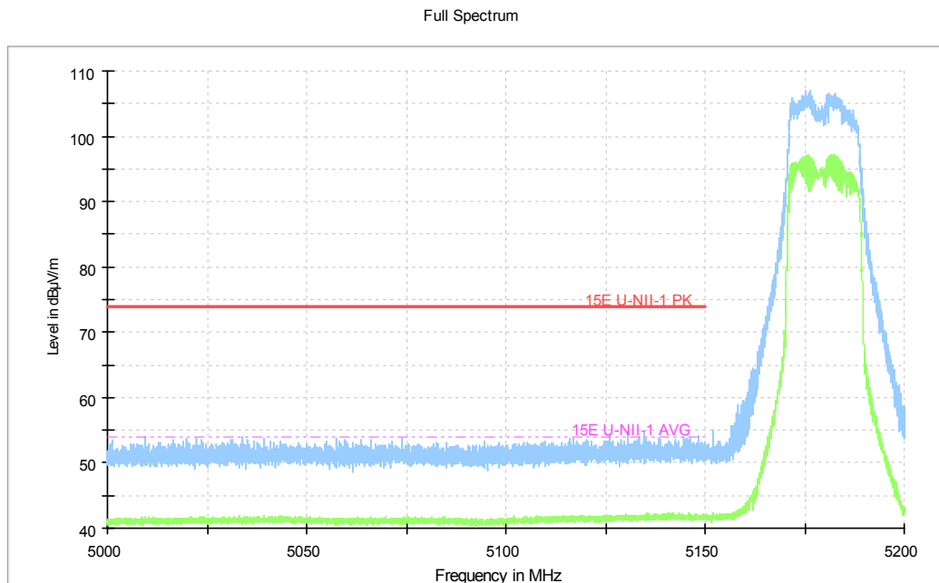
Fig.201 Band Edges (802.11n-HT20, 5180MHz)
