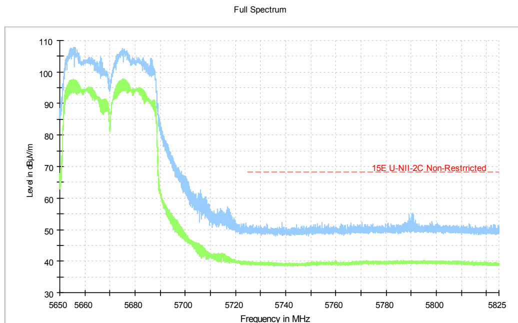
Fig.220 Band Edges (802.11ac-HT40, 5670MHz)
