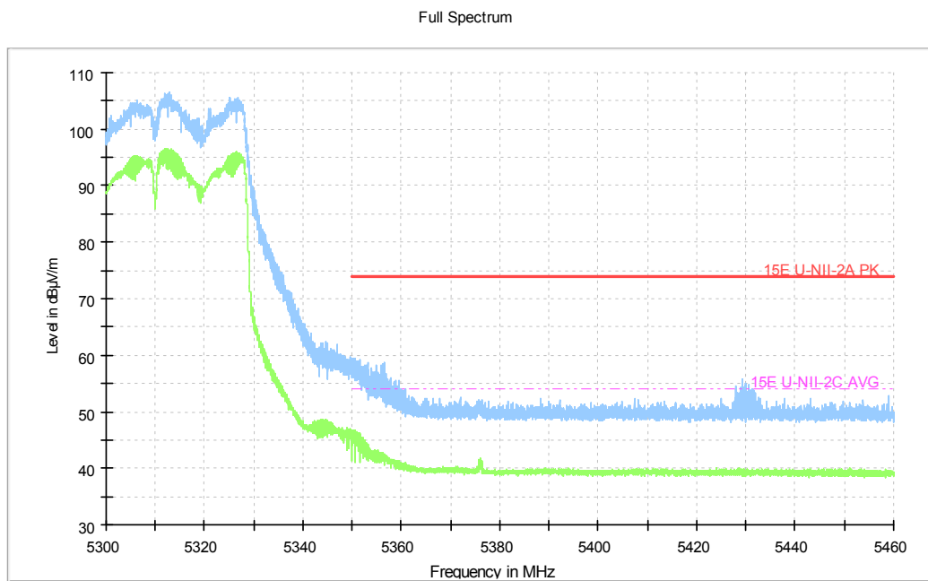
Fig.214 Band Edges (802.11n-HT40, 5310MHz)
