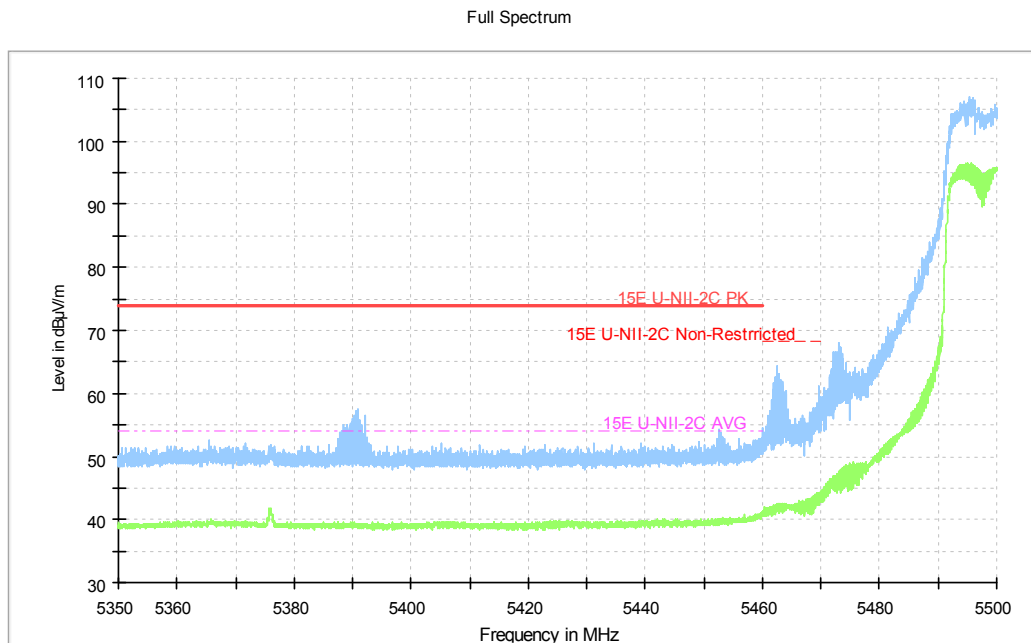
Fig.219 Band Edges (802.11ac-HT40, 5510MHz)
