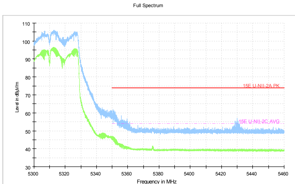
Fig.218 Band Edges (802.11ac-HT40, 5310MHz)
