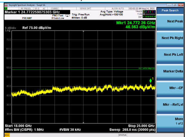
18-25 GHz, Vertical Antenna GFSK, Channel 39
