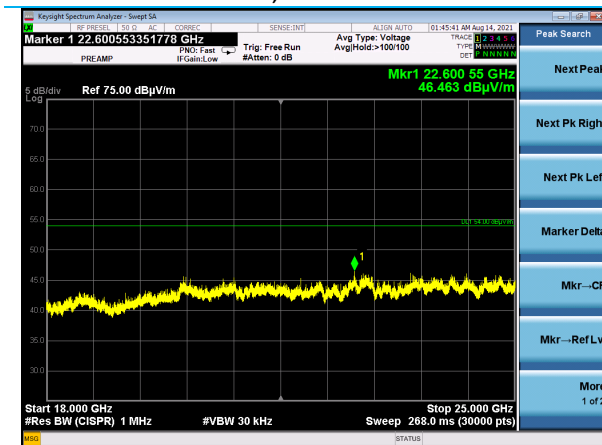
18-25 GHz, Horizontal Antenna GFSK, Channel 39
