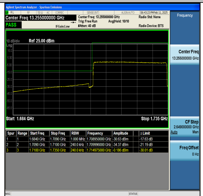
NTNV-n66-PC3-15-25-L-CP-QPSK-Outer_Full-PASS
