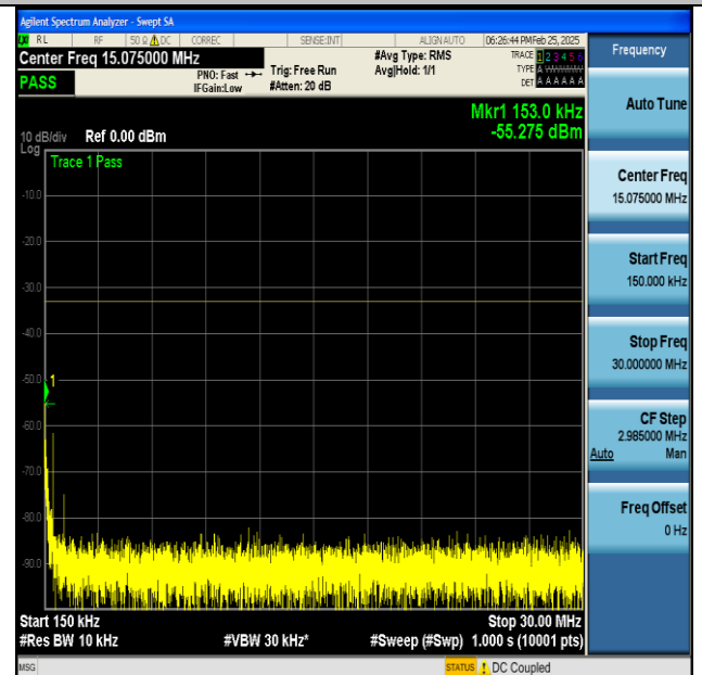
NTNV-n66-PC3-15-40-L-CP-QPSK-Edge_1RB_Left-0.15- 30-PASS
