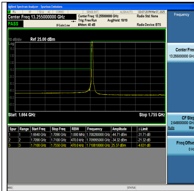
NTNV-n66-PC3-15-45-L-DFT-BPSK-Edge_1RB_Left-PASS
