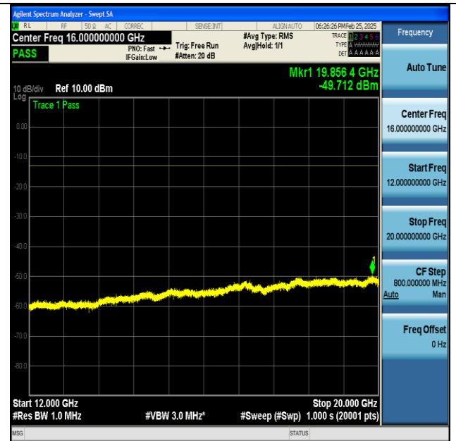
NTNV-n66-PC3-15-40-L-DFT-BPSK-Edge_1RB_Left- 12000-20000-PASS
