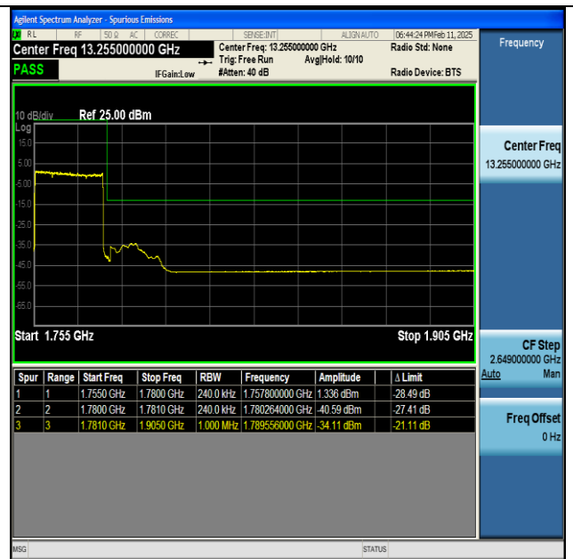
NTNV-n66-PC3-15-25-H-DFT-BPSK-Outer_Full-PASS
