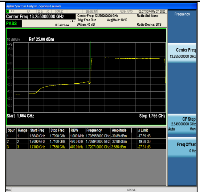
NTNV-n66-PC3-15-45-L-CP-QPSK-Outer_Full-PASS
