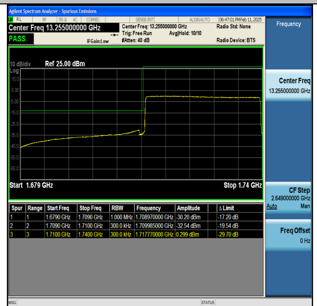
NTNV-n66-PC3-15-30-L-CP-QPSK-Outer_Full-PASS
