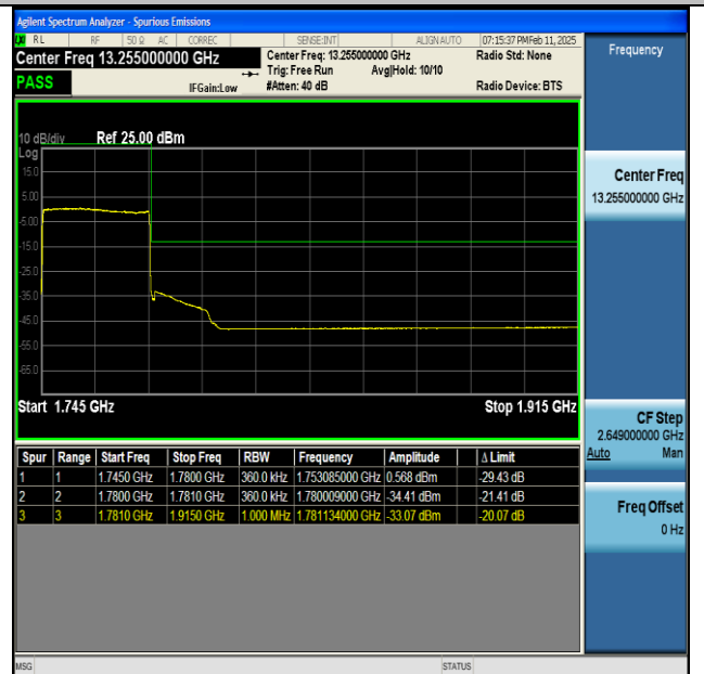
NTNV-n66-PC3-15-35-H-CP-QPSK-Outer_Full-PASS
