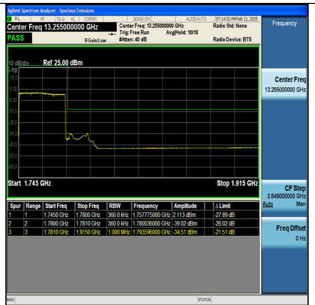
NTNV-n66-PC3-15-35-H-DFT-BPSK-Outer_Full-PASS
