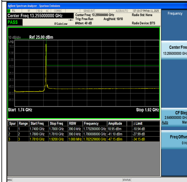
NTNV-n66-PC3-15-40-H-CP-QPSK-Edge_1RB_Right-PASS
