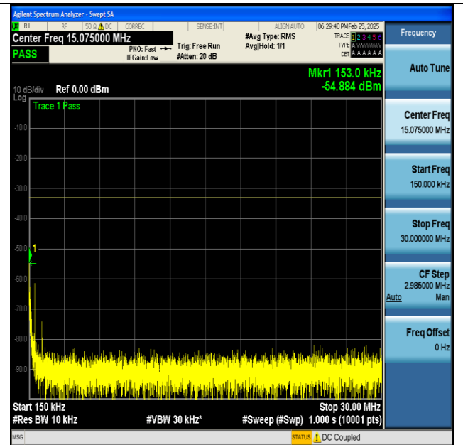
NTNV-n66-PC3-15-40-H-DFT-BPSK-Edge_1RB_Left-0.15- 30-PASS
