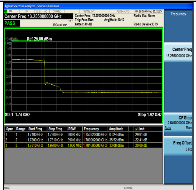
NTNV-n66-PC3-15-40-H-CP-QPSK-Outer_Full-PASS
