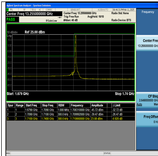
NTNV-n66-PC3-15-30-L-DFT-BPSK-Edge_1RB_Left-PASS
