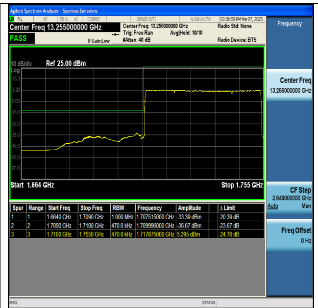
NTNV-n66-PC3-15-45-L-DFT-BPSK-Outer_Full-PASS
