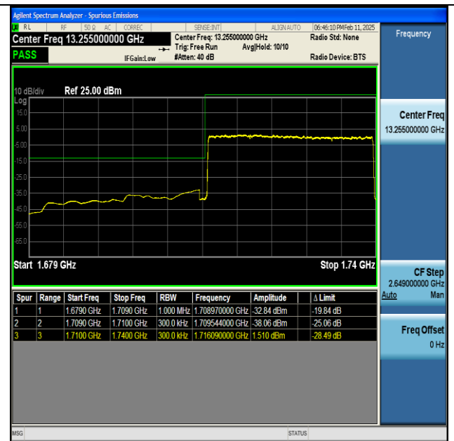
NTNV-n66-PC3-15-30-L-DFT-BPSK-Outer_Full-PASS
