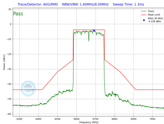
Plot 7-789. LPI In-Band Emission Plot Antenna WF7a (160MHz 802.11ax (UNII Band 7) – Ch. 143, MCS11)
