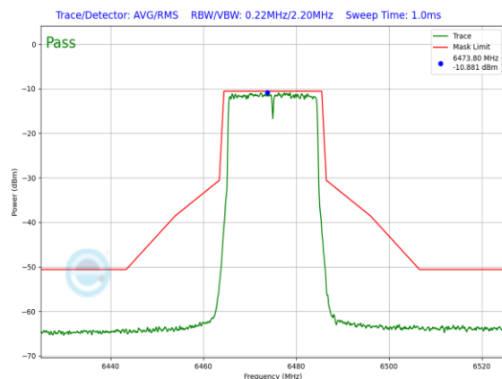
Plot 7-837. LPI In-Band Emission Plot Antenna WF2a (20MHz 802.11ax (UNII Band 6) – Ch. 105, MCS2)
