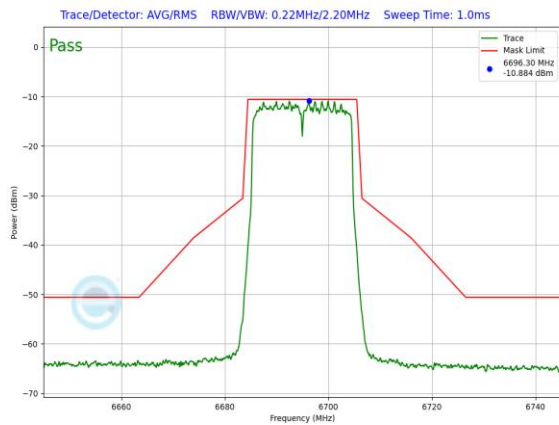
Plot 7-827. SP In-Band Emission Plot Antenna WF7a (20MHz 802.11ax (UNII Band 7) – Ch. 149, MCS11)
