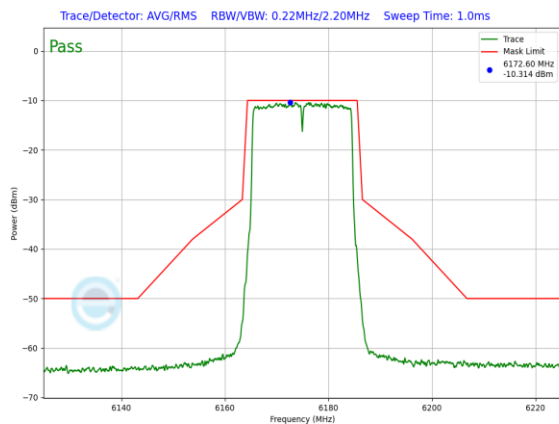
Plot 7-740. LPI In-Band Emission Plot Antenna WF7a (20MHz 802.11ax (UNII Band 5) – Ch. 45, MCS2)
