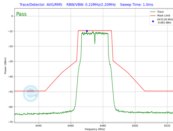
Plot 7-780. LPI In-Band Emission Plot Antenna WF7a (20MHz 802.11a (UNII Band 6) – Ch. 105, 54Mbps)
