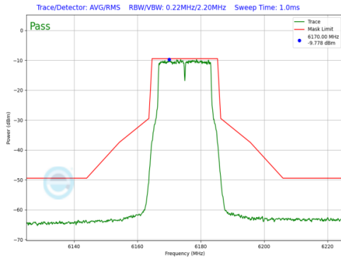
Plot 7-810. SP In-Band Emission Plot Antenna WF7a (20MHz 802.11a (UNII Band 5) – Ch. 45, 24Mbps)
