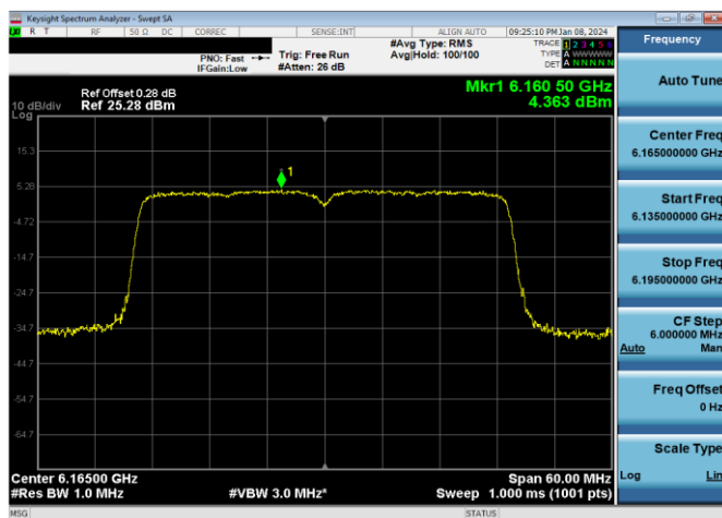
Plot 7-725. Power Spectral Density Plot CDD Diversity Antenna WF2a Standard Power (40MHz 802.11ax (UNII Band 5) – Ch. 43, MCS11)
