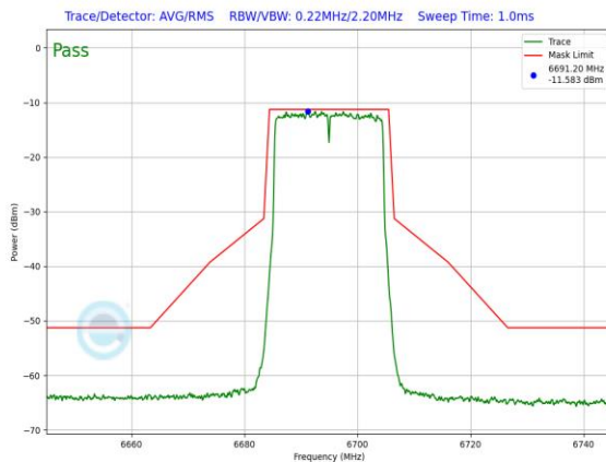
Plot 7-806. SP In-Band Emission Plot Antenna WF7a (20MHz 802.11ax (UNII Band 7) – Ch. 149, MCS2)
