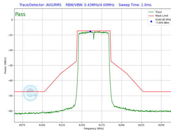
Plot 7-741. LPI In-Band Emission Plot Antenna WF7a (40MHz 802.11ax (UNII Band 5) – Ch. 43, MCS2)
