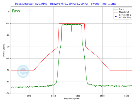
Plot 7-836. LPI In-Band Emission Plot Antenna WF2a (20MHz 802.11a (UNII Band 6) – Ch. 105, 12Mbps)
