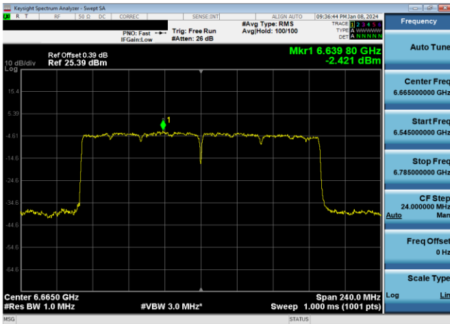
Plot 7-737. Power Spectral Density Plot CDD Diversity Antenna WF2a Standard Power (160MHz 802.11ax (UNII Band 7) – Ch. 143, MCS11)
