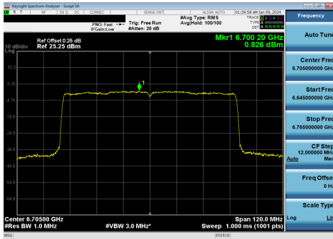
Plot 7-720. Power Spectral Density Plot CDD Diversity Antenna WF7b Standard Power (80MHz 802.11ax (UNII Band 7) – Ch. 151, MCS4)
