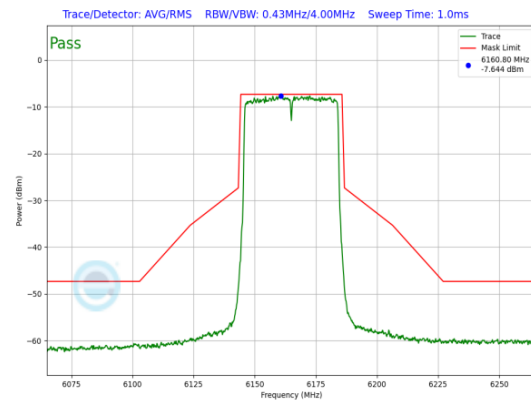
Plot 7-801. SP In-Band Emission Plot Antenna WF7a (40MHz 802.11ax (UNII Band 5) – Ch. 43, MCS2)
