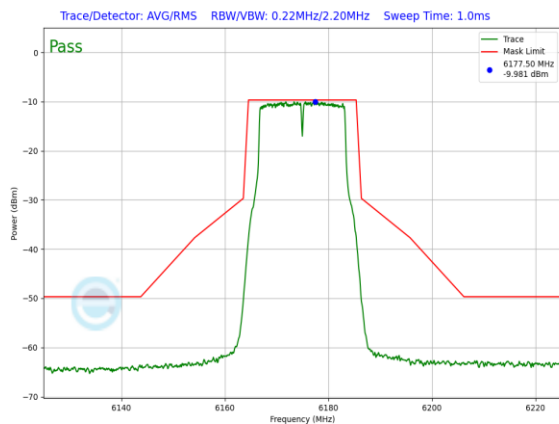
Plot 7-739. LPI In-Band Emission Plot Antenna WF7a (20MHz 802.11a (UNII Band 5) – Ch. 45, 12Mbps)
