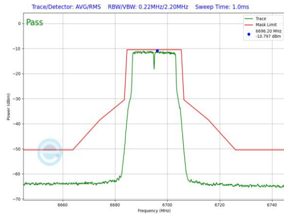
Plot 7-805. SP In-Band Emission Plot Antenna WF7a (20MHz 802.11a (UNII Band 7) – Ch. 149, 12Mbps)
