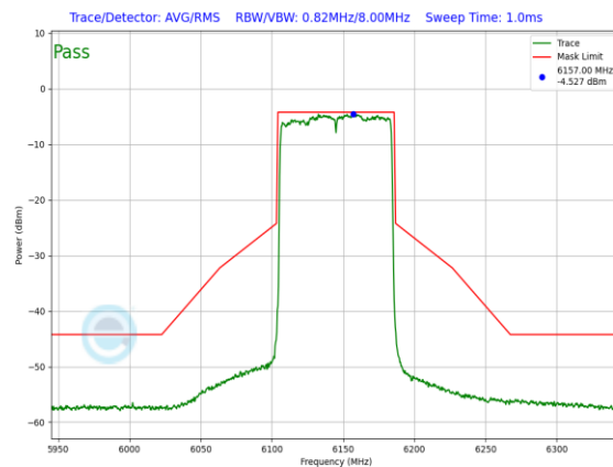
Plot 7-742. LPI In-Band Emission Plot Antenna WF7a (80MHz 802.11ax (UNII Band 5) – Ch. 39, MCS2)
