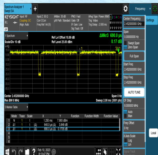
NTNV-11N40MIMO-Ant2-2452
