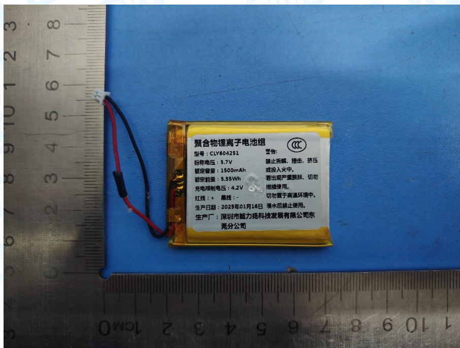
Photo 11 Battery Appearance
