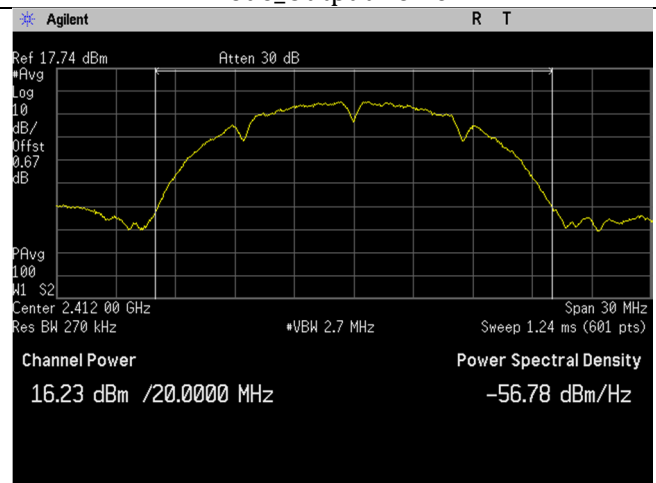
WIFI_Low Ch_2412MHz_20MHz BW_b-mode_Output Power
