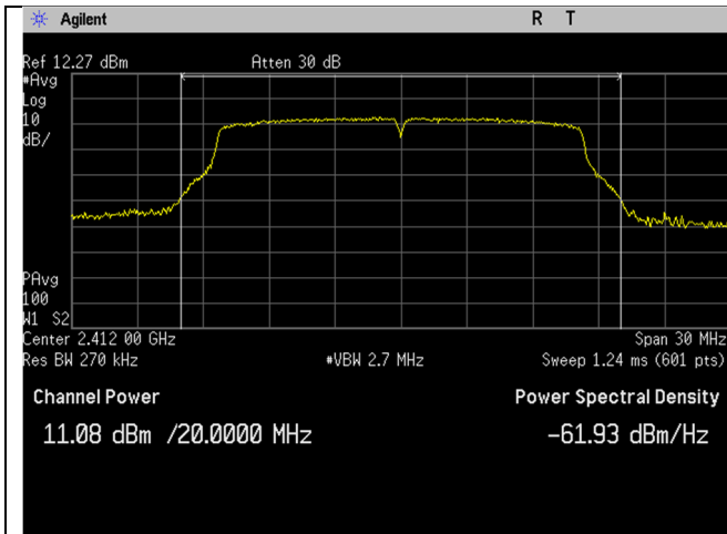
WIFI_Low Ch_2412MHz_20MHz BW_g-mode_Output Power
