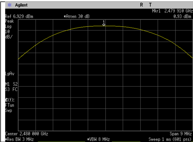
BLE_High Ch_2480MHz_1MBit_Output Power
