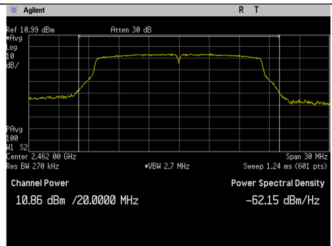
WIFI_High Ch_2462MHz_20MHz BW_g-mode_Output Power
