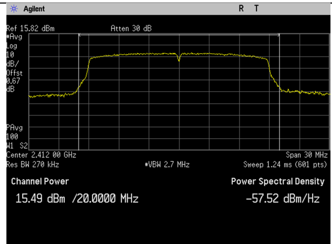
WIFI_Low Ch_2412MHz_20MHz BW_n-mode_Output Power
