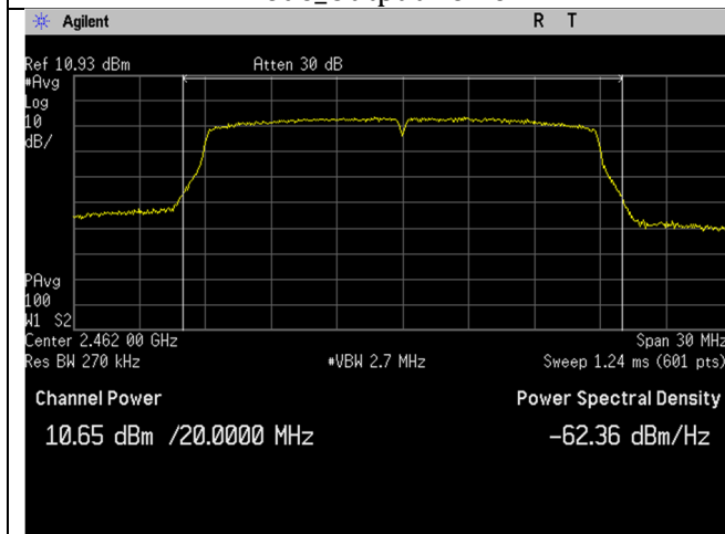
WIFI_High Ch_2462MHz_20MHz BW_n-mode_Output Power
