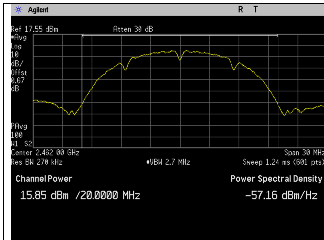
WIFI_High Ch_2462MHz_20MHz BW_b-mode_Output Power
