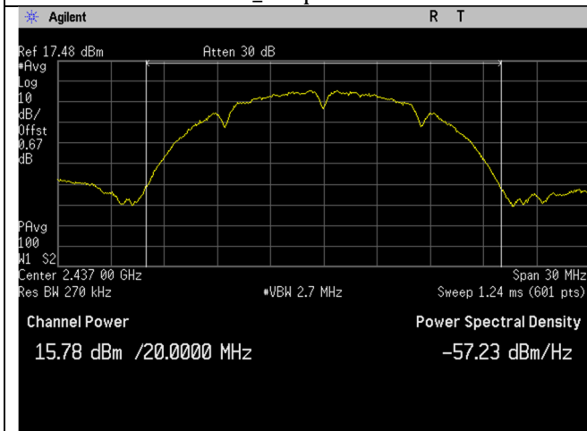
WIFI_Mid Ch_2437MHz_20MHz BW_b-mode_Output Power
