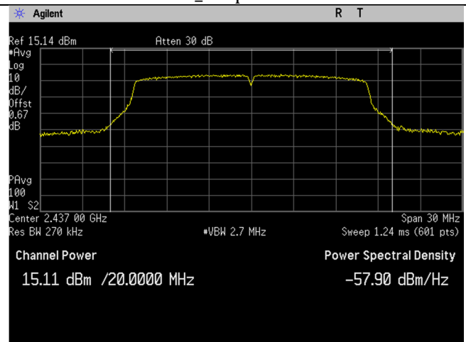
WIFI_Mid Ch_2437MHz_20MHz BW_g-mode_Output Power
