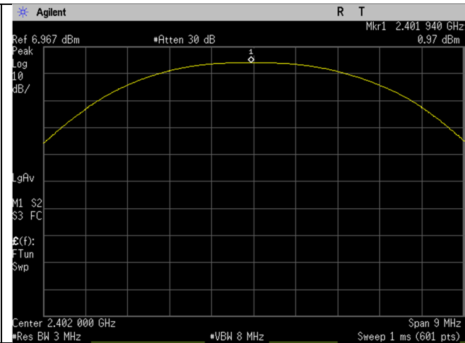
BLE_Low Ch_2402MHz_1MBit_Output Power
