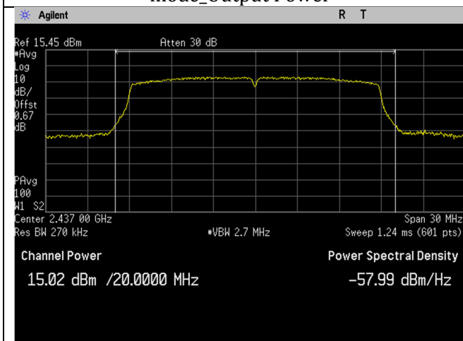
WIFI_Mid Ch_2437MHz_20MHz BW_n-mode_Output Power
