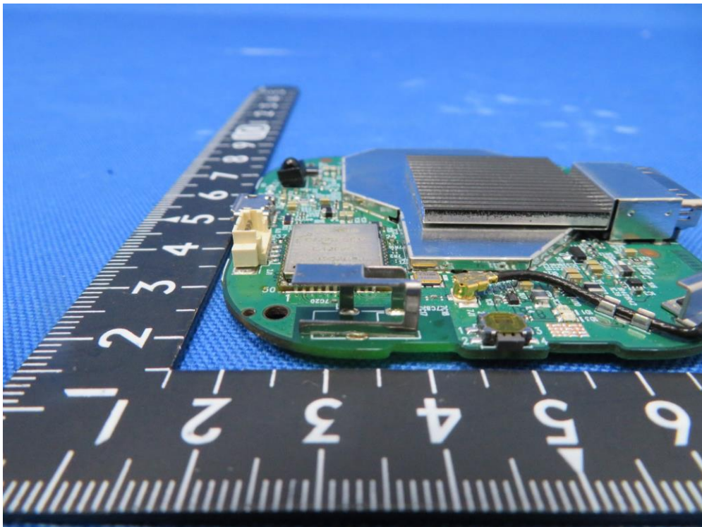
(6) Antenna Photo
