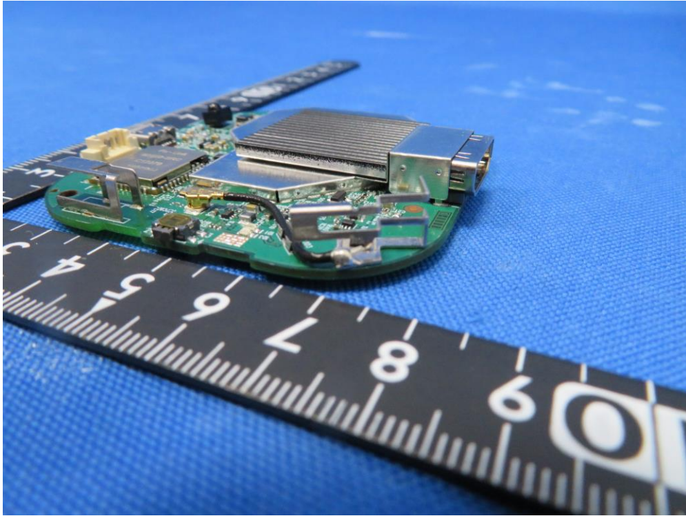
(5) Antenna Photo
