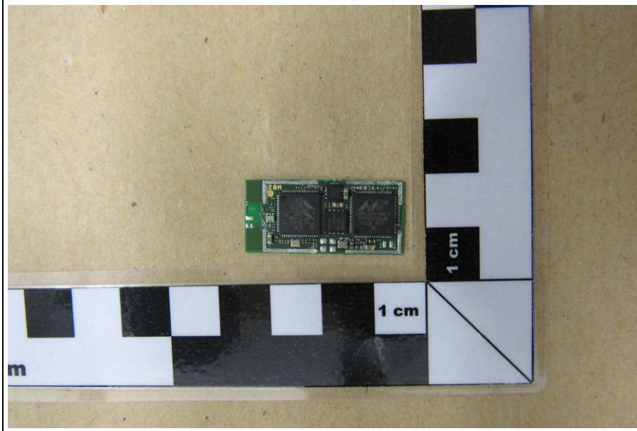
ENW49A01C3EF MODULE TOP WITHOUT SHIELDING
