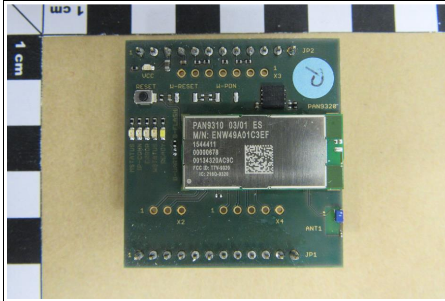
ENW49A01C3EF REFERENCE DESIGN TOP
