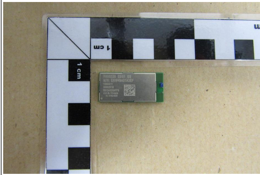
ENW49A01A3EF MODULE TOP WITH SHIELDING
