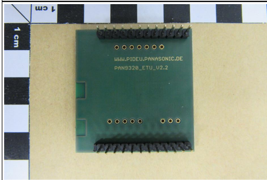
ENW49A01C3EF REFERENCE DESIGN BOTTOM
