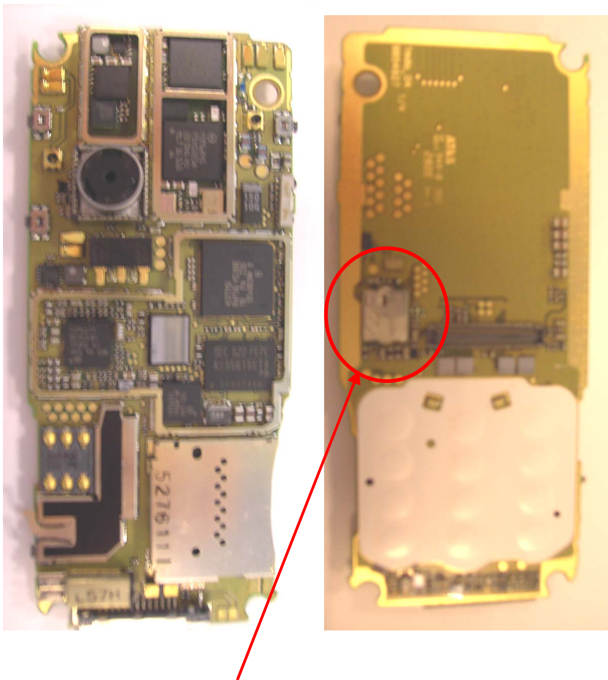
BT Antenna
