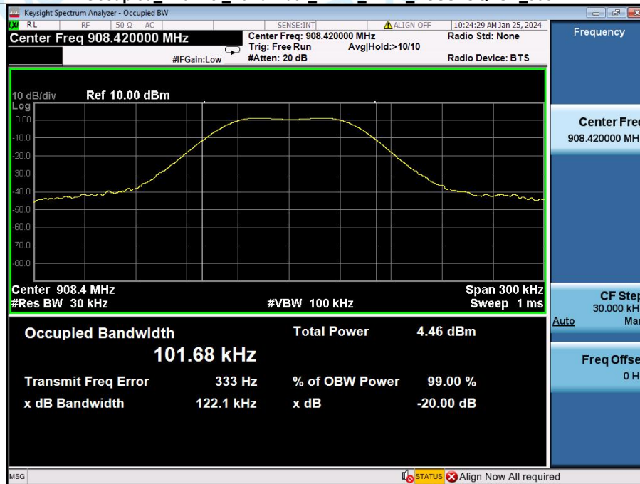
Occupied_Channel_Bandwidth_NVNT_ANT1_DSSS/OQPSK_908.42
