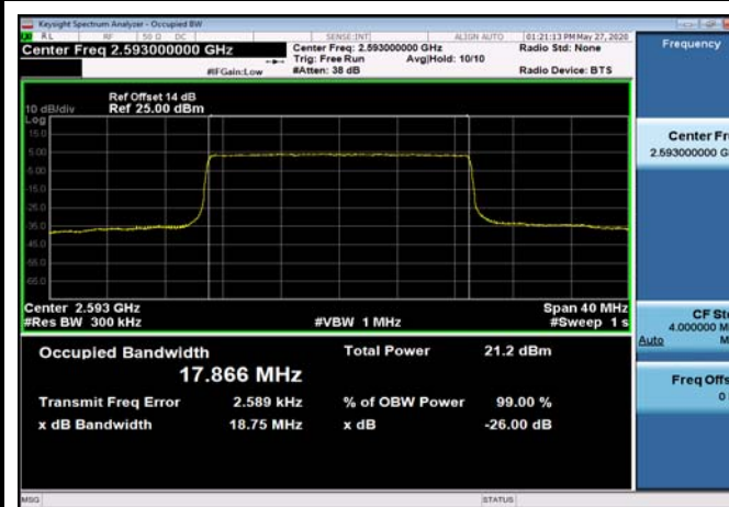
TDD41_MidRange_20_2593_QPSK
