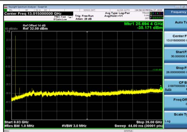
FDD12_HighRange_1.4MHz_30MHz~26GHz
