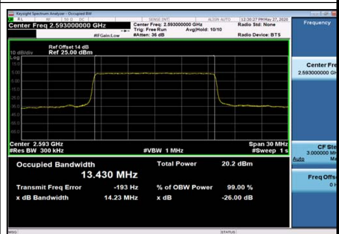
TDD41_MidRange_15MHz_2593MHz_Q16
