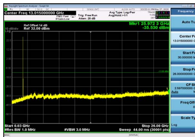
FDD02_MidRange_20MHz_30MHz~26GHz
