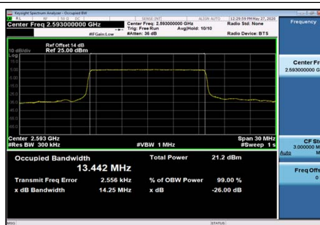
TDD41_MidRange_15MHz_2593MHz_QPSK
