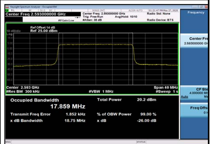
TDD41_MidRange_20_2593_Q16
