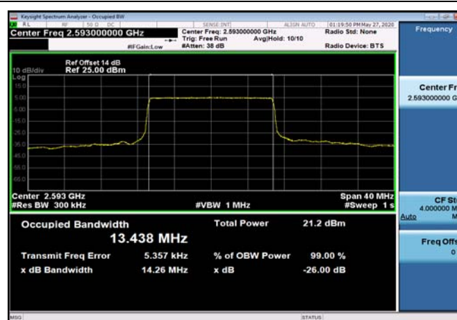
TDD41_MidRange_15_2593_QPSK
