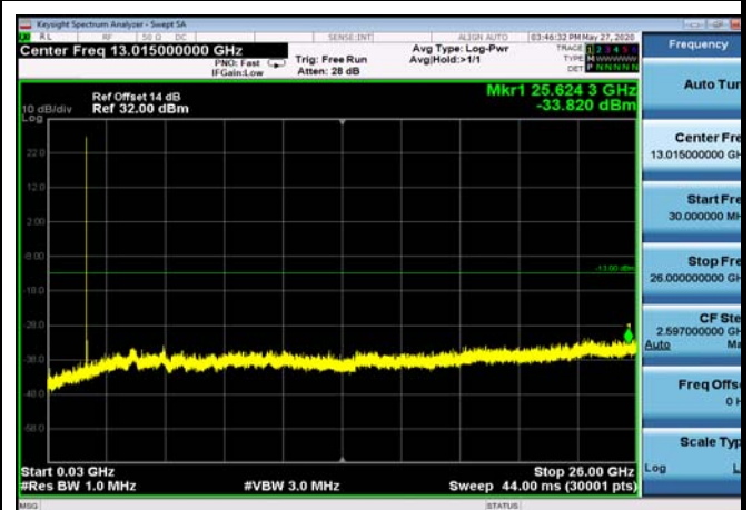
FDD04_HighRange_15MHz_30MHz~26GHz
