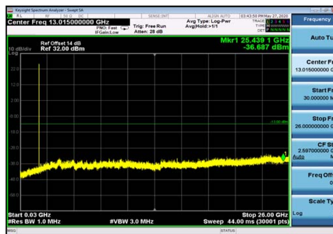
FDD02_LowRange_5MHz_30MHz~26GHz
