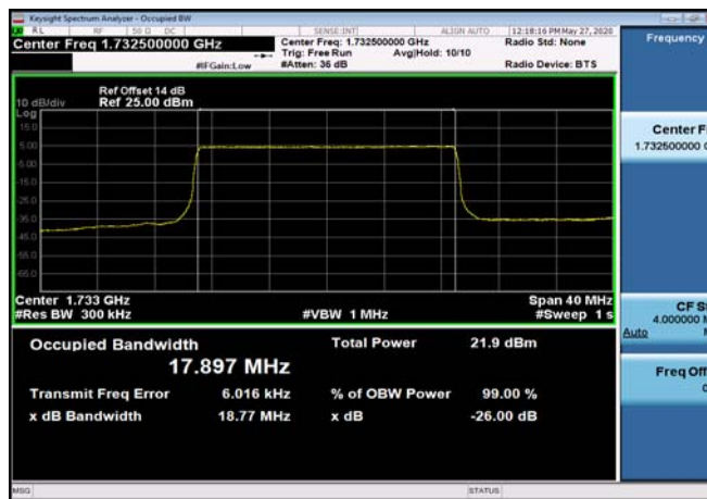
FDD04_MidRange_20MHz_1732.5MHz _QPSK
