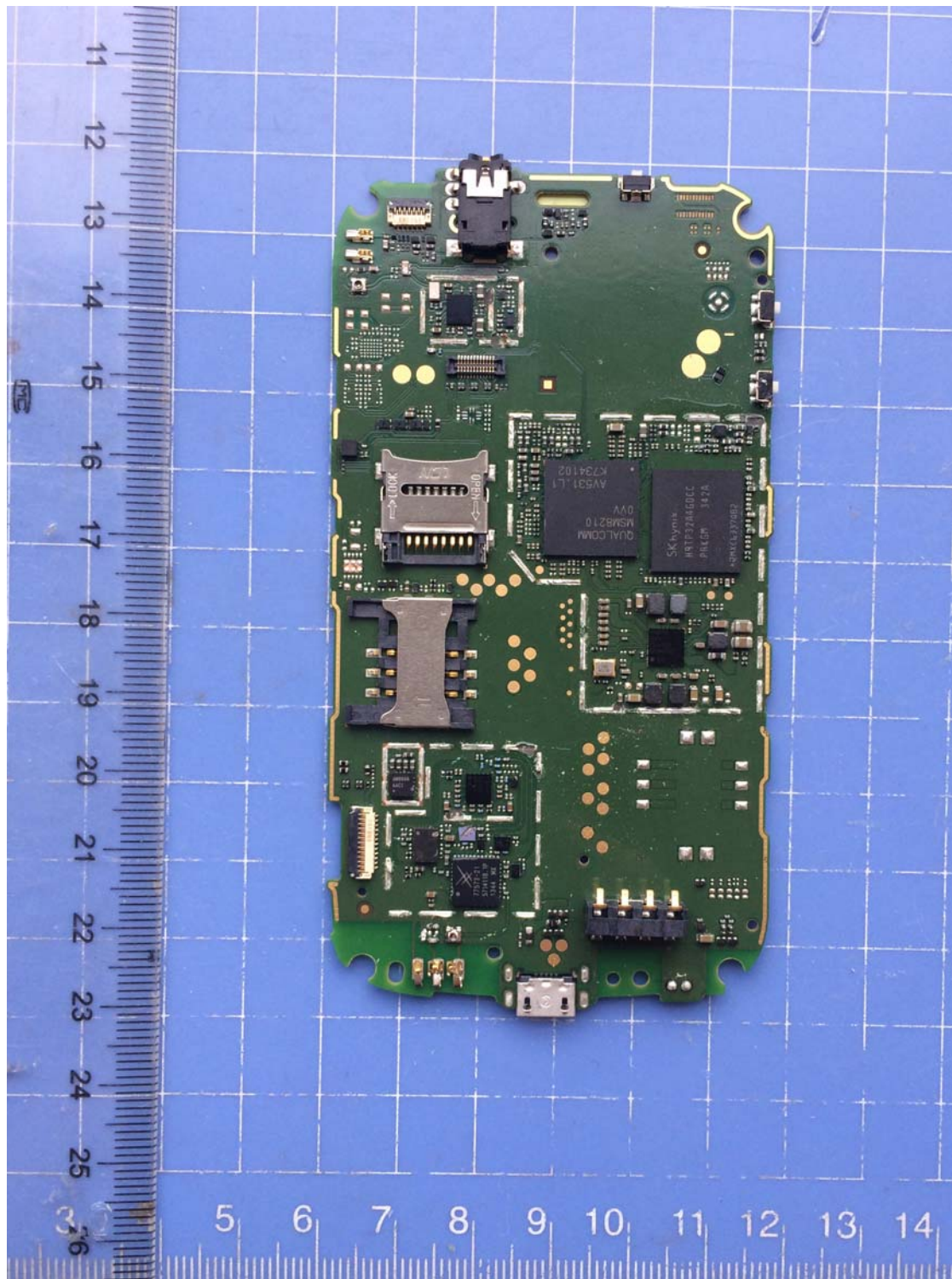
Pic A-5 Mobile phone Disassembly
