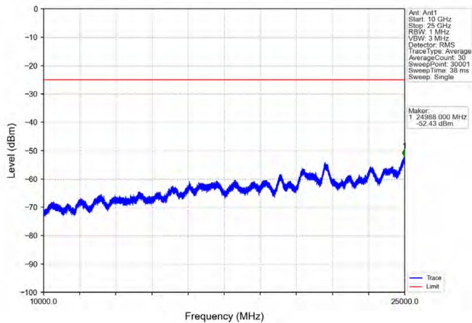
Band7_5MHz_16QAM_LCH_2502.5MHz_RB_1_0_NTV
