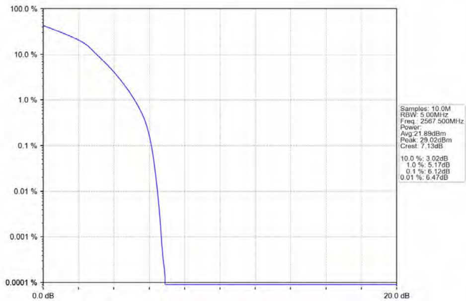
Band7_5MHz_16QAM_HCH_2567.5MHz_RB_25_0_NTV
