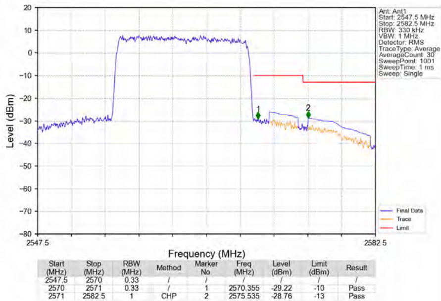
Band7_15MHz_16QAM_HCH_2562.5MHz_RB_75_0_NTNV
