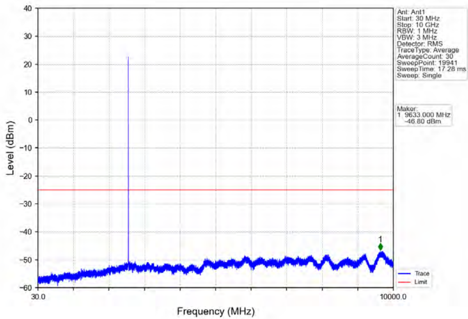
Band7_5MHz_64QAM_HCH_2567.5MHz_RB_1_0_NTNV
