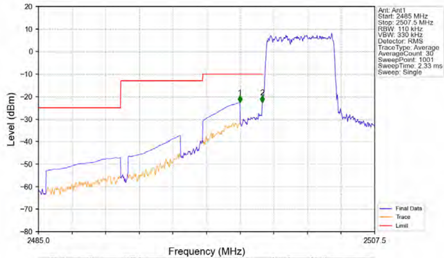
Band7_5MHz_16QAM_LCH_2502.5MHz_RB_25_0_NTV
