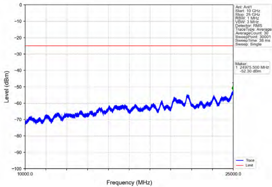
Band7_15MHz_64QAM_MCH_2535MHz_RB_1_0_NTNV
