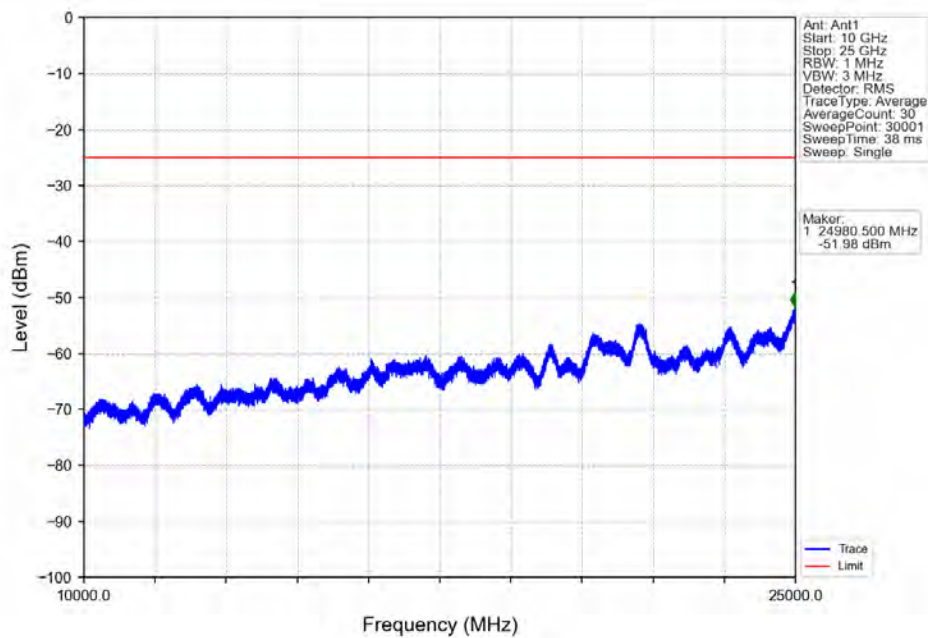
Band7_5MHz_16QAM_MCH_2535MHz_RB_1_0_NTN
