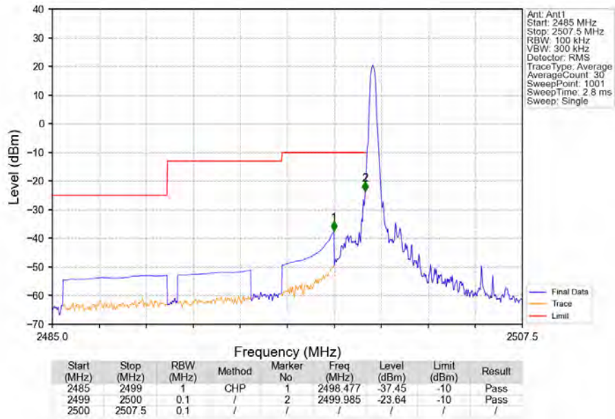
Band7 5MHz 64QAM LCH 2502.5MHz RB 1 0 NTNV
