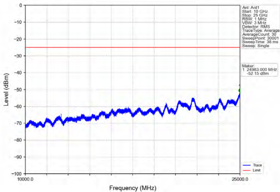
Band7_15MHz_16QAM_LCH_2507.5MHz_RB_1_0_NTNV
