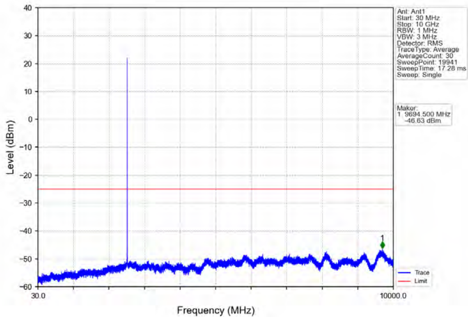
Band7_5MHz_64QAM_MCH_2535MHz_RB_1_0 NTN
