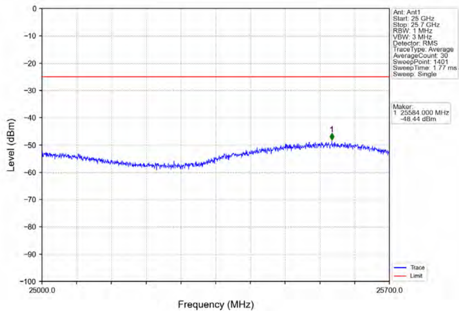
Band7_5MHz_64QAM_MCH_2535MHz_RB_1_0_NTNV
