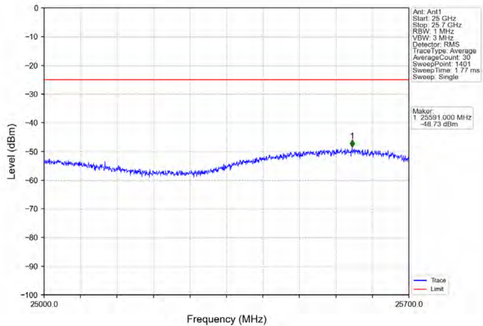
Band7_10MHz_64QAM_LCH_2505MHz_RB_1_0_NTNV
