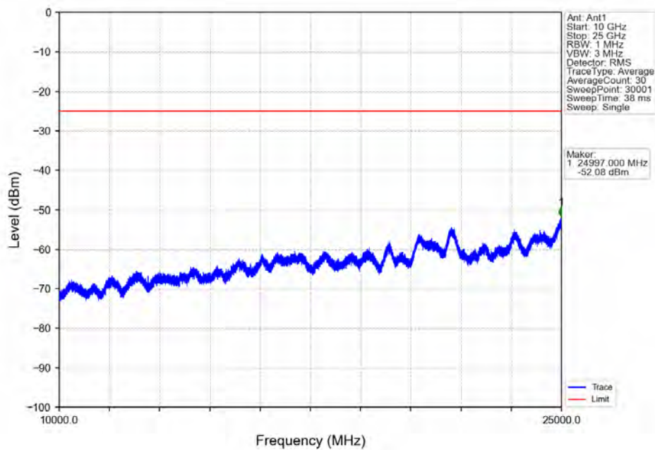
Band7_10MHz_16QAM_MCH_2535MHz_RB_1_0_NTNV
