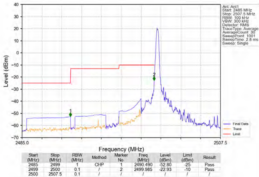
Band7_5MHz_16QAM_LCH_2502.5MHz_RB_1_0_NTV
