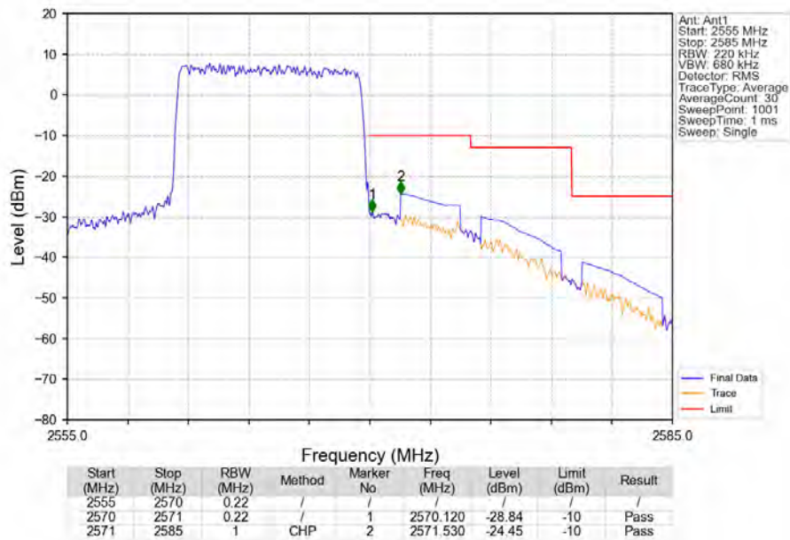
Band7_10MHz_16QAM_HCH_2565MHz_RB_50_0_NTNV
