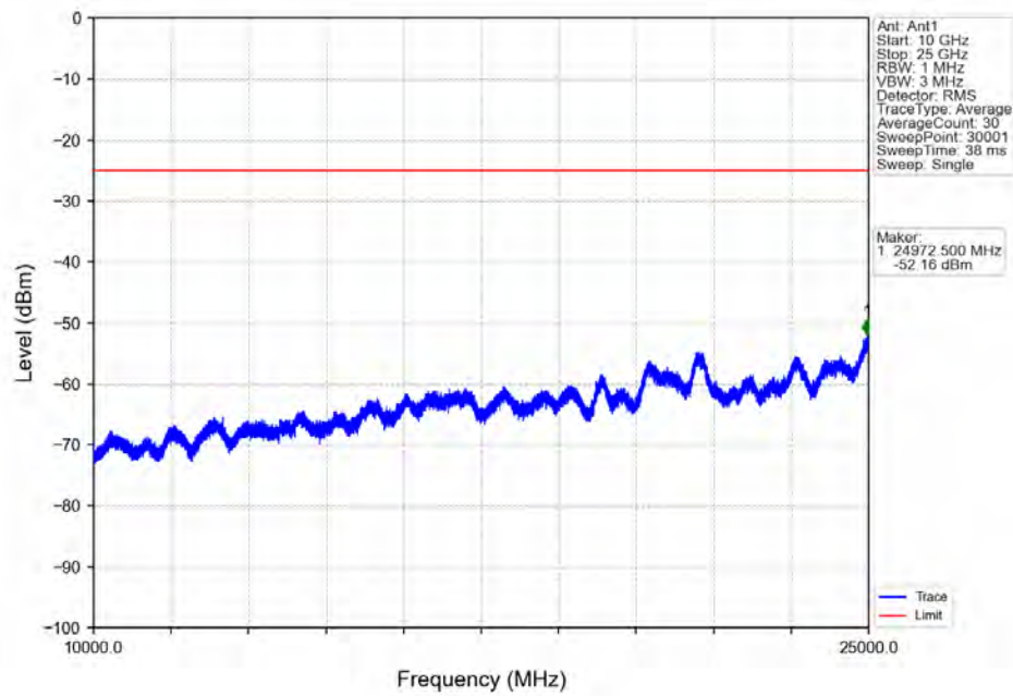
Band7_15MHz_64QAM_LCH_2507.5MHz_RB_1_0_NTNV
