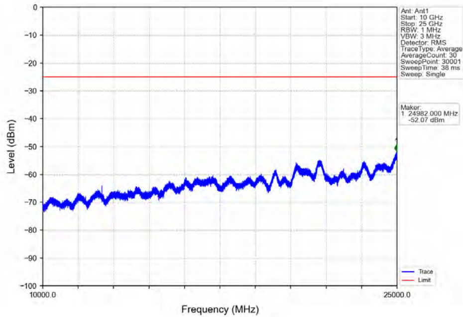
Band7_15MHz_QPSK_LCH_2507.5MHz_RB_1_0_NTV
