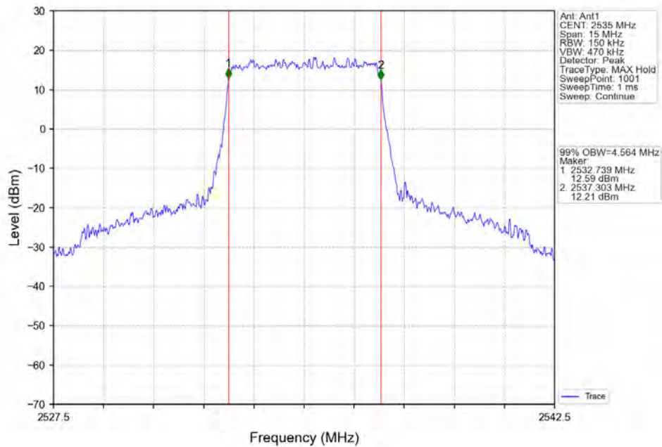
Band7_5MHz_64QAM_MCH_2535MHz_RB_25_0_NTV
