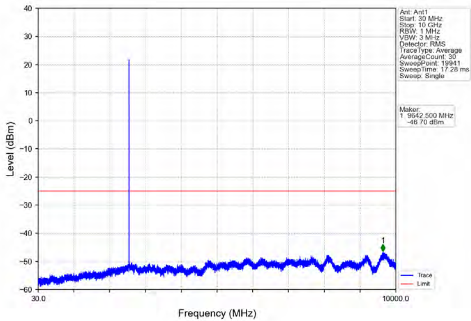
Band7_10MHz_64QAM_HCH_2565MHz_RB_1_0_NTNV
