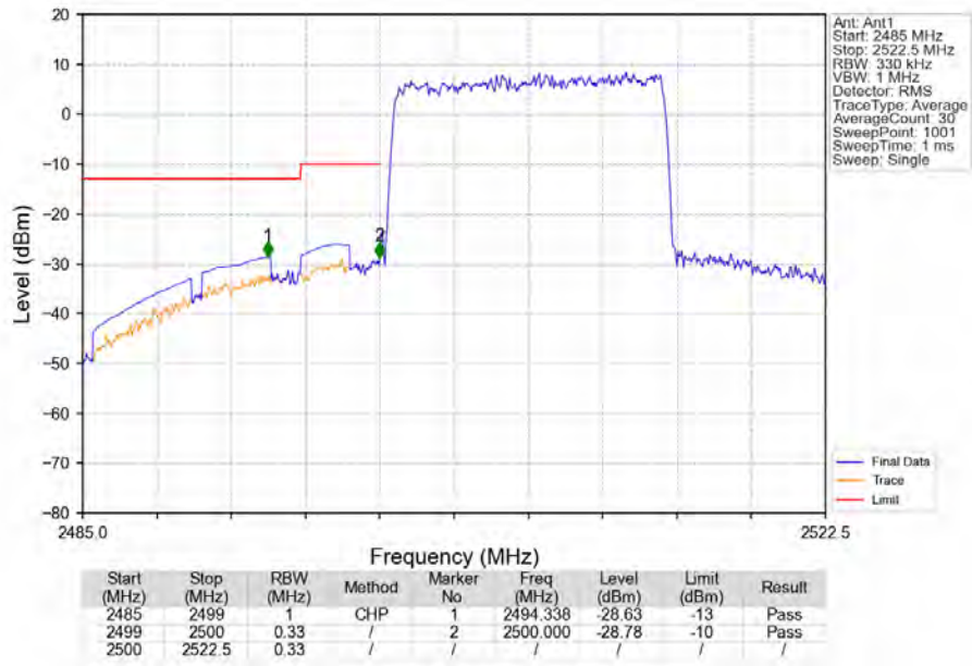
Band7 15MHz 64QAM LCH 2507.5MHz RB 75 0 NTNV
