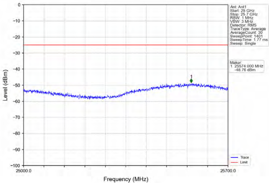
Band7_5MHz_64QAM_HCH_2567.5MHz_RB_1_24_NTV
