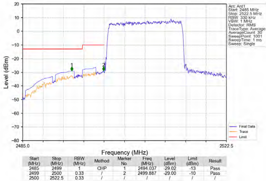
Band7_15MHz_16QAM_LCH_2507.5MHz_RB_75_0_NTNV
