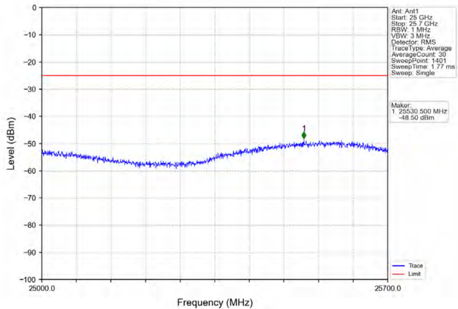
Band7_15MHz_QPSK_LCH_2507.5MHz_RB_1_0_NTV
