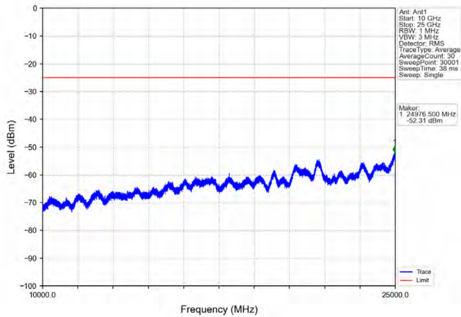
Band7_5MHz_64QAM_MCH_2535MHz_RB_1_0_NTNV
