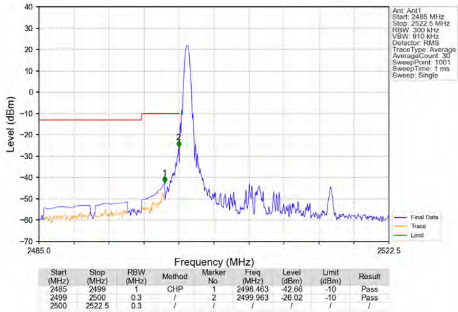
Band7_15MHz_64QAM_LCH_2507.5MHz_RB_1_0_NTNV
