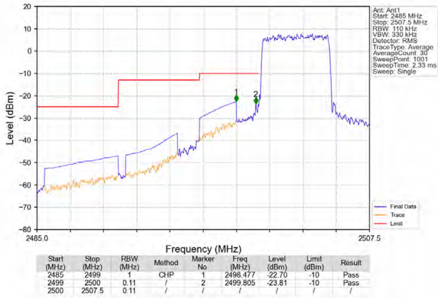
Band7 5MHz 64QAM LCH 2502.5MHz RB 25 0 NTN
