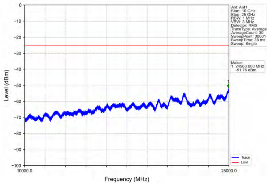
Band7_15MHz_QPSK_HCH_2562.5MHz_RB_1_0_NTV
