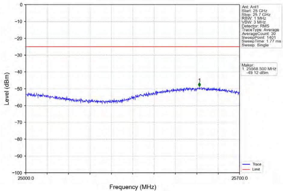
Band7_10MHz_64QAM_MCH_2535MHz_RB_1_0_NTNV
