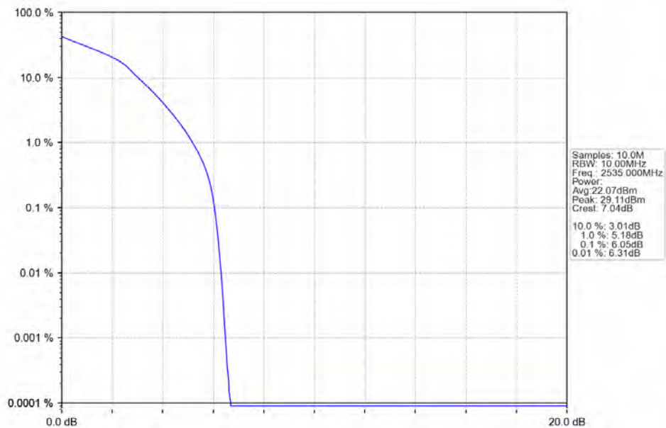
Band7_10MHz_64QAM_MCH_2535MHz_RB_50_0_NTV
