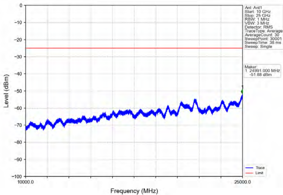
Band7_15MHz_64QAM_HCH_2562.5MHz_RB_1_0_NTNV
