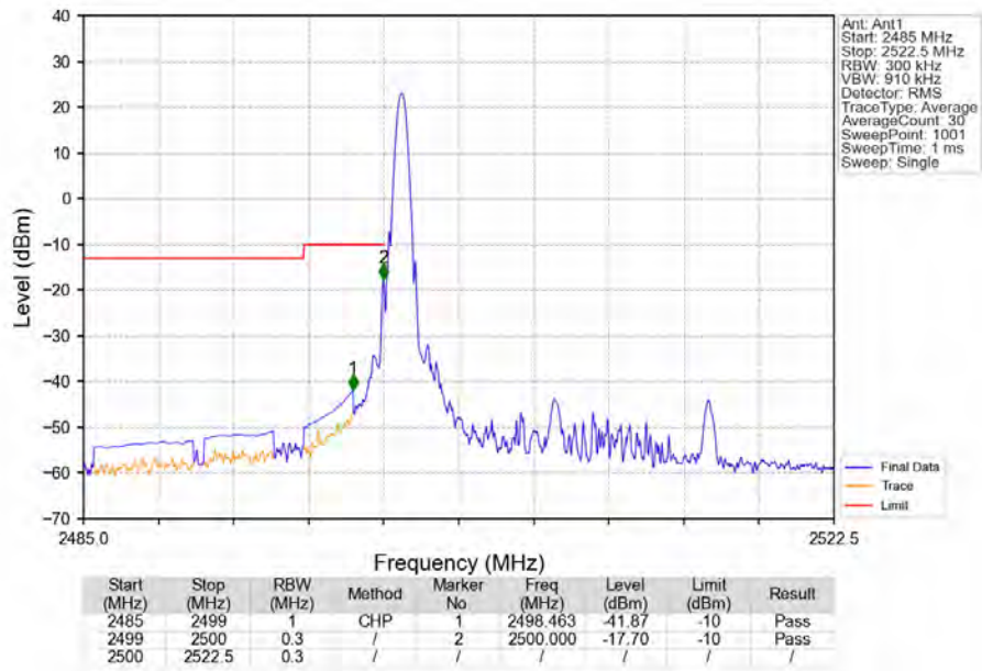
Band7_15MHz_QPSK_LCH_2507.5MHz_RB_1_0_NTNV
