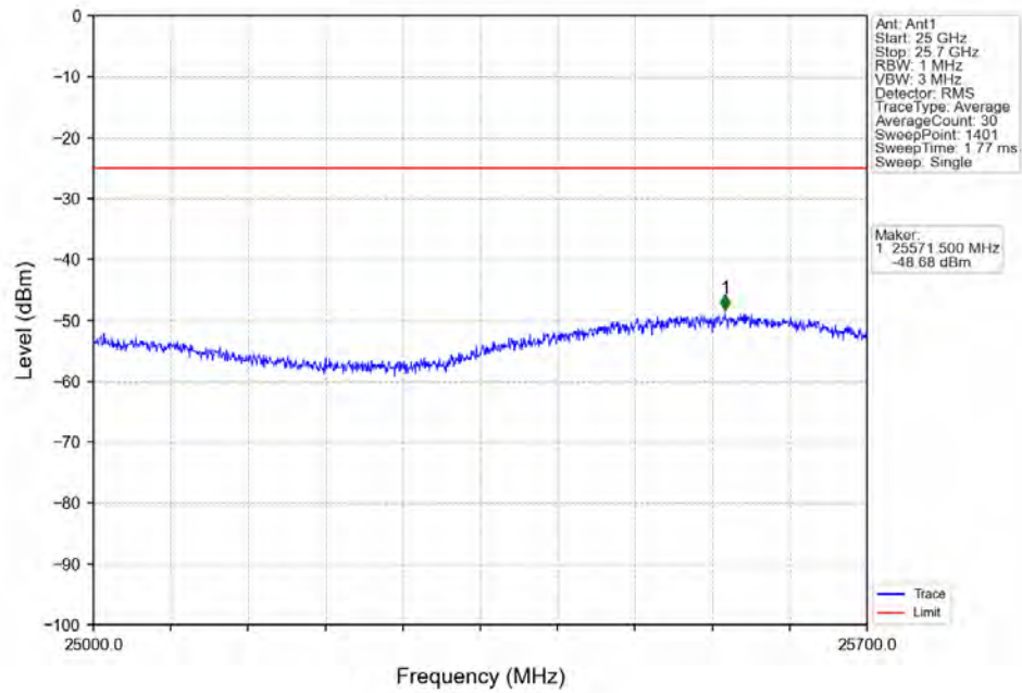
Band7_5MHz_16QAM_LCH_2502.5MHz_RB_25_0_NTV
