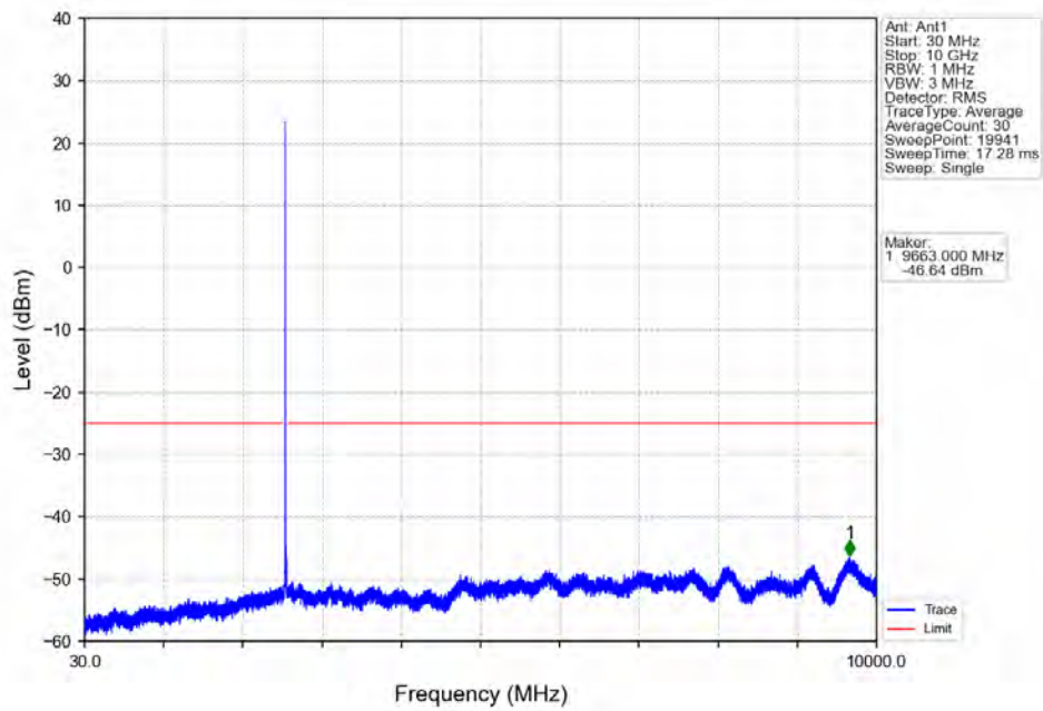
Band7_15MHz_QPSK_HCH_2562.5MHz_RB_1_0_NTV
