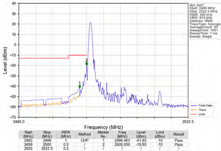
Band7_15MHz_16QAM_LCH_2507.5MHz_RB_1_0_NTNV
