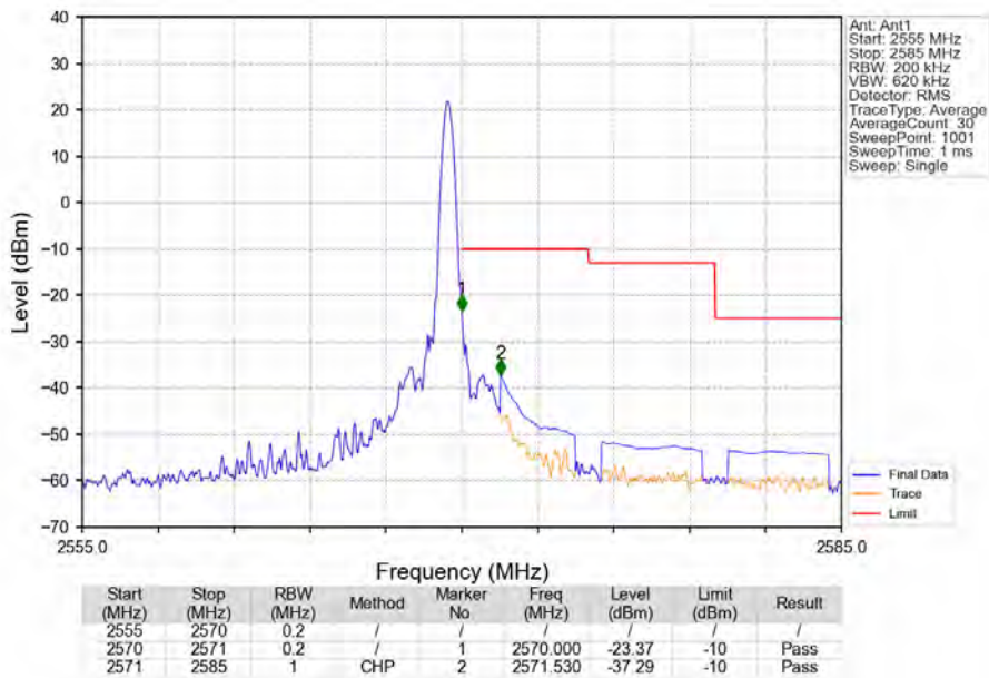
Band7_10MHz_64QAM_HCH_2565MHz_RB_1_49_NTV
