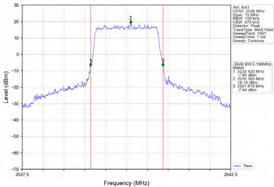
Band7_5MHz_64QAM_MCH_2535MHz_RB_25_0_NTV
