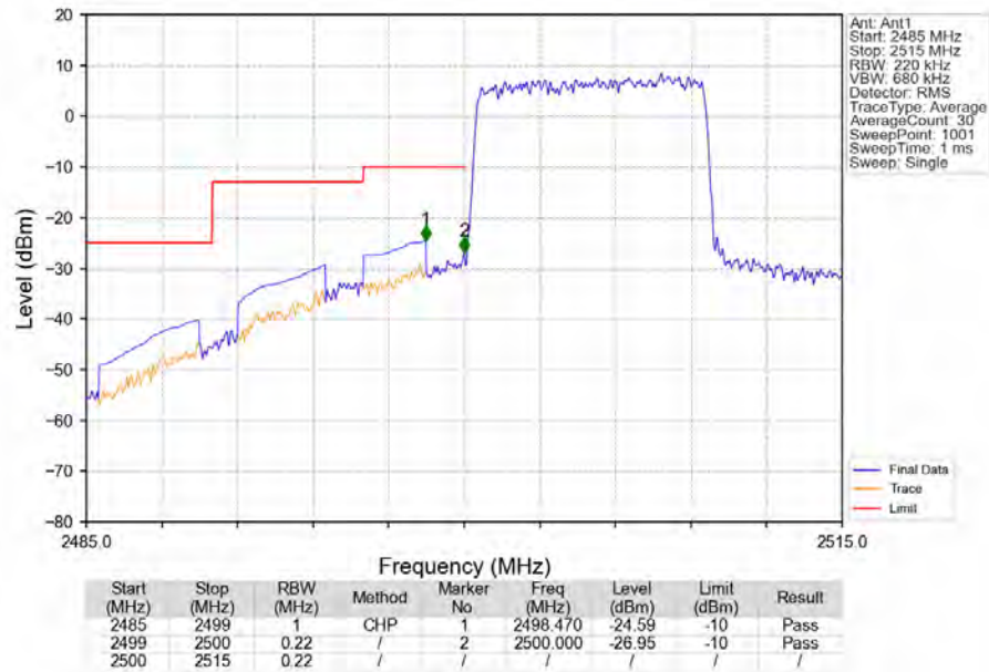
Band7_10MHz_16QAM_LCH_2505MHz_RB_50_0_NTV
