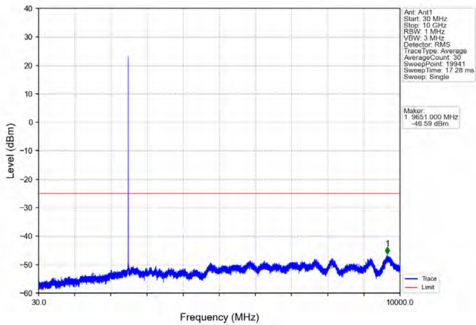
Band7_5MHz_16QAM_LCH_2502.5MHz_RB_1_0_NTV
