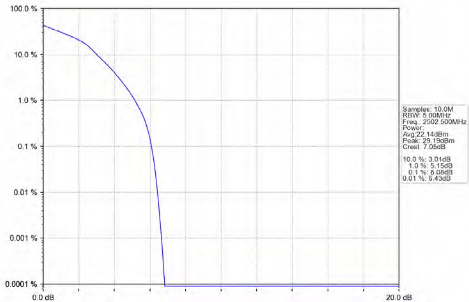
Band7_5MHz_16QAM_LCH_2502.5MHz_RB_25_0_NTV
