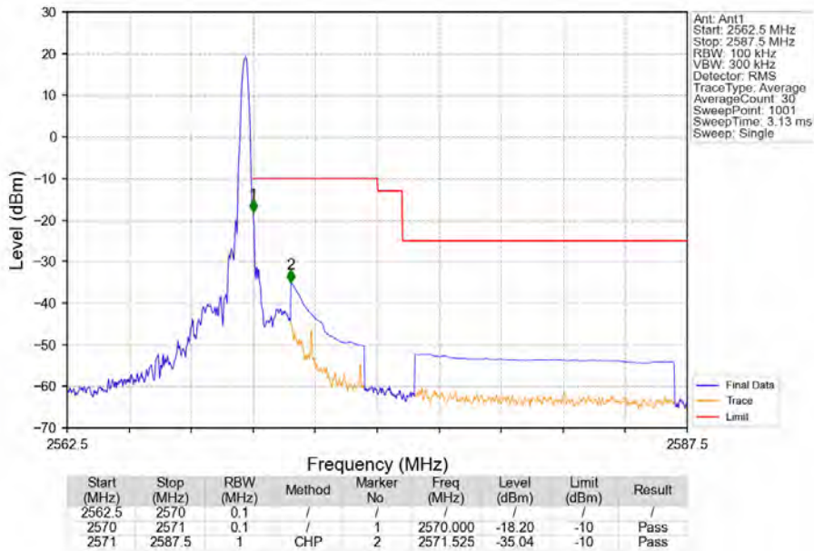
Band7_5MHz_64QAM_HCH_2567.5MHz_RB_1_24_NTV
