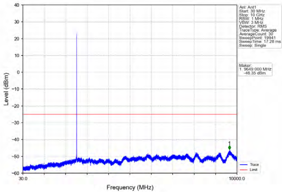
Band7_5MHz_16QAM_MCH_2535MHz_RB_1_0_NTN
