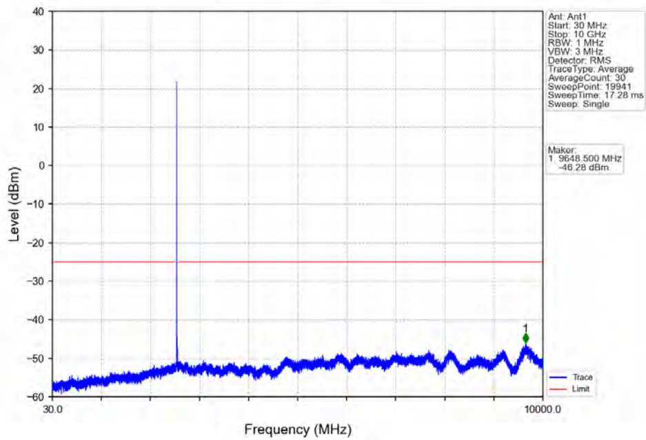
Band7_15MHz_64QAM_HCH_2562.5MHz_RB_1_0_NTNV
