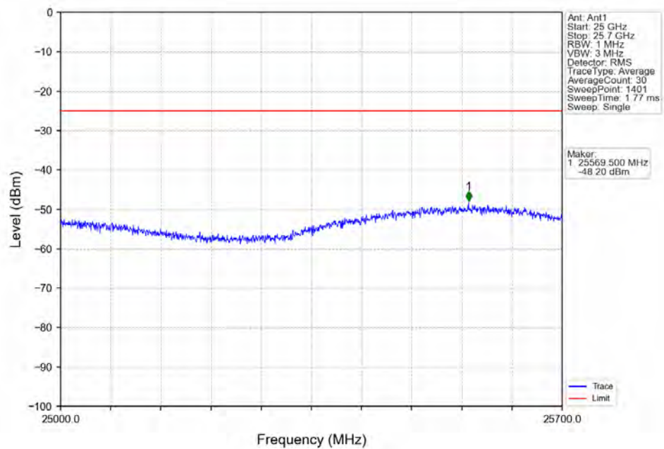
Band7_10MHz_16QAM_HCH_2565MHz_RB_1_0_NTNV
