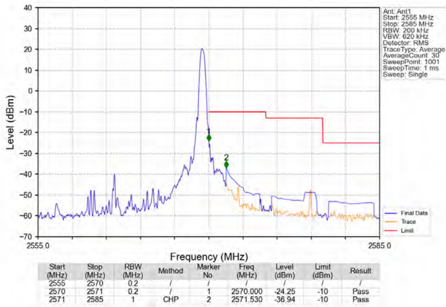
Band7_10MHz_16QAM_HCH_2565MHz_RB_1_49_NTNV
