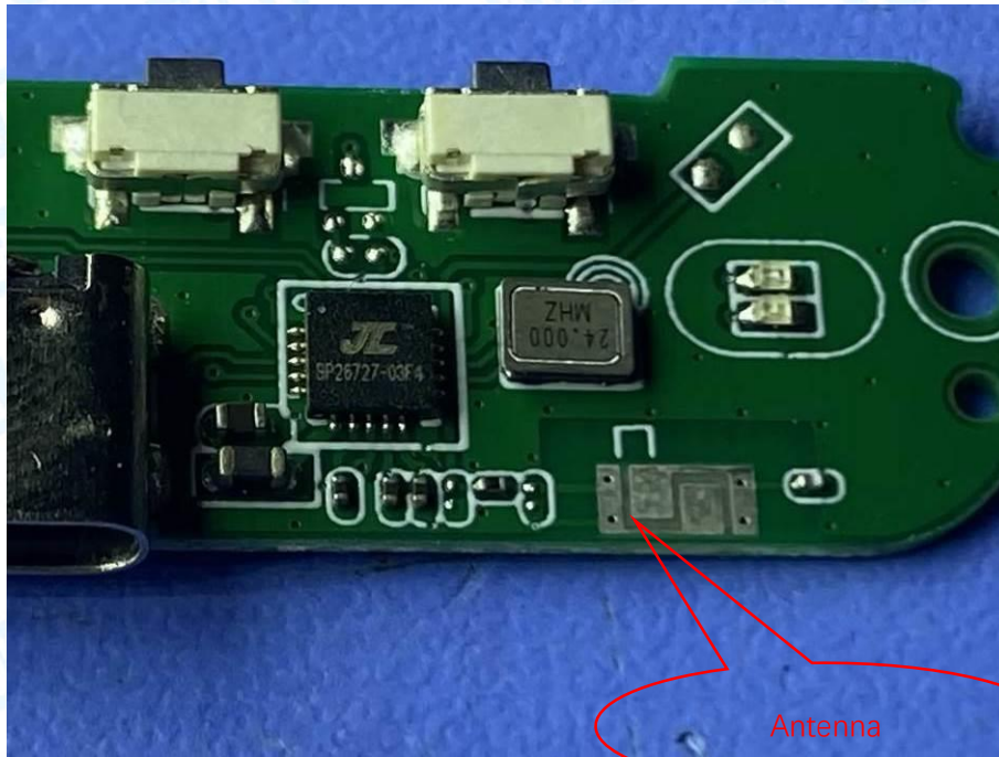
Photo 15 Internal of PCB
