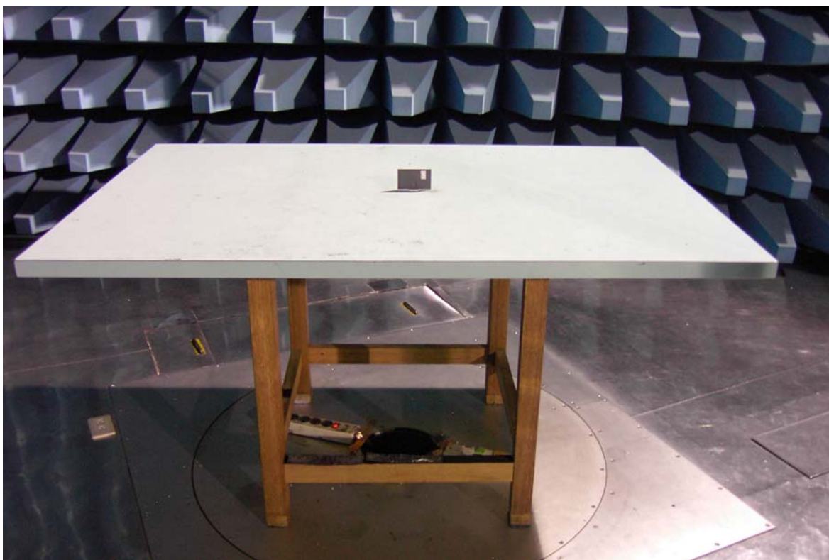
Front View of the Test Configuration
