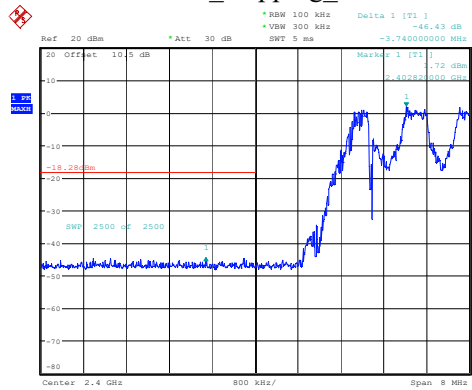
DH1_Hopping_Lower
