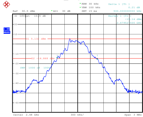
DH1_High 0.930MHz
