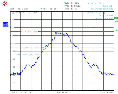
DH1_Middle 0.934MHz
