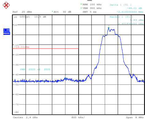
2DH1_Low
