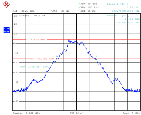
DH1_Low 0.934MHz
