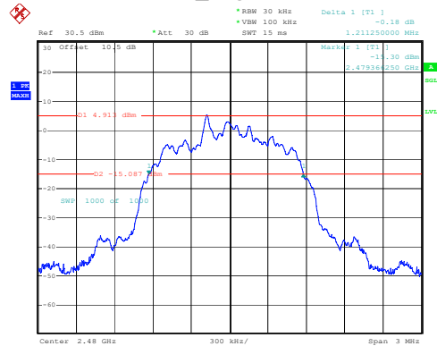
2DH1_High 1.211MHz
