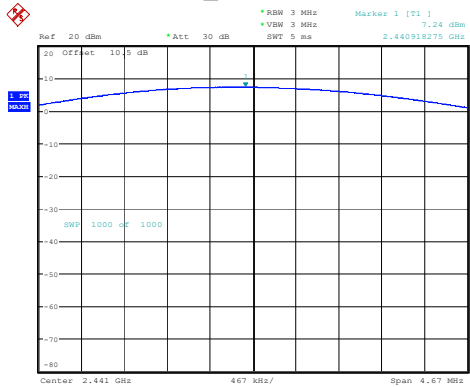
DH1_Middle 7.24dBm
