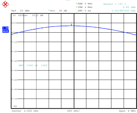
2DH1_Low 6.85dBm
