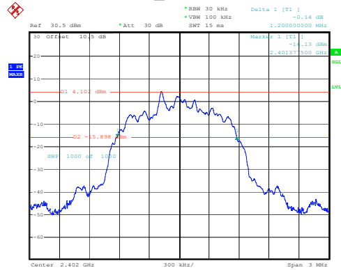
2DH1_Low 1.200MHz
