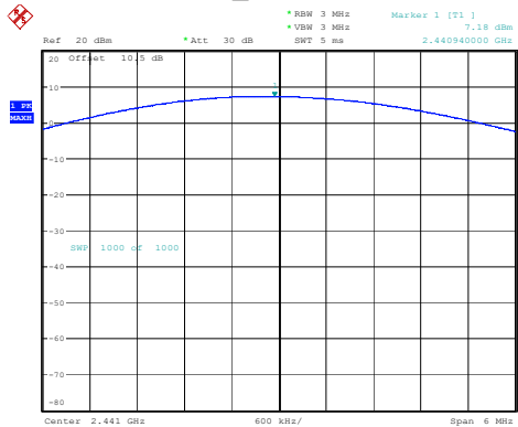
2DH1_Middle 7.18dBm
