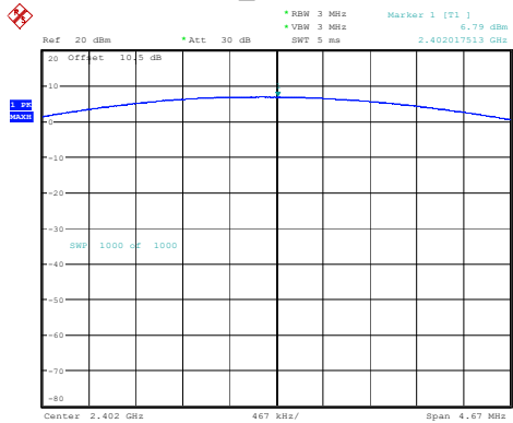
DH1_Low 6.79dBm
