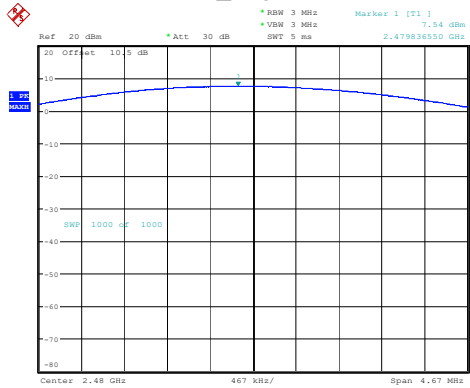
DH1_High 7.54dBm
