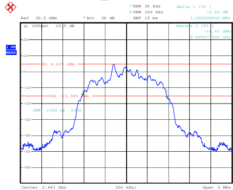
2DH1_Middle 1.200MHz
