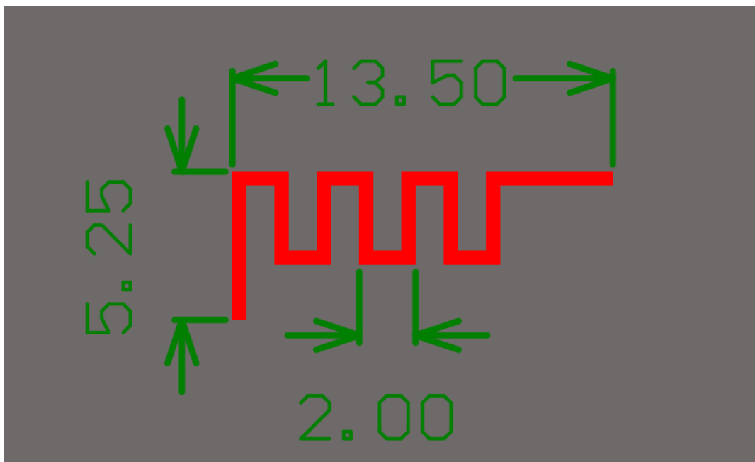
Antenna Dimension for Find My Locator Card
