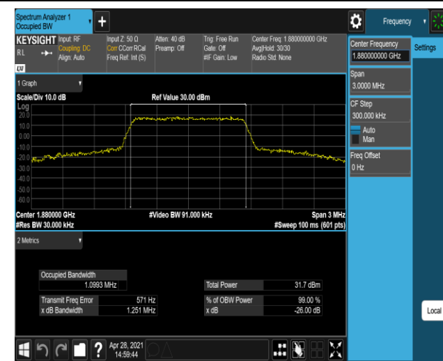
Band2-1.4MHz-16QAM-18900-6RB#0
