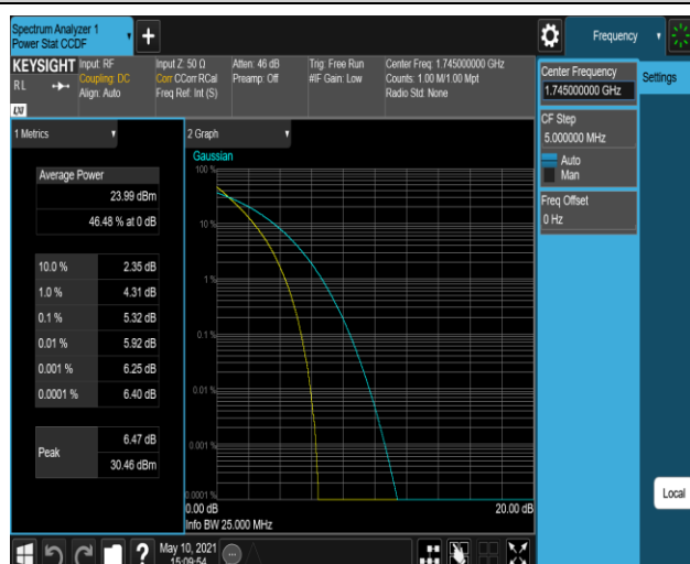
Band66-20MHz-QPSK-132322-100RB#0
