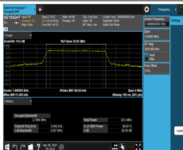
Band2-3MHz-16QAM-19185-15RB#0
