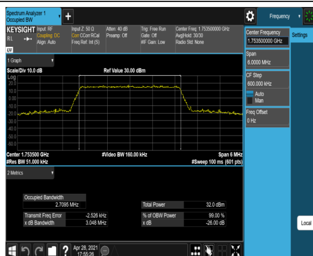
Band4-3MHz-16QAM-20385-15RB#0
