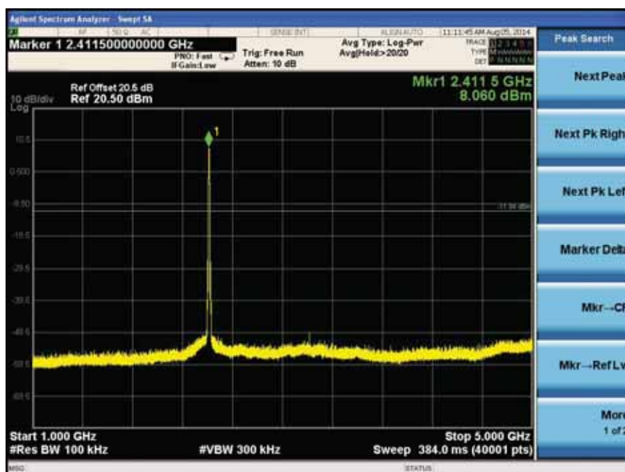
Channel 01 (2412MHz)-2
