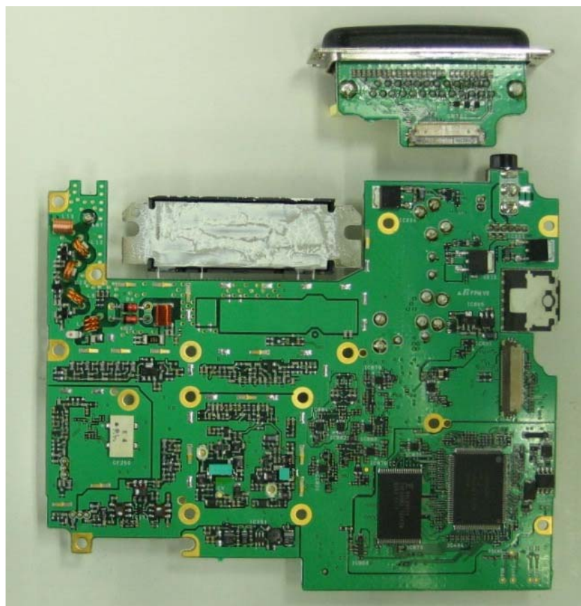
TXRX Foil Side View
