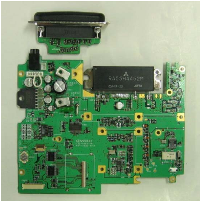
TXRX Component Side View
