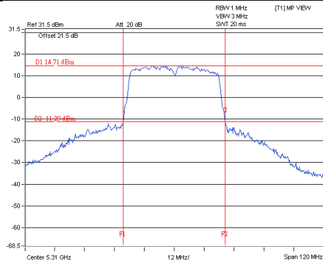
802.11ac (VHT40)_Chain 1 / CH62
