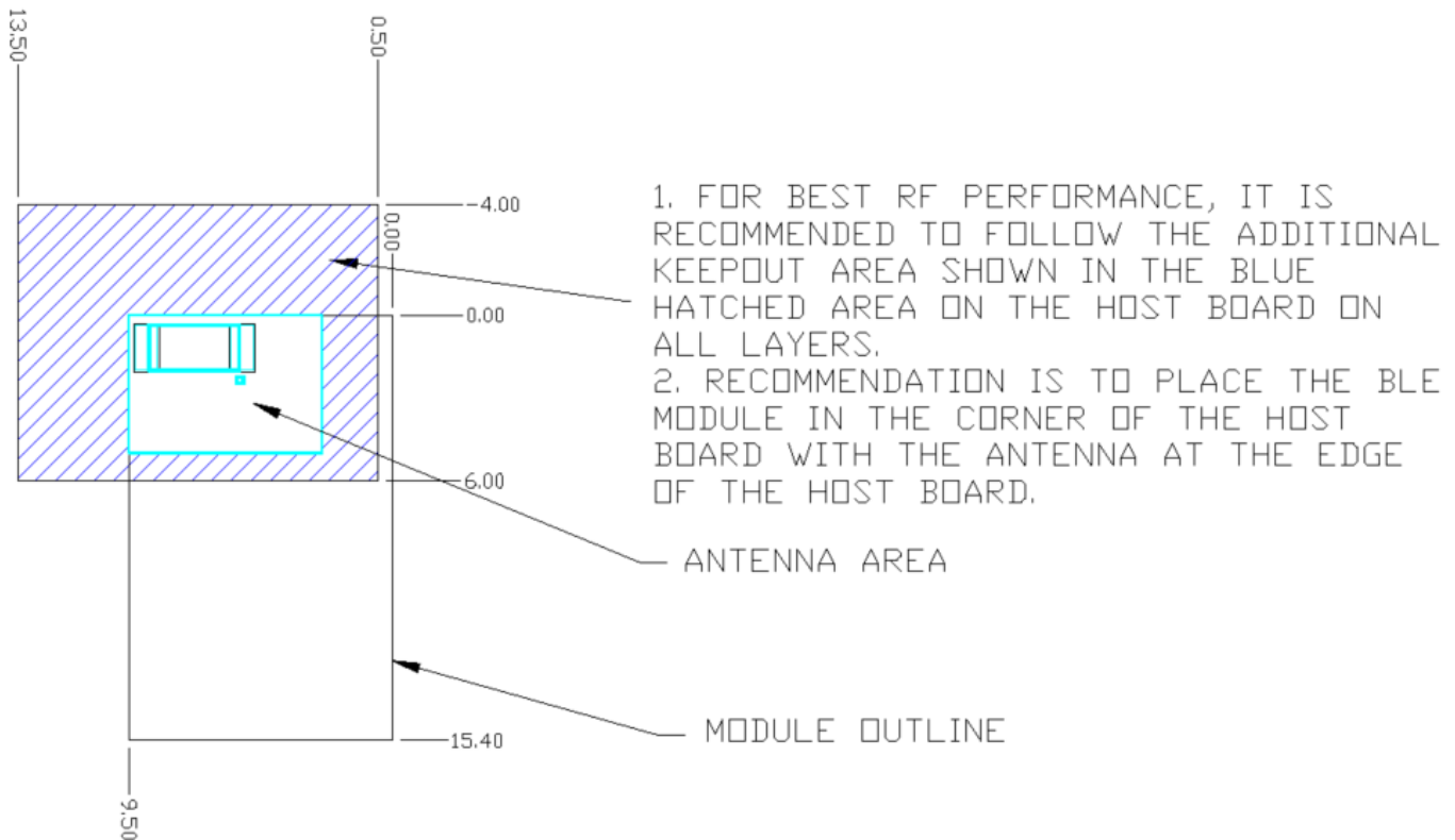
Figure 3. Recommended Host PCB Keep-Out Area around CYBLE-224110-00 Trace Antenna
