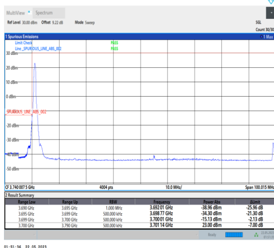
1-N77-3700-3980-PC1-30-90-L-4-CP-QPSK-Edge_1 RB_Left-1@0-Ant0-1--PASS-see graph
