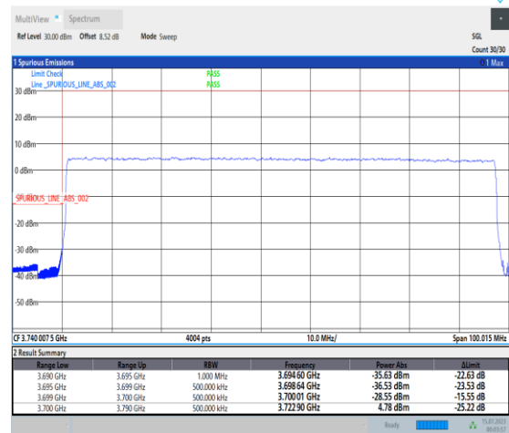
1-N77-3700-3980-PC1-30-90-L-3-DFT-PI2BPSK-O uter_Full-240@0-Ant0-1--PASS-see graph
